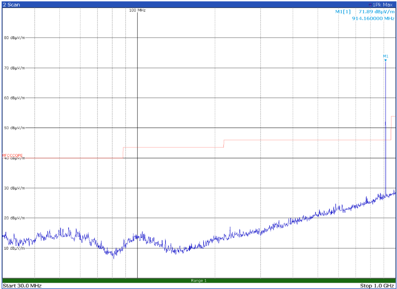
Figure 8.9-21: Radiated spurious emissions on high channel - LoRa 500 kHz BW – Antenna in horizontal polarization
