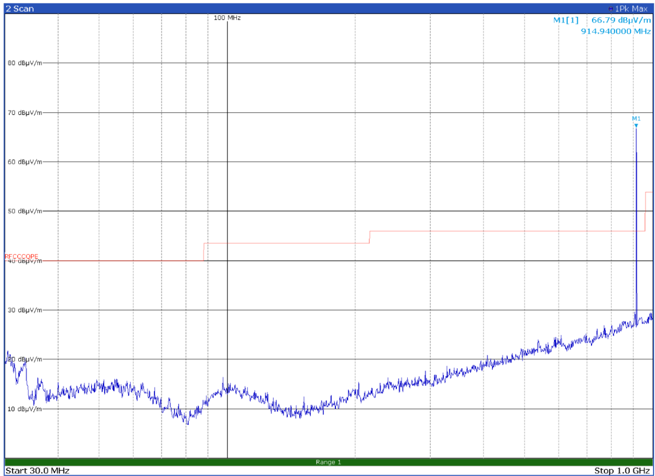
Figure 8.9-10: Radiated spurious emissions on high channel - LoRa 125 kHz BW – Antenna in vertical polarization
