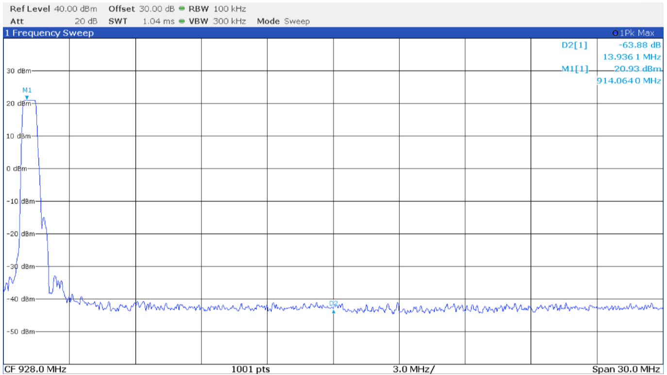
Figure 8.9-49: Band edge spurious emissions at 928 MHz - LoRa 500 kHz BW
