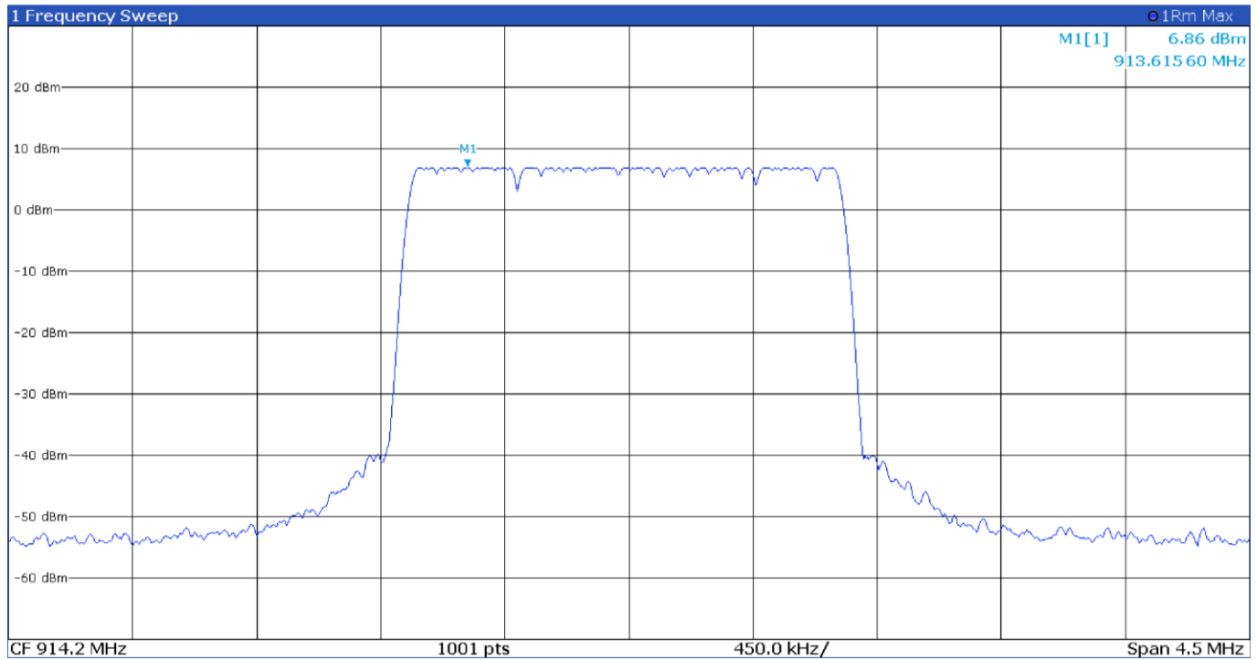
Figure 8.10-6: PSD on high channel – LR-FHSS
