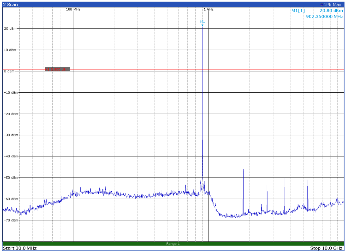
Figure 8.9-37: Conducted spurious emissions on low channel - LoRa 125 kHz BW
