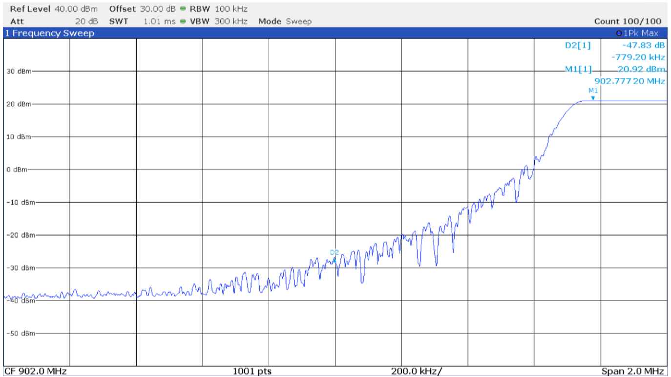
Figure 8.9-48: Band edge spurious emissions at 902 MHz - LoRa 500 kHz BW
