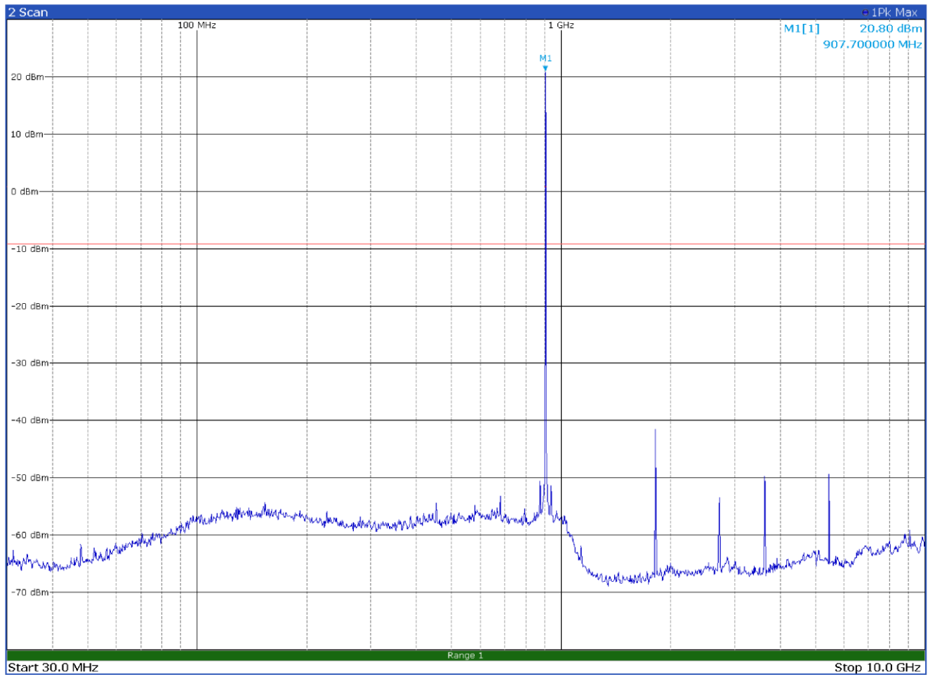
Figure 8.9-41: Conducted spurious emissions on mid channel - LoRa 500 kHz BW
