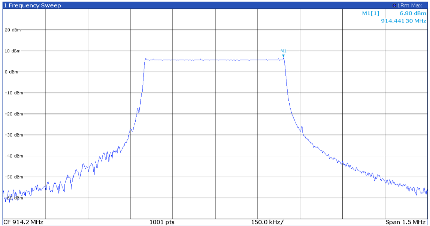
Figure 8.10-3: PSD on high channel - LoRa 500 kHz BW
