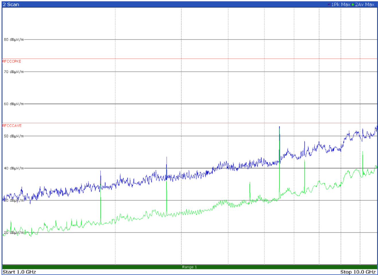
Figure 8.9-24: Radiated spurious emissions on high channel - LoRa 500 kHz BW – Antenna in vertical polarization
