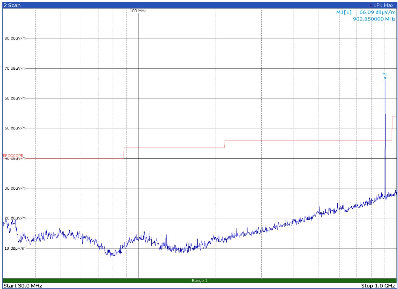
Figure 8.9-14: Radiated spurious emissions on low channel - LoRa 500 kHz BW – Antenna in vertical polarization
