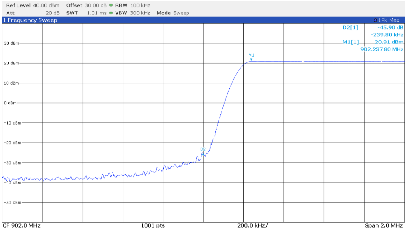
Figure 8.9-50: Band edge spurious emissions at 902 MHz – LR-FHSS
