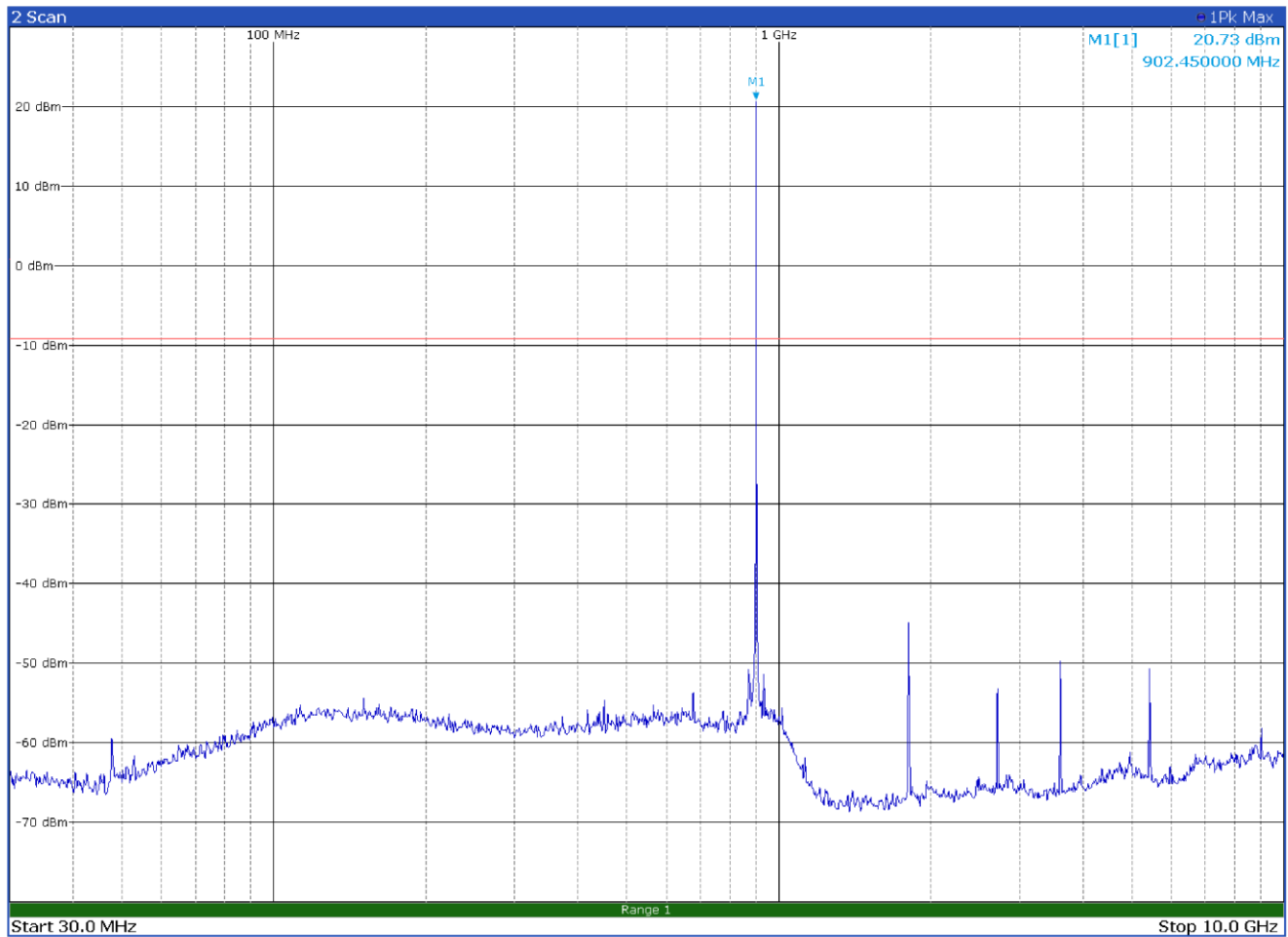
Figure 8.9-43: Conducted spurious emissions on low channel – LR-FHSS
