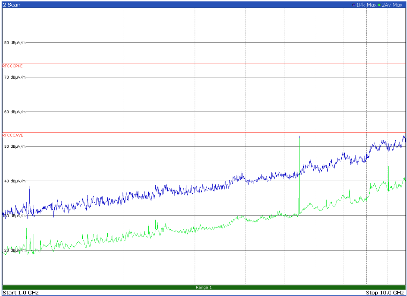
Figure 8.9-19: Radiated spurious emissions on mid channel - LoRa 500 kHz BW – Antenna in horizontal polarization
