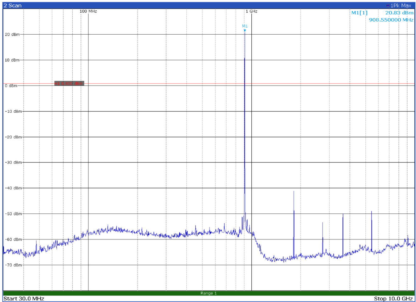
Figure 8.9-38: Conducted spurious emissions on mid channel - LoRa 125 kHz BW
