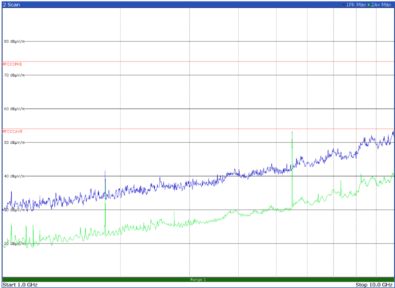
Figure 8.9-23: Radiated spurious emissions on high channel - LoRa 500 kHz BW – Antenna in horizontal polarization
