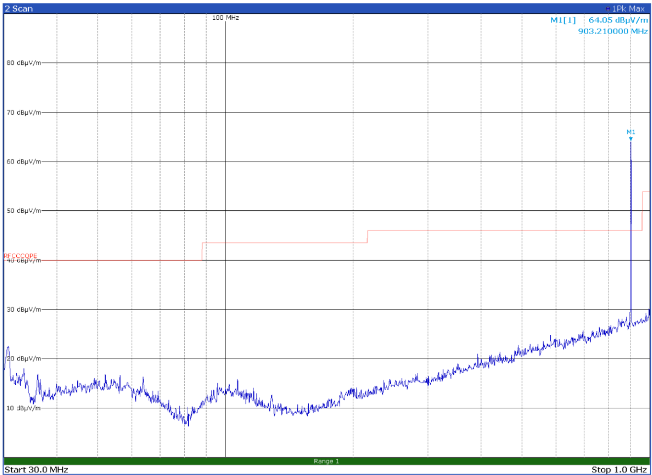
Figure 8.9-26: Radiated spurious emissions on low channel - LR-FHSS – Antenna in vertical polarization
