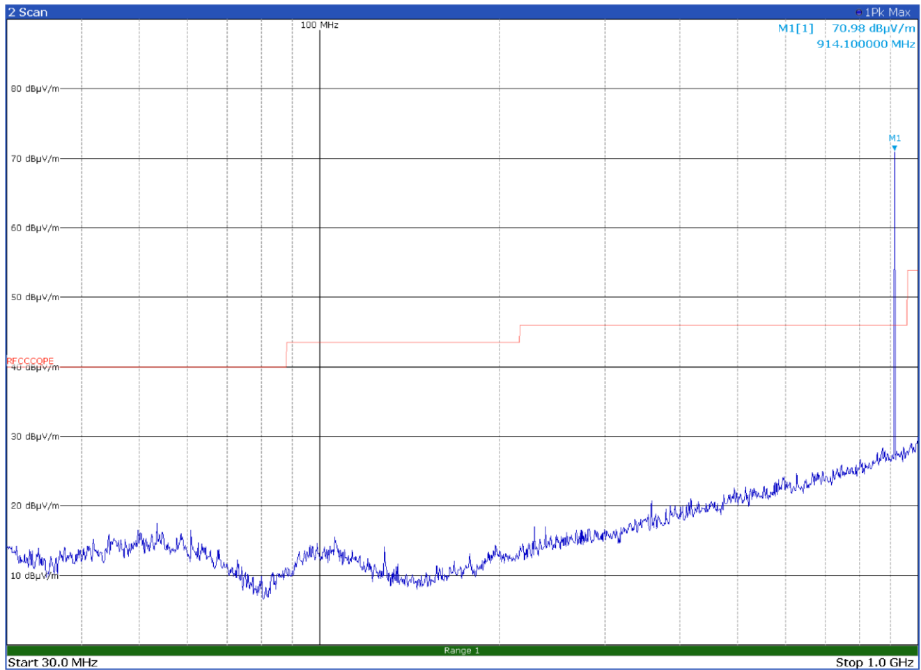
Figure 8.9-33: Radiated spurious emissions on high channel - LR-FHSS – Antenna in horizontal polarization
