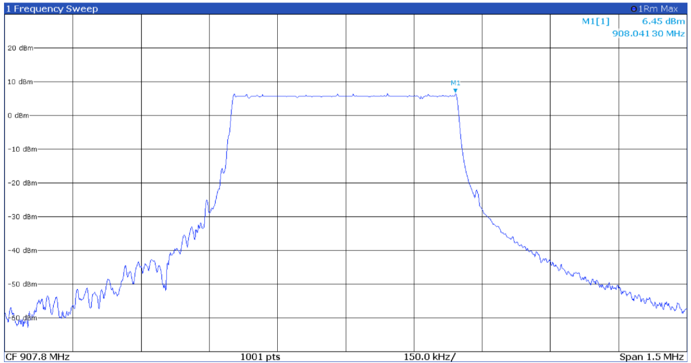
Figure 8.10-2: PSD on mid channel - LoRa 500 kHz BW
