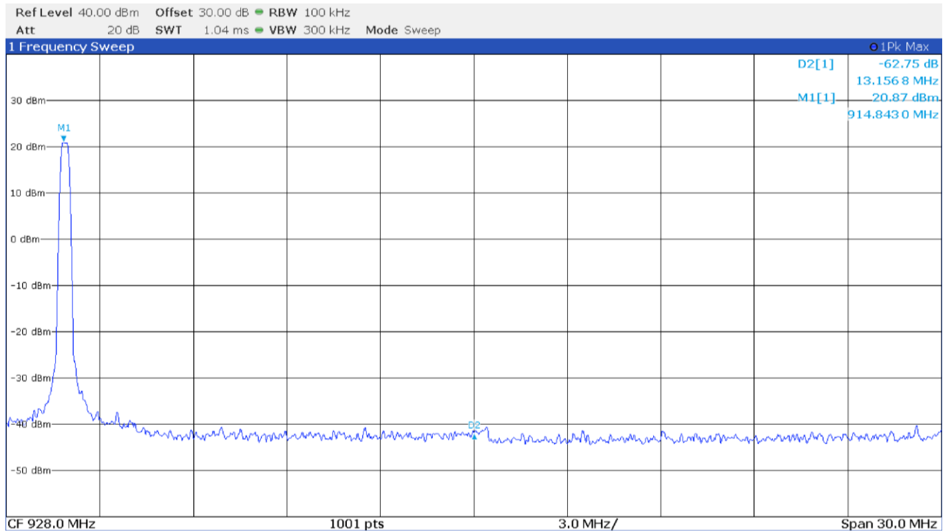
Figure 8.9-47: Band edge spurious emissions at 928 MHz - LoRa 125 kHz BW
