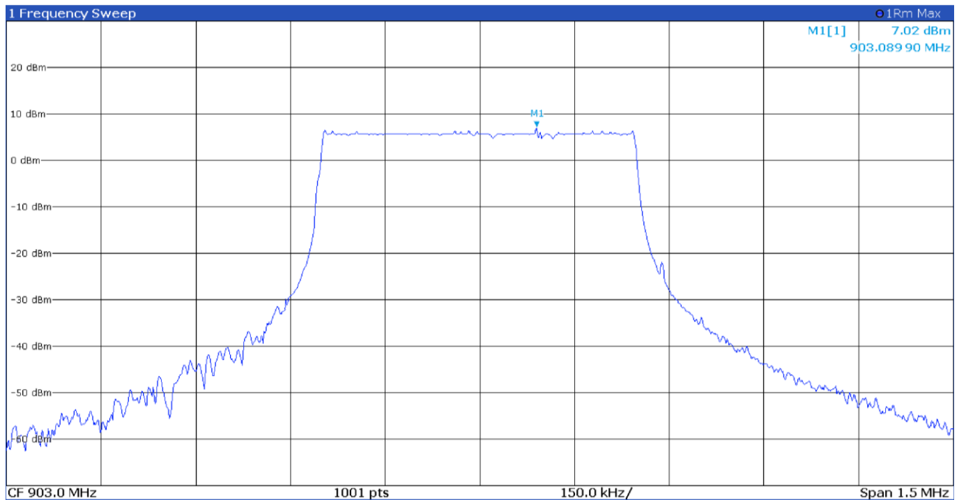
Figure 8.10-1: PSD on low channel - LoRa 500 kHz BW
