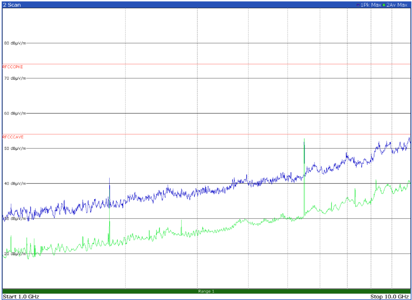
Figure 8.9-35: Radiated spurious emissions on high channel - LR-FHSS – Antenna in horizontal polarization
