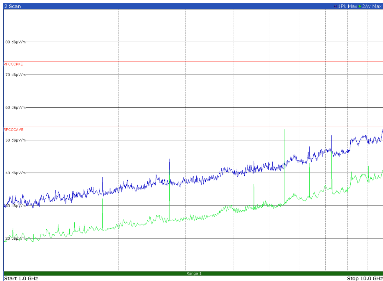
Figure 8.9-32: Radiated spurious emissions on mid channel - LR-FHSS – Antenna in vertical polarization
