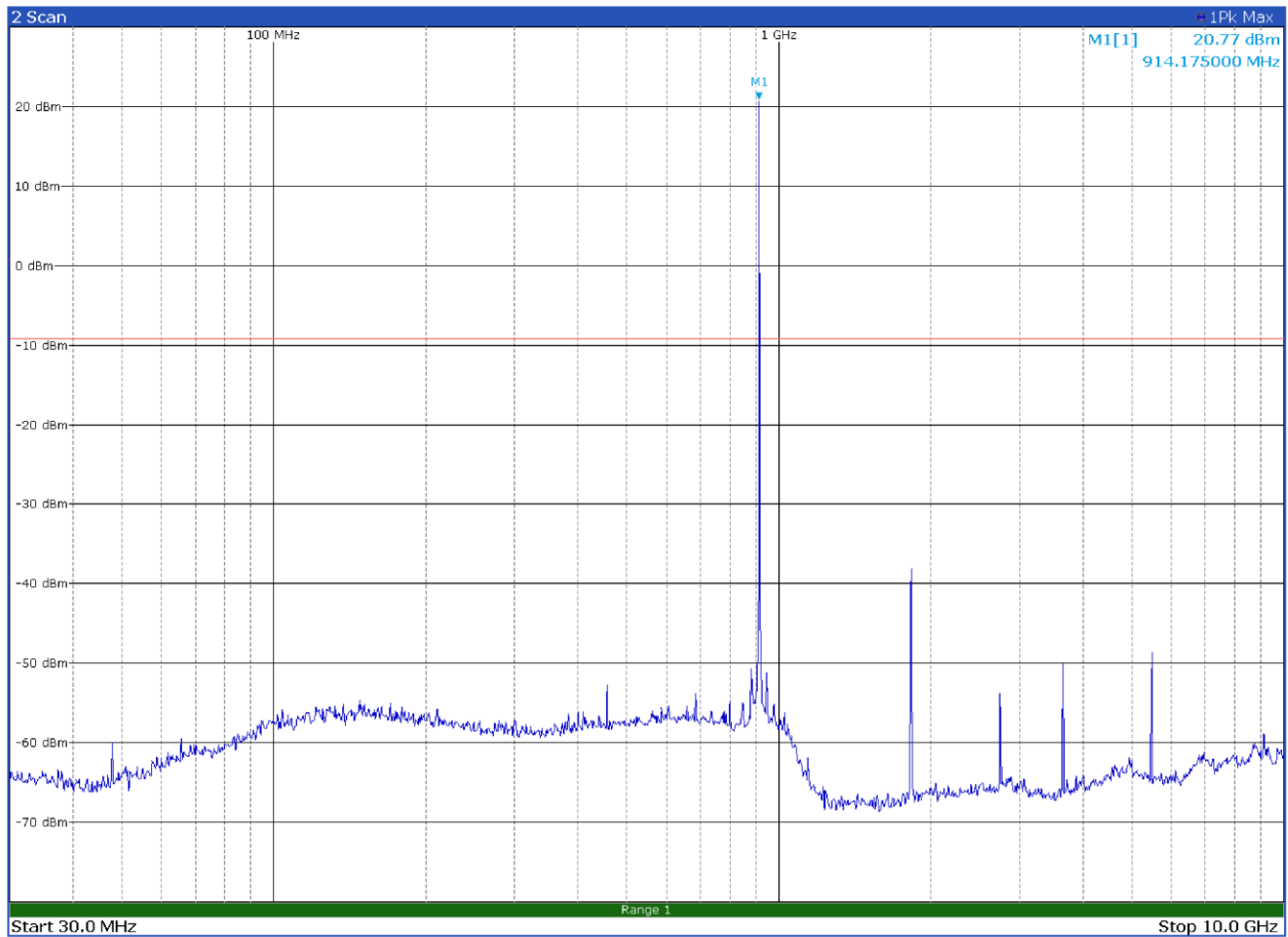
Figure 8.9-42: Conducted spurious emissions on high channel - LoRa 500 kHz BW
