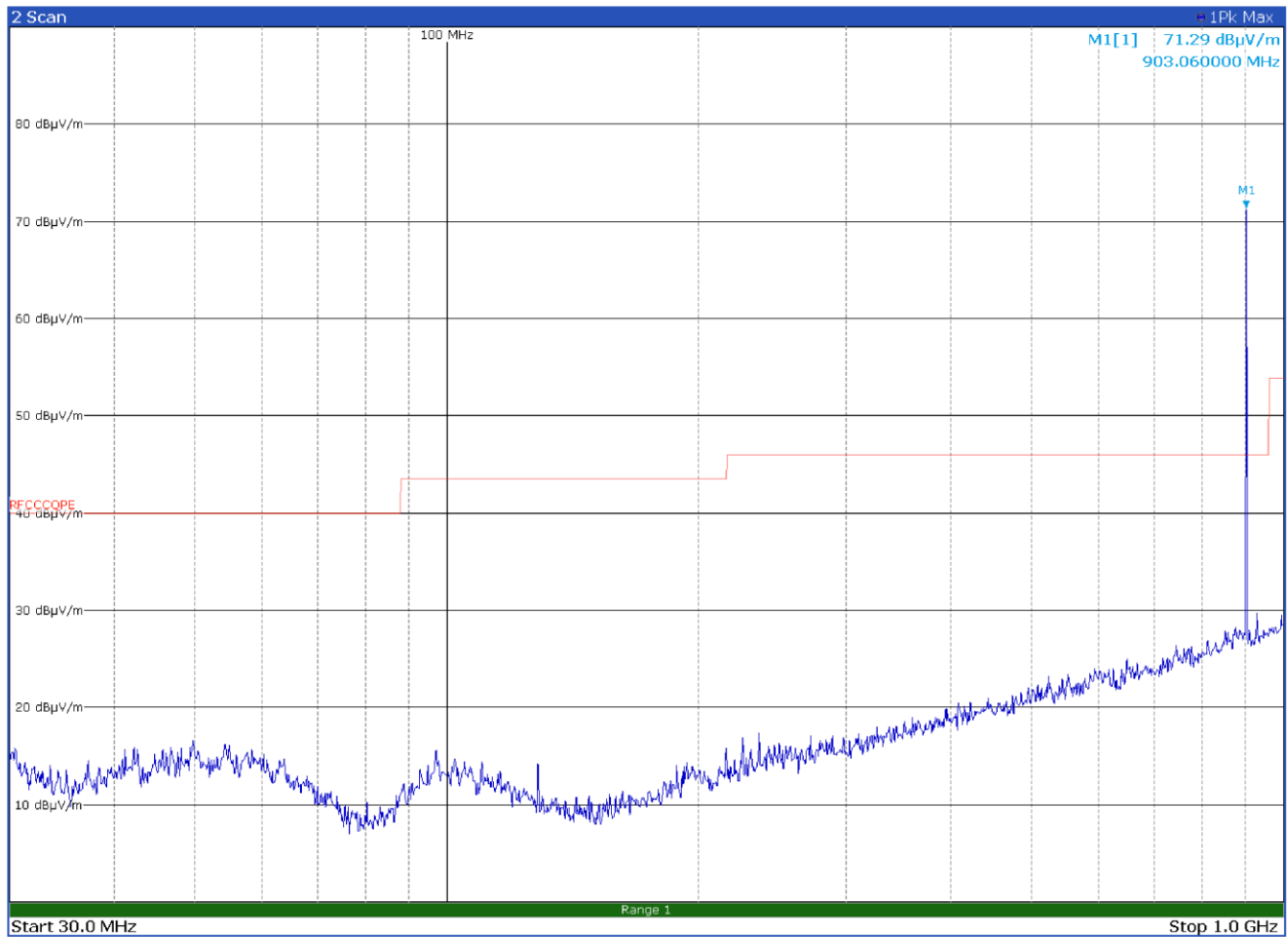
Figure 8.9-25: Radiated spurious emissions on low channel - LR-FHSS – Antenna in horizontal polarization
