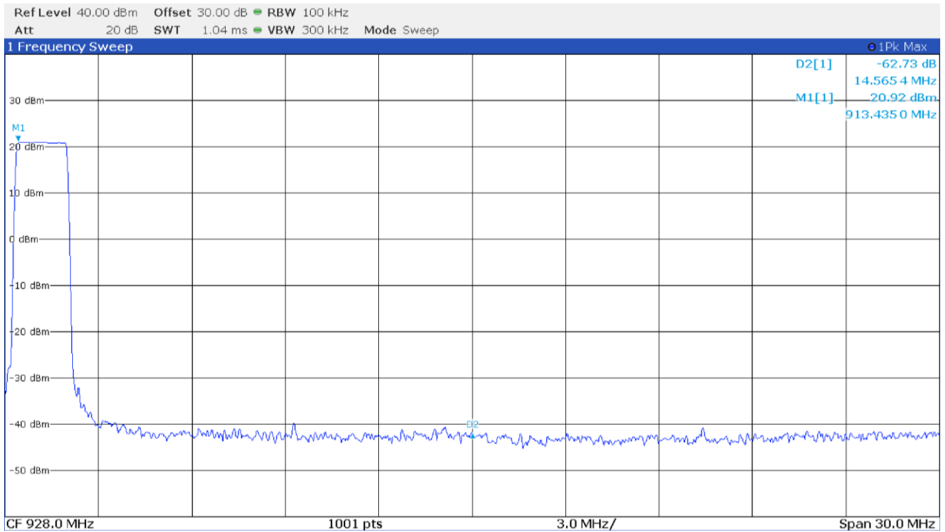
Figure 8.9-51: Band edge spurious emissions at 928 MHz – LR-FHSS
