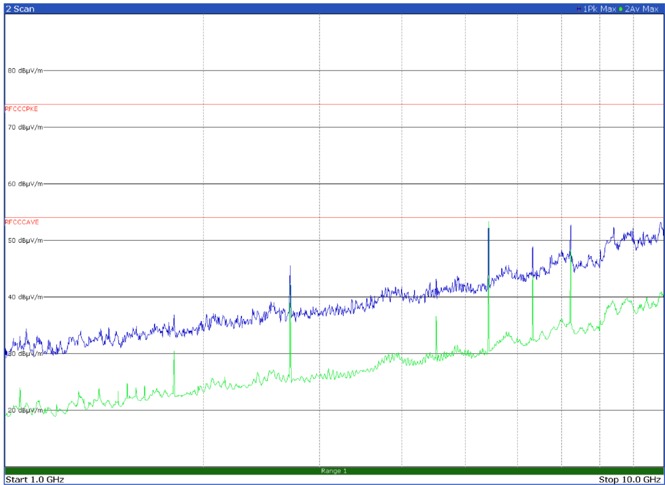
Figure 8.9-28: Radiated spurious emissions on low channel - LR-FHSS – Antenna in vertical polarization
