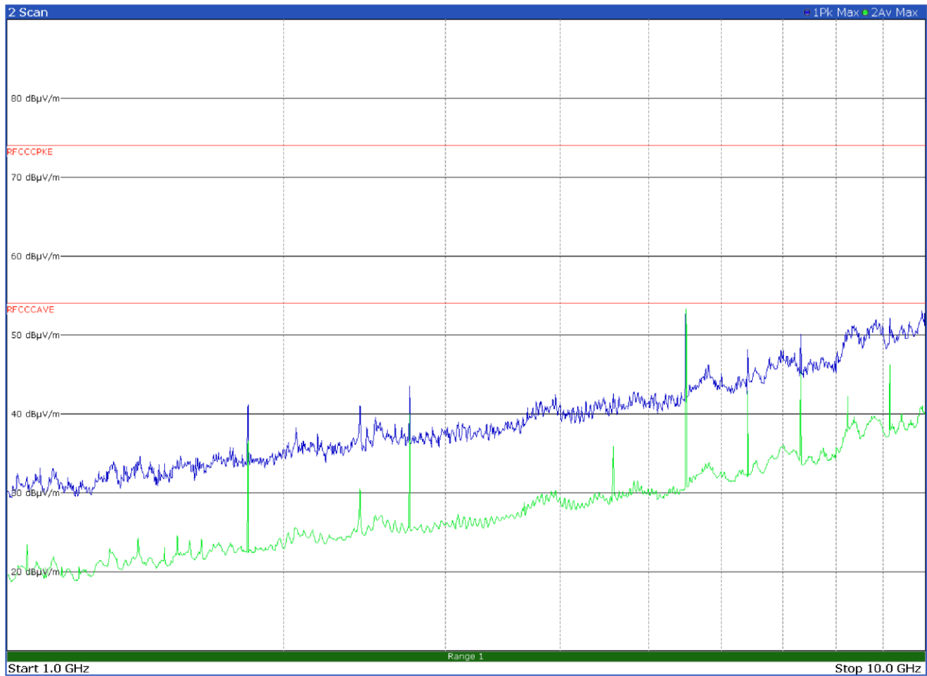
Figure 8.9-12: Radiated spurious emissions on high channel - LoRa 125 kHz BW – Antenna in vertical polarization
