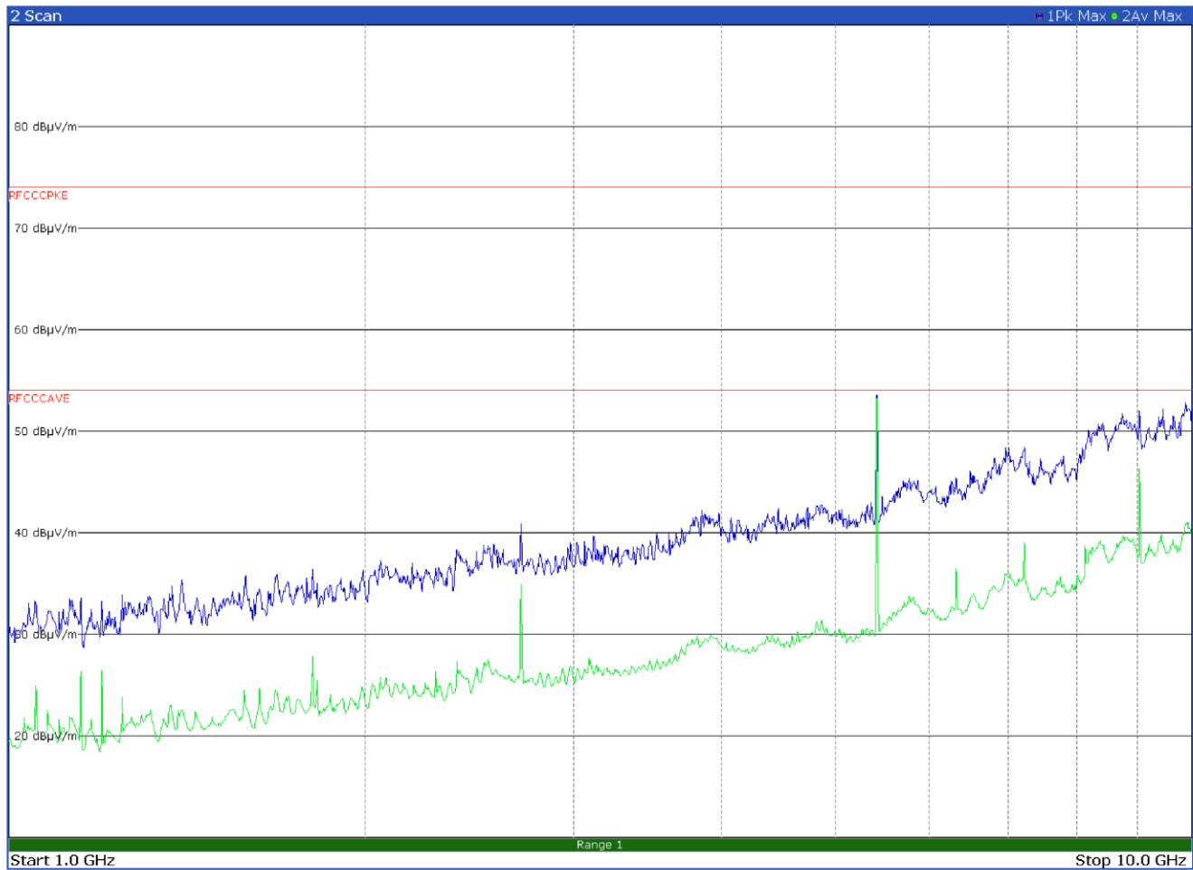
Figure 8.9-15: Radiated spurious emissions on low channel - LoRa 500 kHz BW – Antenna in horizontal polarization
