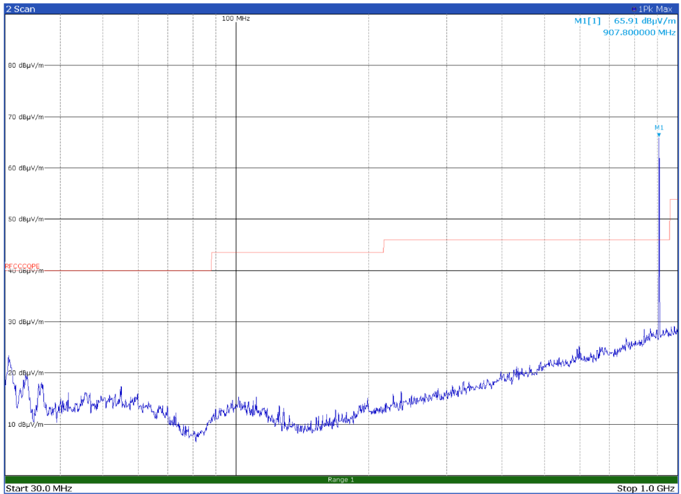
Figure 8.9-18: Radiated spurious emissions on mid channel - LoRa 500 kHz BW – Antenna in vertical polarization
