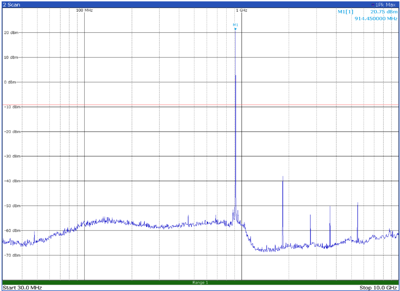
Figure 8.9-45: Conducted spurious emissions on high channel - LR-FHSS
