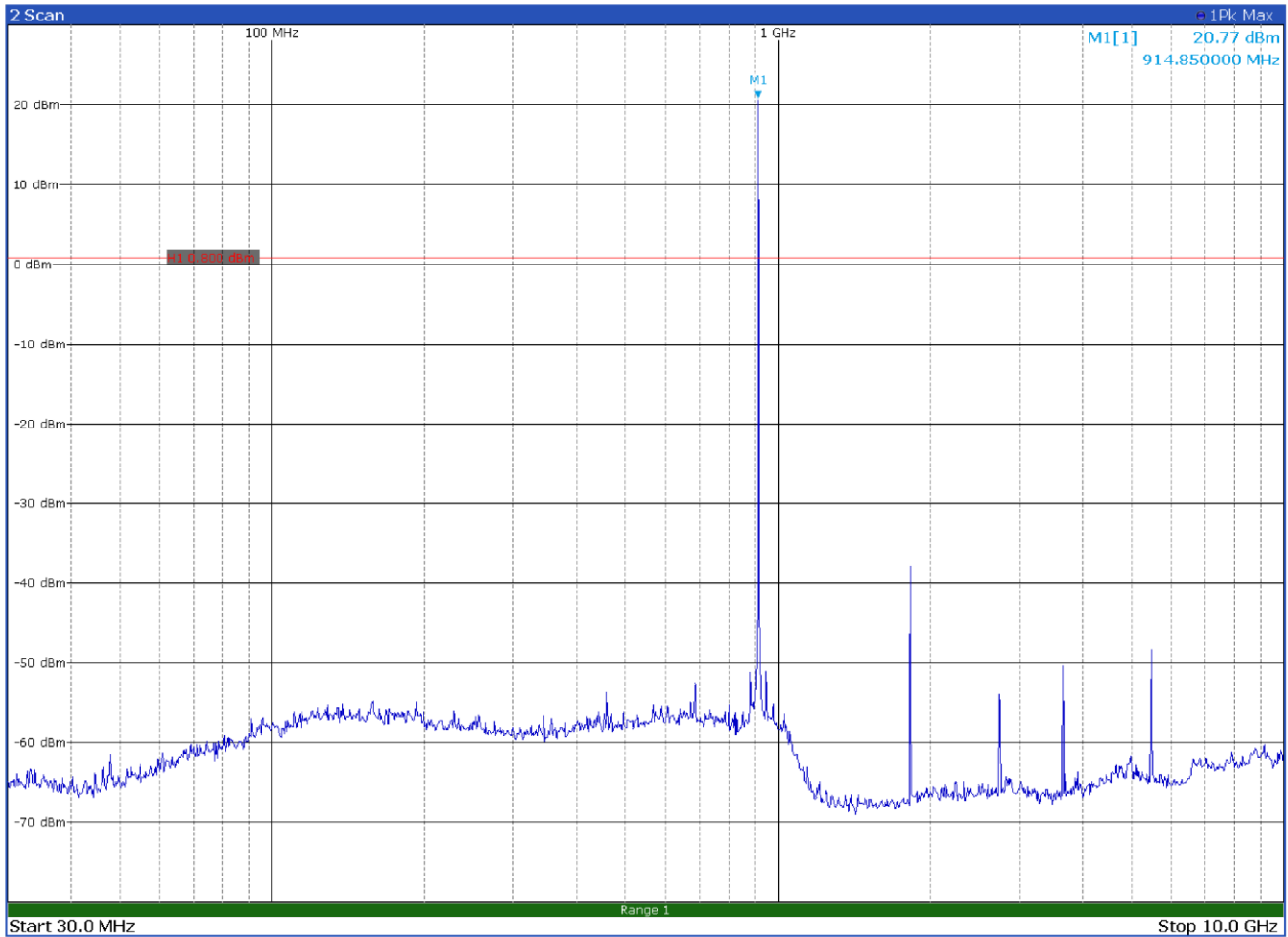
Figure 8.9-39: Conducted spurious emissions on high channel - LoRa 125 kHz BW
