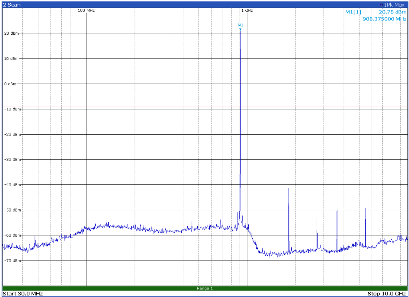
Figure 8.9-44: Conducted spurious emissions on mid channel - LR-FHSS
