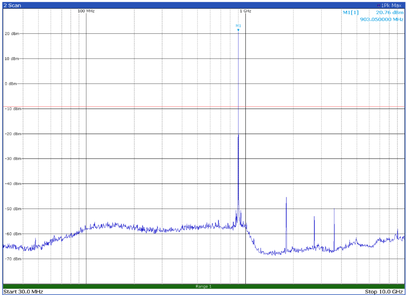
Figure 8.9-40: Conducted spurious emissions on low channel - LoRa 500 kHz BW
