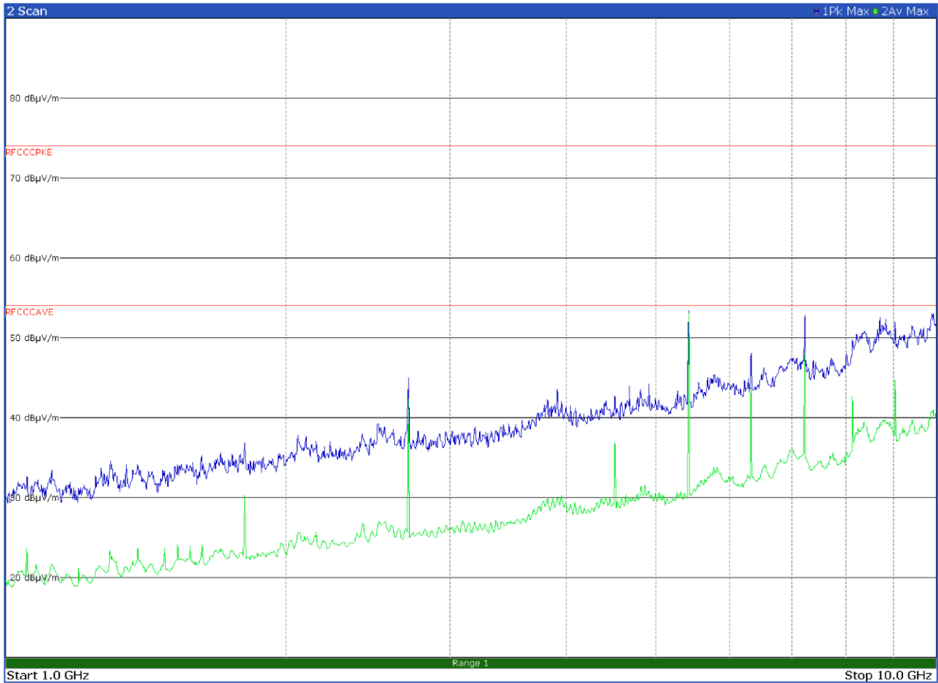
Figure 8.9-16: Radiated spurious emissions on low channel - LoRa 500 kHz BW – Antenna in vertical polarization
