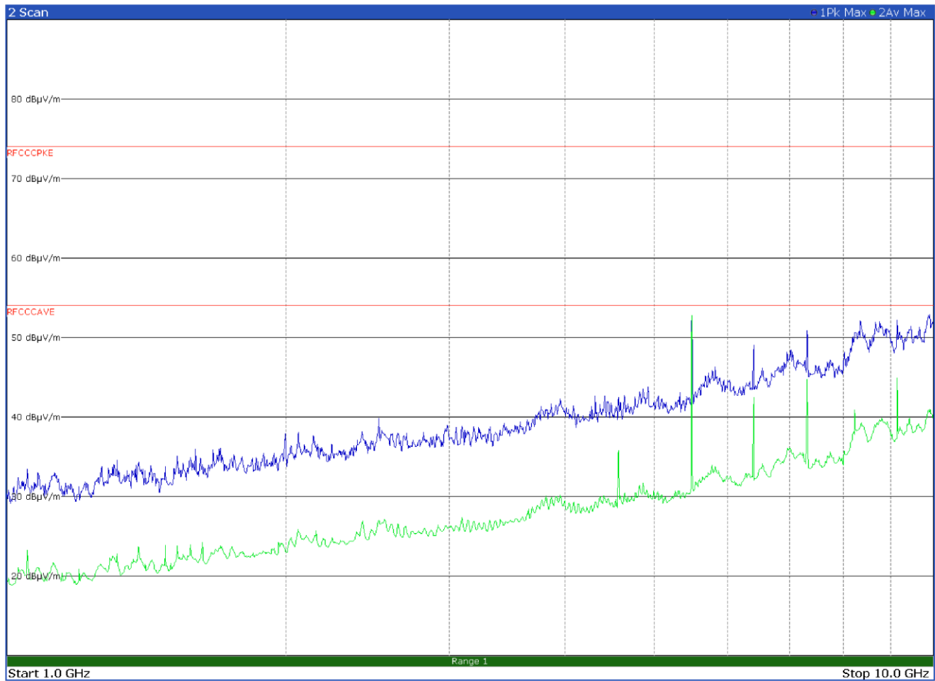
Figure 8.9-36: Radiated spurious emissions on high channel - LR-FHSS – Antenna in vertical polarization
