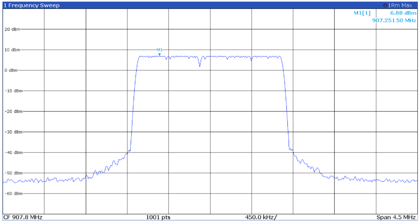
Figure 8.10-5: PSD on mid channel – LR-FHSS
