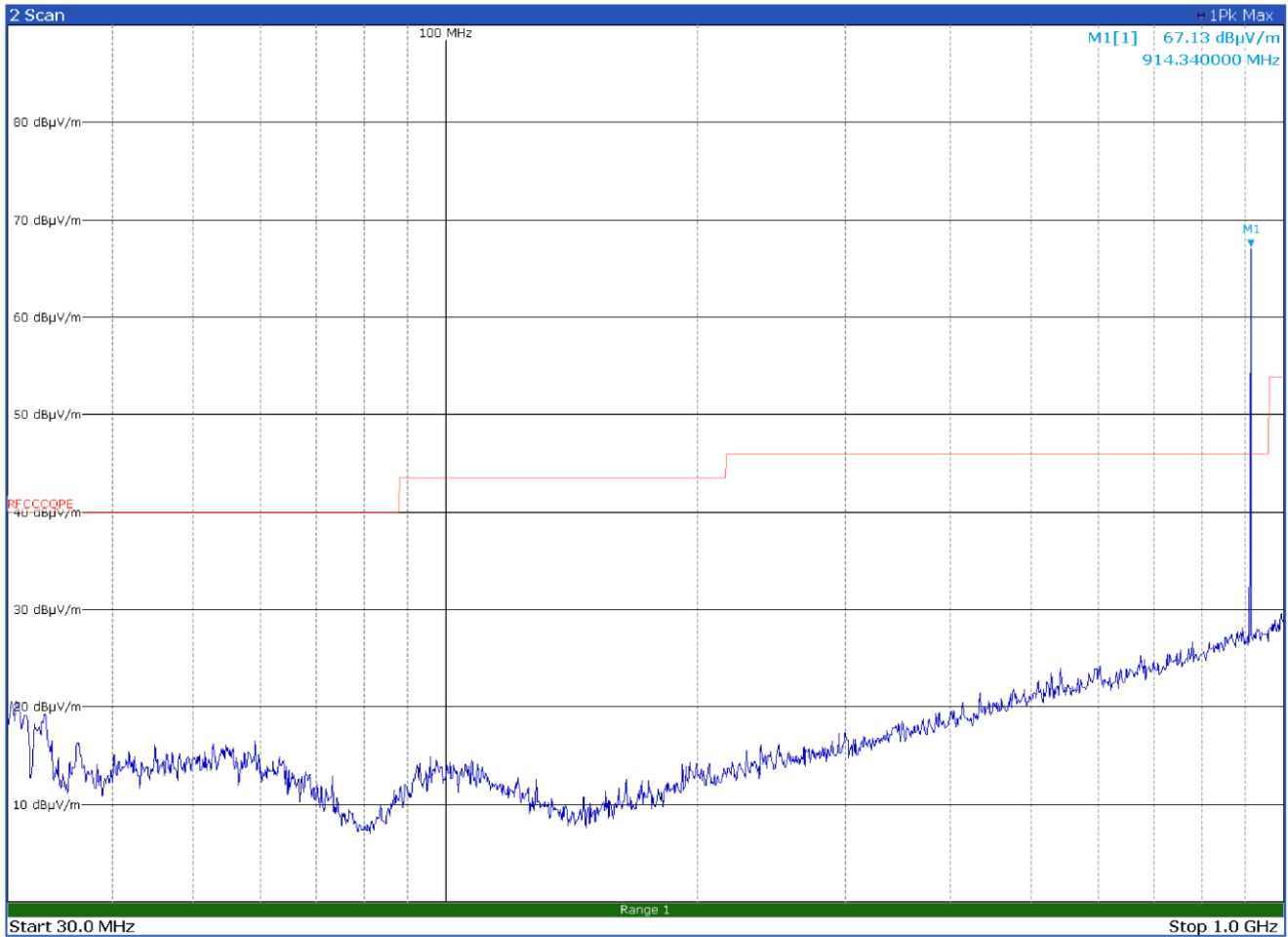
Figure 8.9-22: Radiated spurious emissions on high channel - LoRa 500 kHz BW – Antenna in vertical polarization
