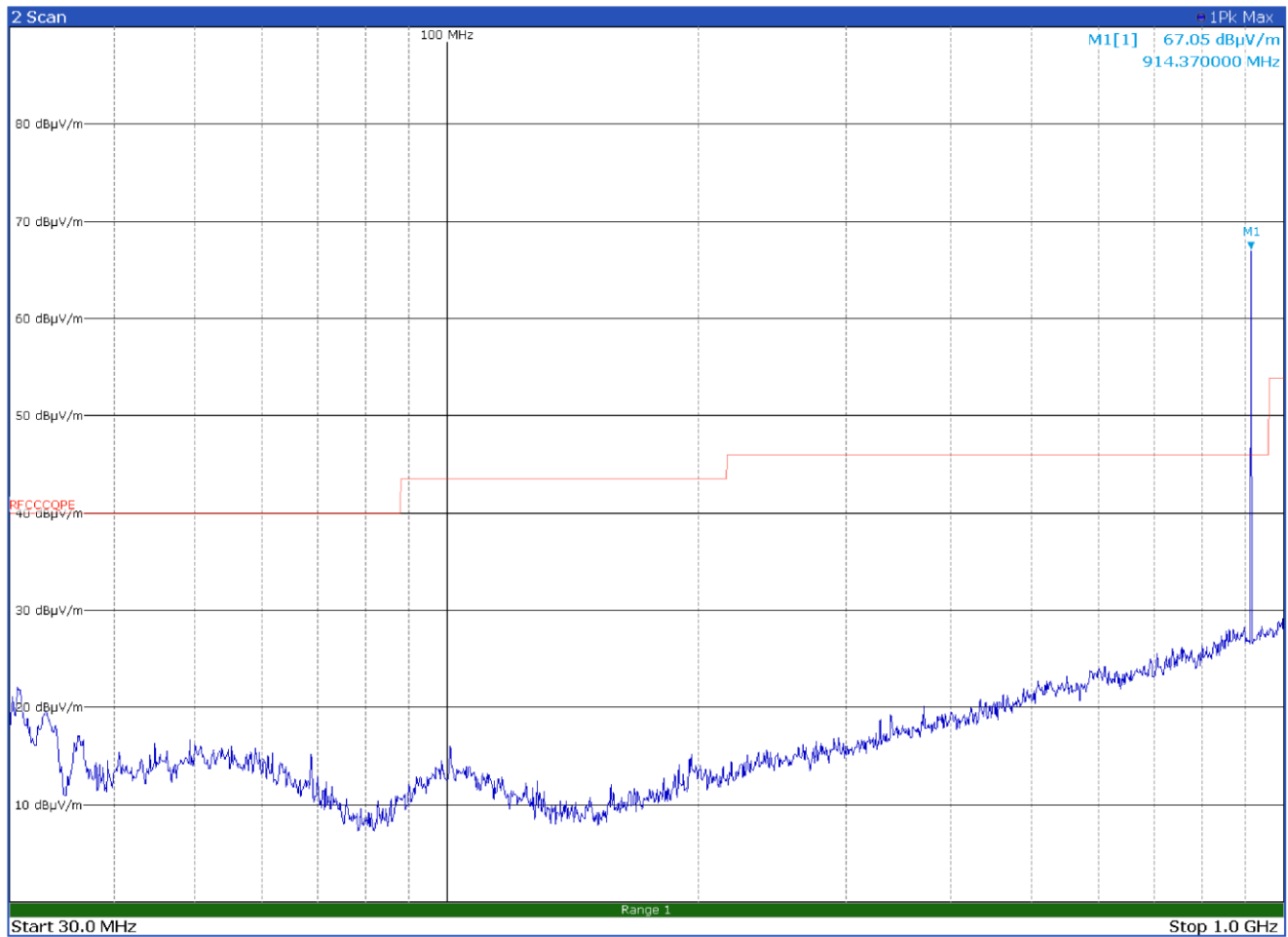
Figure 8.9-34: Radiated spurious emissions on high channel - LR-FHSS – Antenna in vertical polarization
