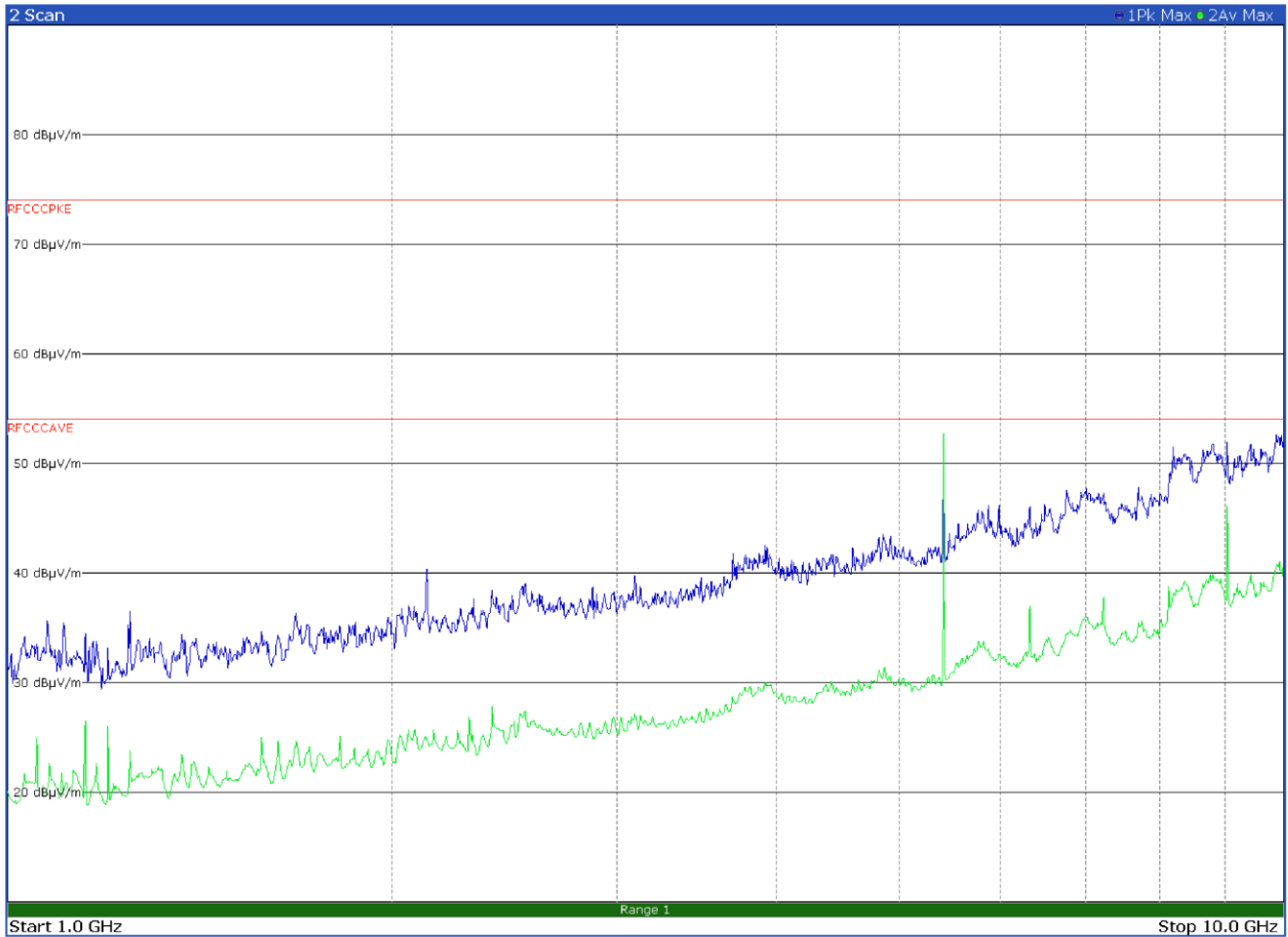
Figure 8.9-27: Radiated spurious emissions on low channel - LR-FHSS – Antenna in horizontal polarization
