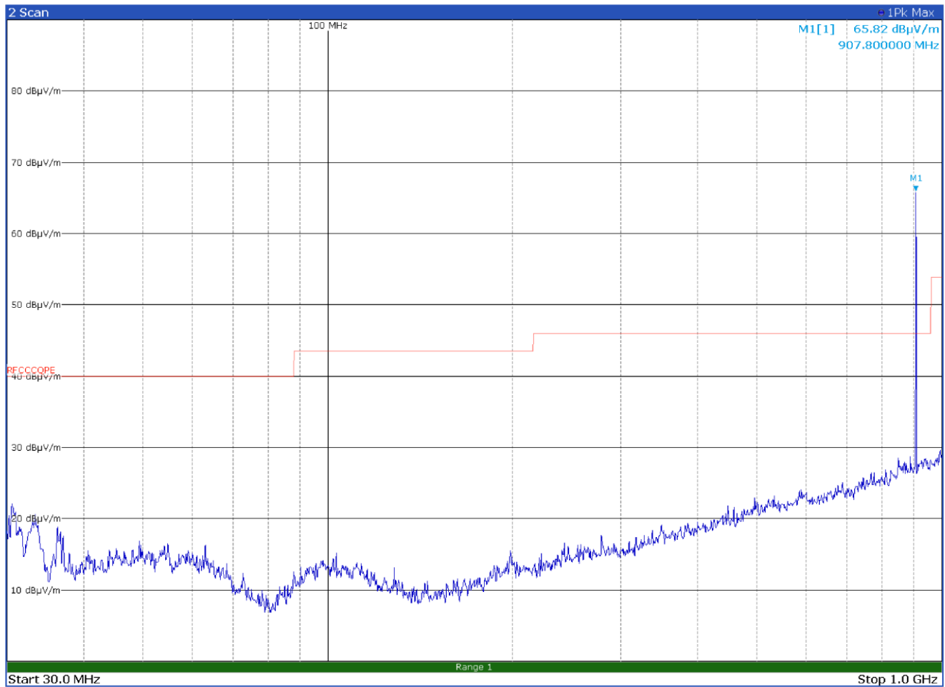
Figure 8.9-30: Radiated spurious emissions on mid channel - LR-FHSS – Antenna in vertical polarization
