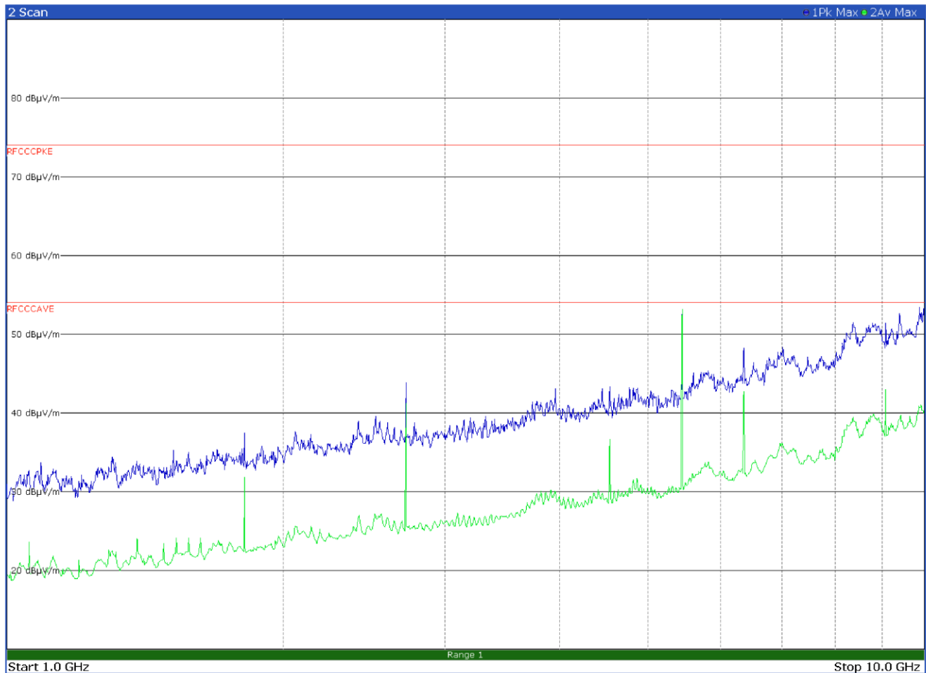
Figure 8.9-20: Radiated spurious emissions on mid channel - LoRa 500 kHz BW – Antenna in vertical polarization
