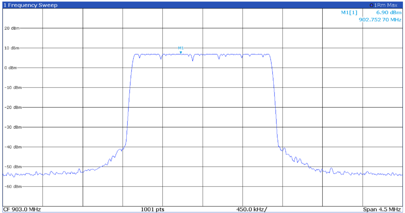
Figure 8.10-4: PSD on low channel – LR-FHSS
