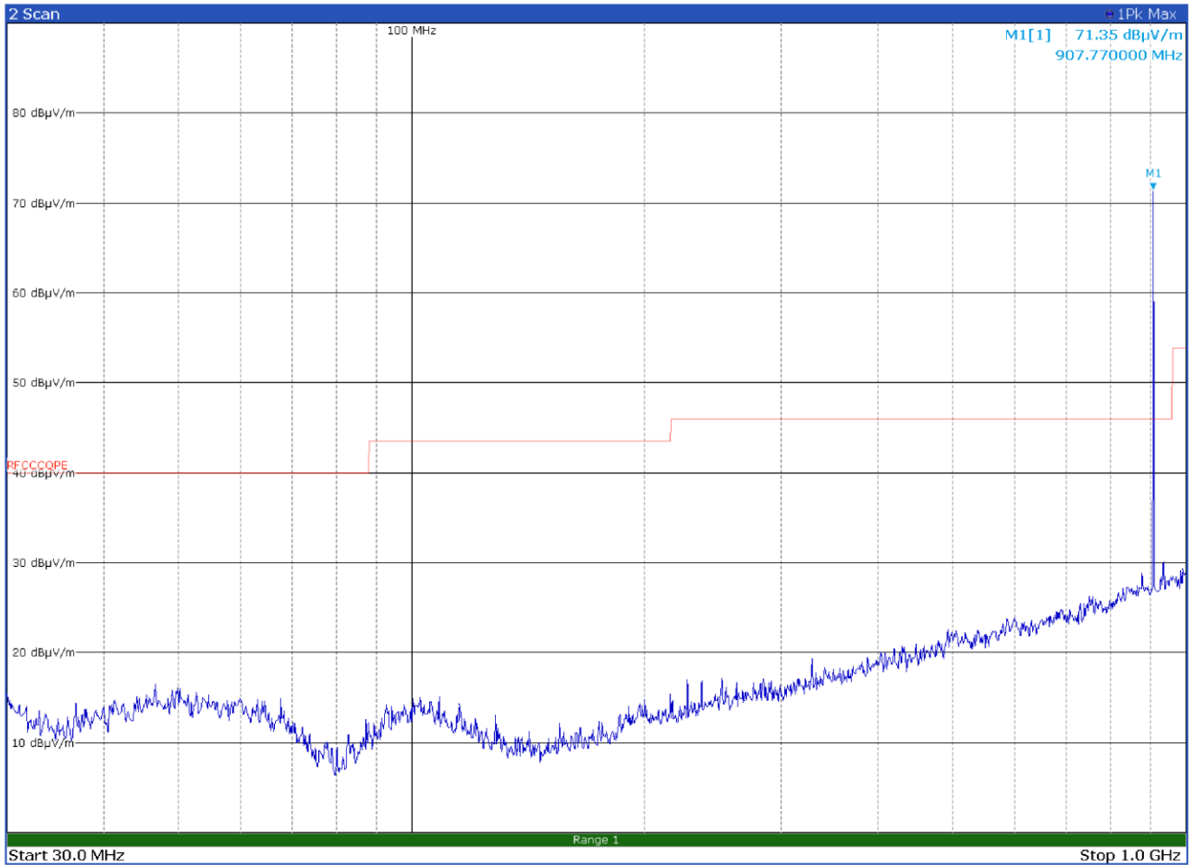
Figure 8.9-17: Radiated spurious emissions on mid channel - LoRa 500 kHz BW – Antenna in horizontal polarization
