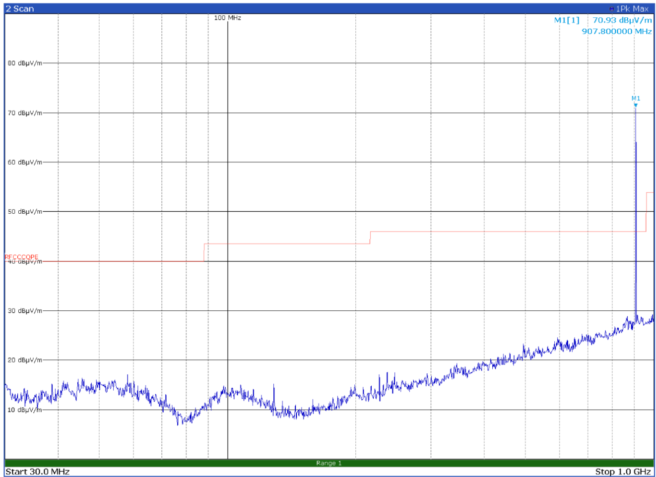
Figure 8.9-29: Radiated spurious emissions on mid channel - LR-FHSS – Antenna in horizontal polarization
