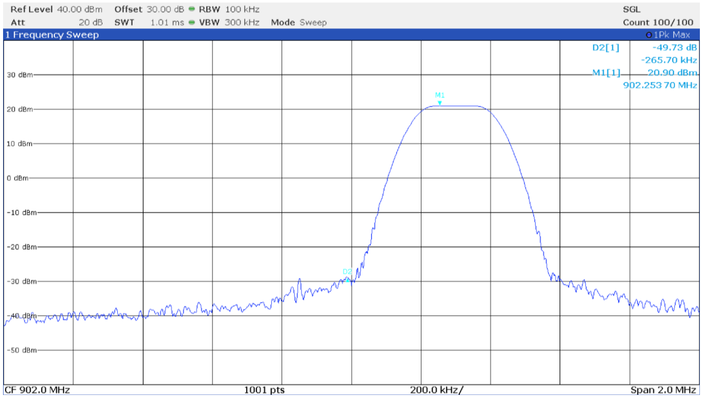
Figure 8.9-46: Band edge spurious emissions at 902 MHz - LoRa 125 kHz BW
