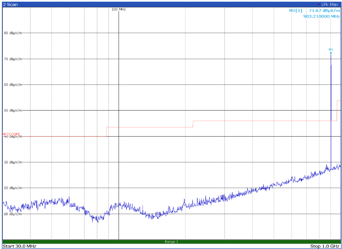
Figure 8.9-13: Radiated spurious emissions on low channel - LoRa 500 kHz BW – Antenna in horizontal polarization
