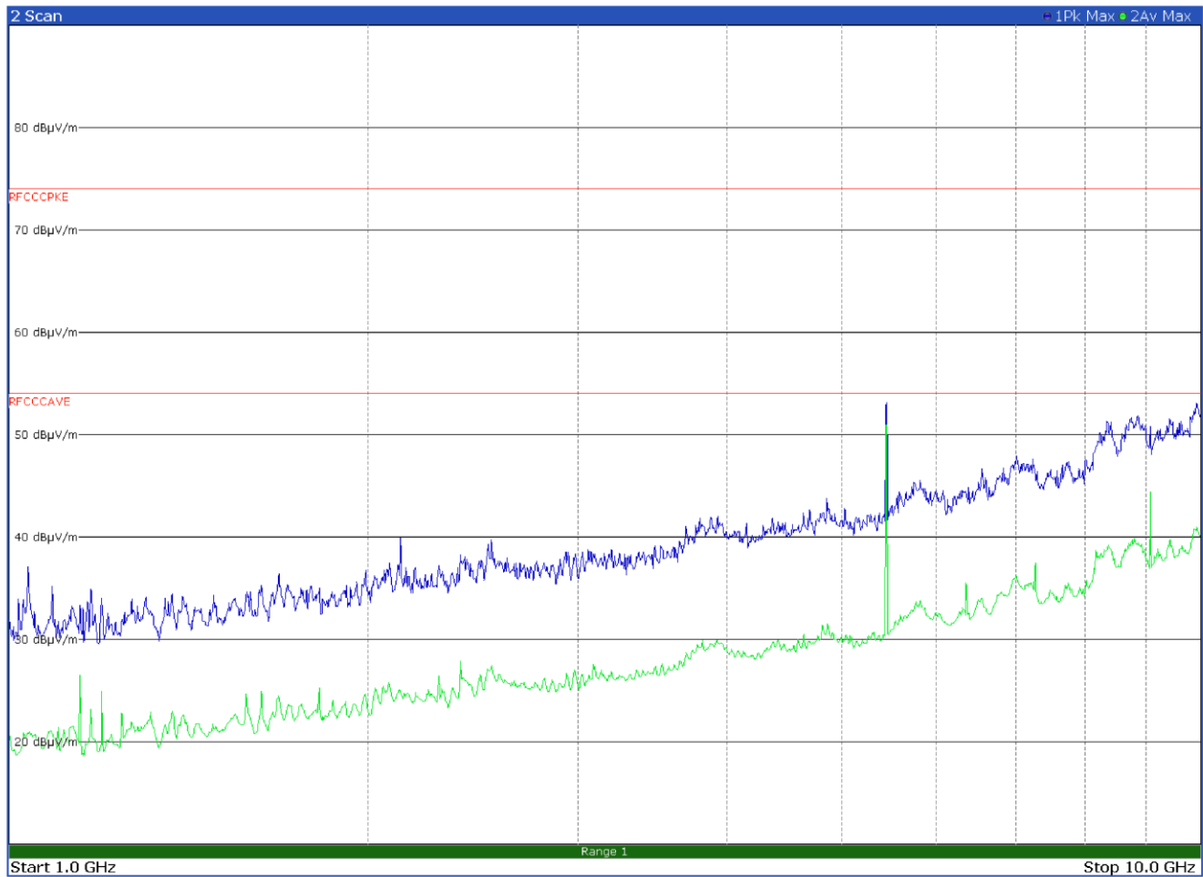
Figure 8.9-31: Radiated spurious emissions on mid channel - LR-FHSS – Antenna in horizontal polarization
