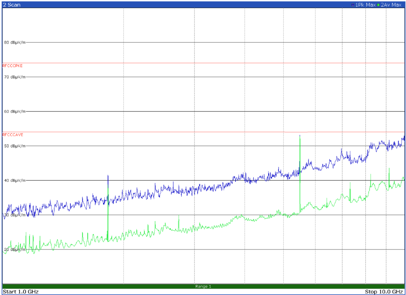
Figure 8.9-11: Radiated spurious emissions on high channel - LoRa 125 kHz BW – Antenna in horizontal polarization
