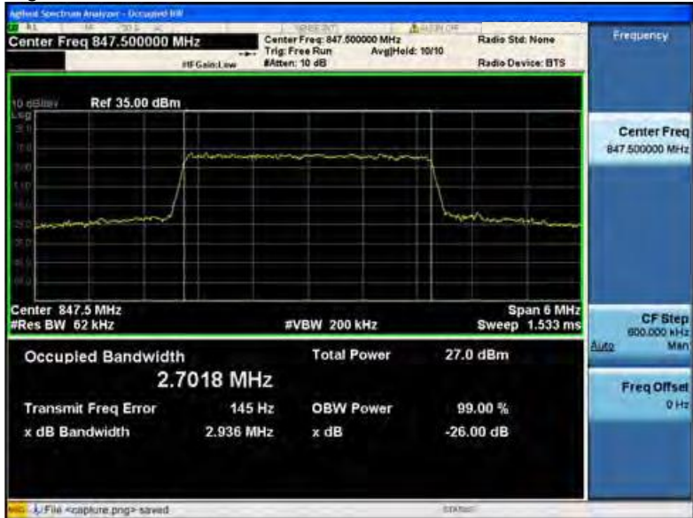
LTE Band 5 Highest channel:
