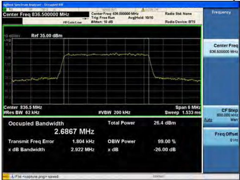
LTE Band 5 Middle channel
