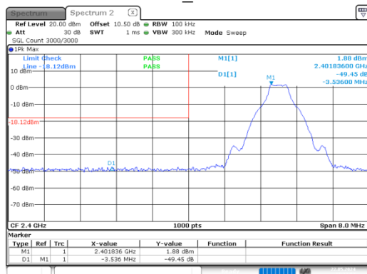
DH1_Low
