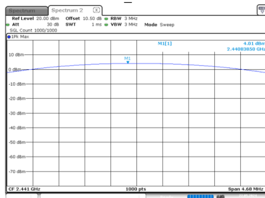
DH1_Middle
