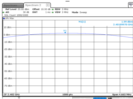
DH1_Low
