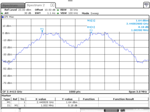
DH1_Middle
