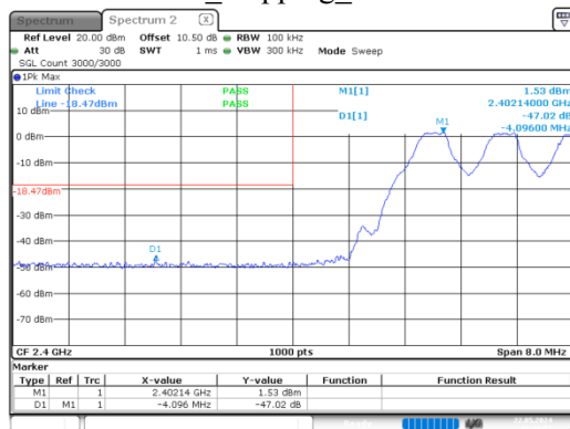
DH1_Hopping_Lower
