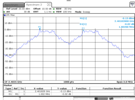
DH1_Low
