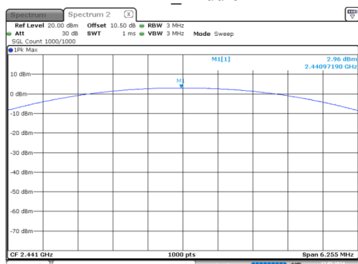
2DH1_Middle
