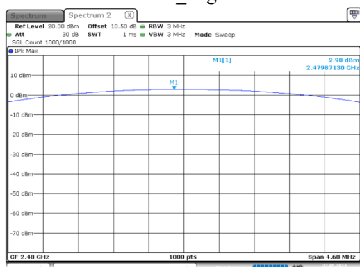
DH1_High
