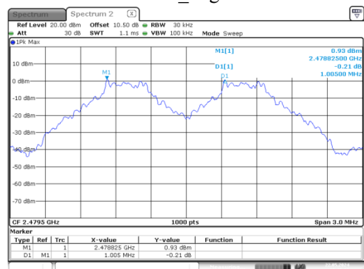
DH1_High
