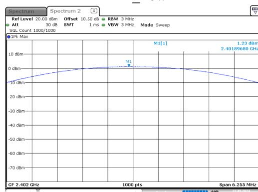
2DH1_Low
