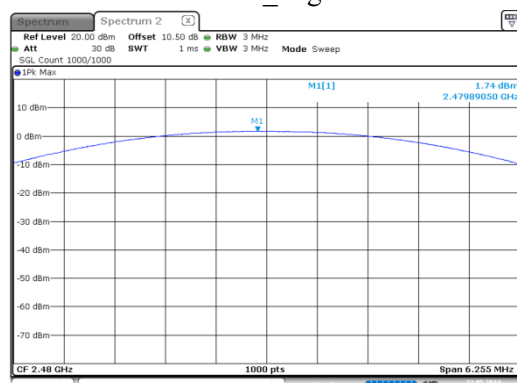
2DH1_High
