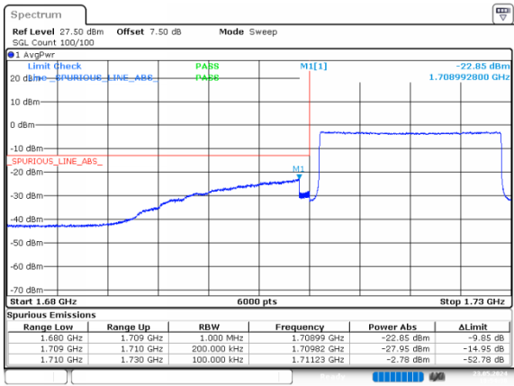
20MHz_Low_16QAM_100@0
