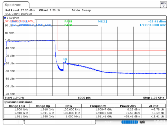
10MHz_High_16QAM_50@0
