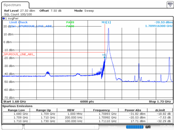
20MHz_Low_16QAM_1@0
