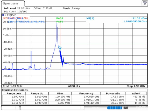
20MHz_High_16QAM_1@99
