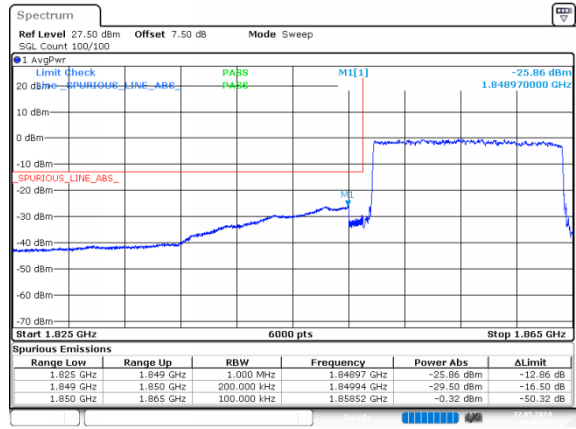
15MHz_Low_QPSK_75@0
