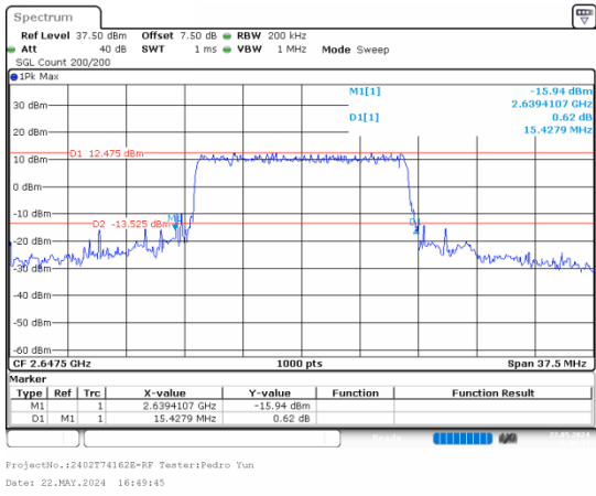
26dB Bandwidth
