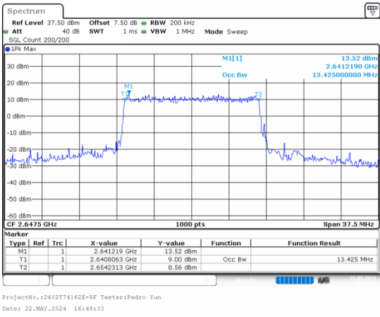
Occupied Bandwidth
