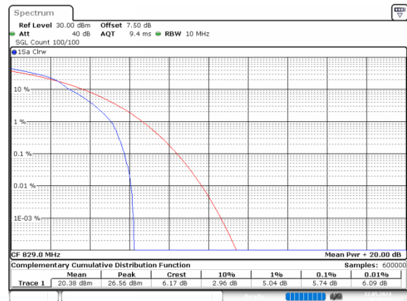
10MHz_Low_16QAM_1@0
