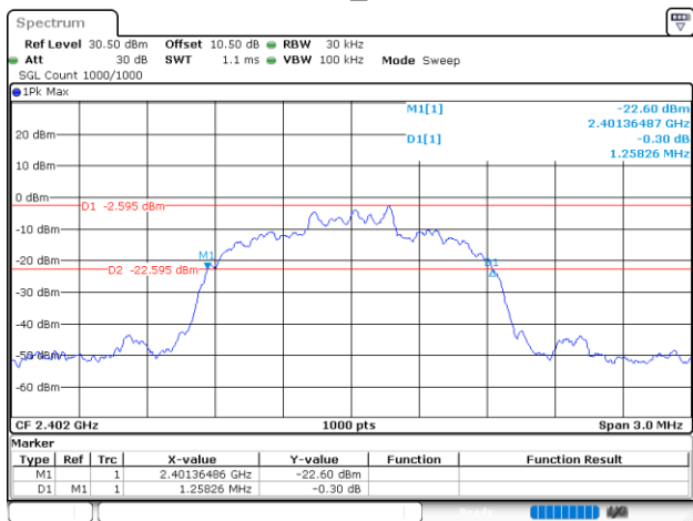
3DH5_Low
