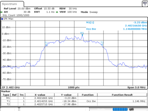
2DH5_Low
