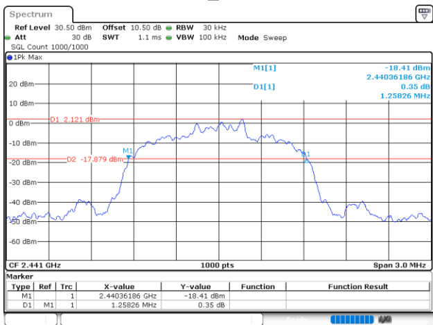
3DH5_Middle
