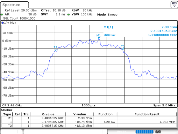
2DH5_High
