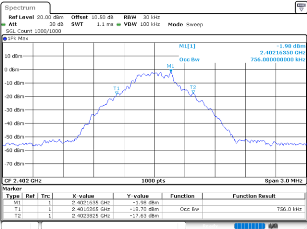
DH5_Low
