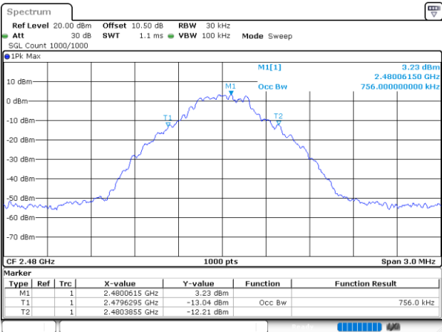
DH5_High
