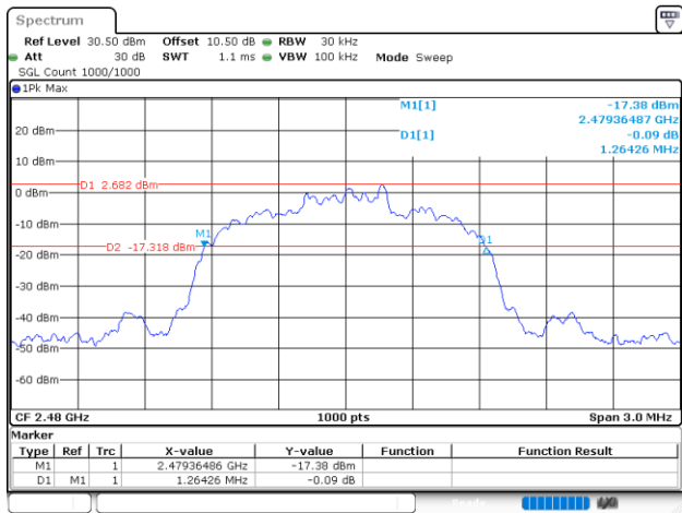
3DH5_High
