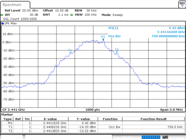
DH5_Middle
