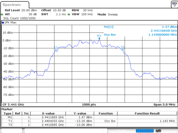
2DH5_Middle
