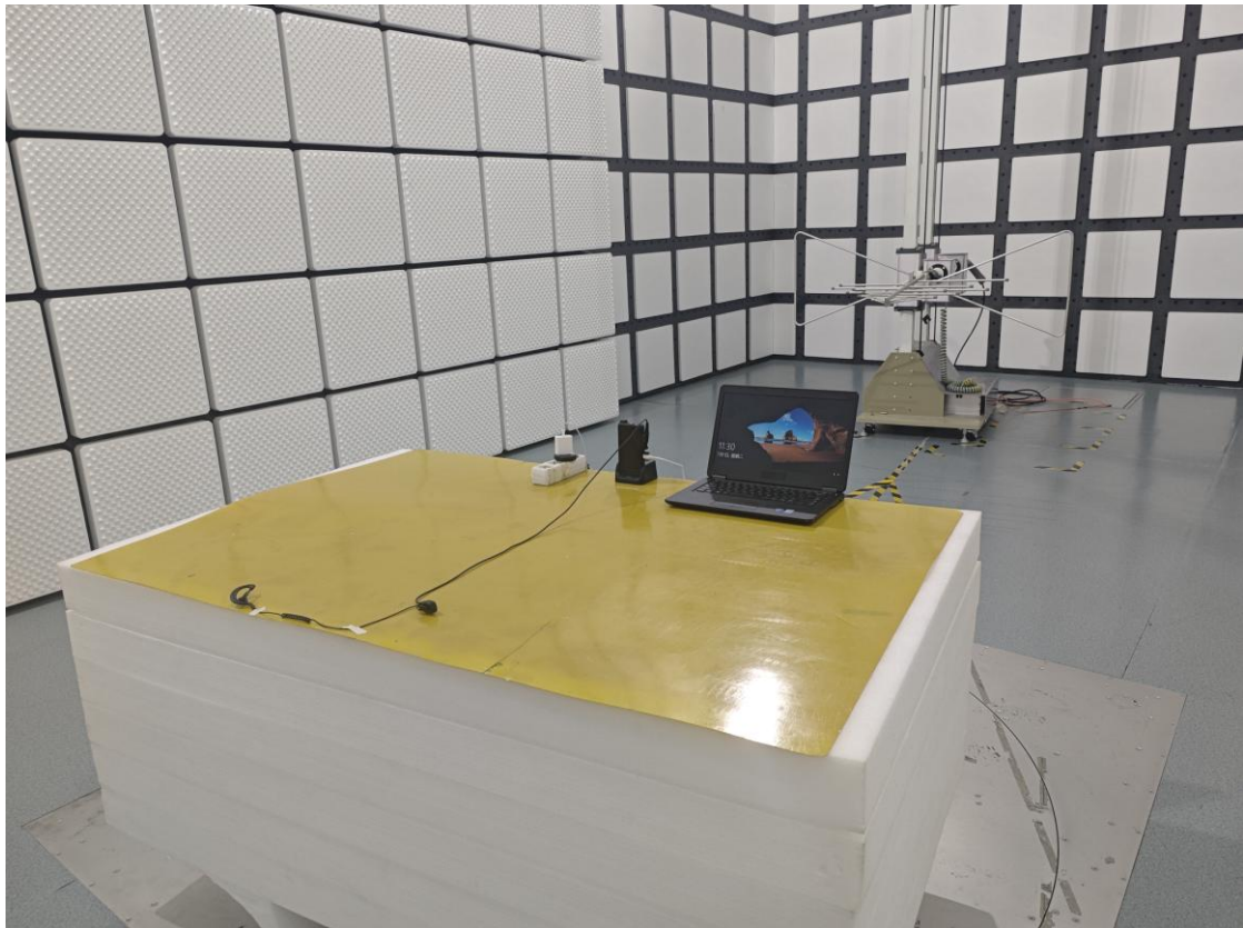
Radiated Spurious Emissions Test View (30MHz-1GHz) (Test Mode 2)
