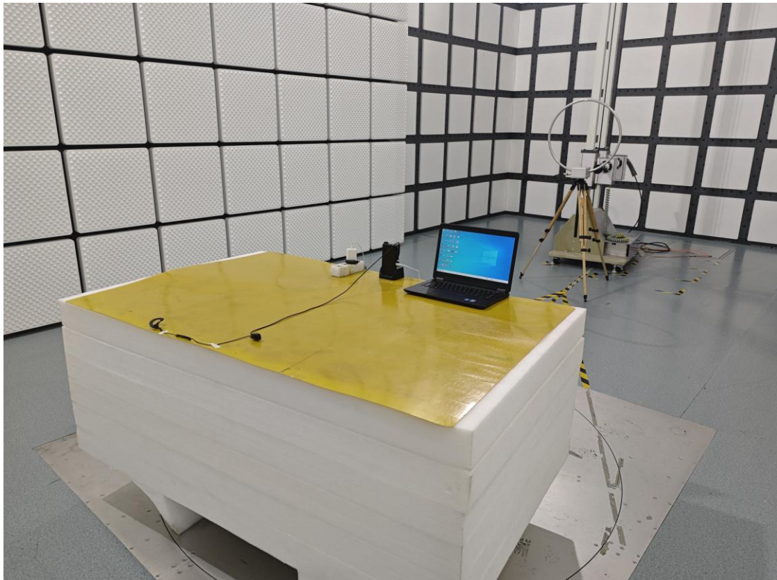
Radiated Spurious Emissions Test View (9kHz-30MHz) (Test Mode 2)
