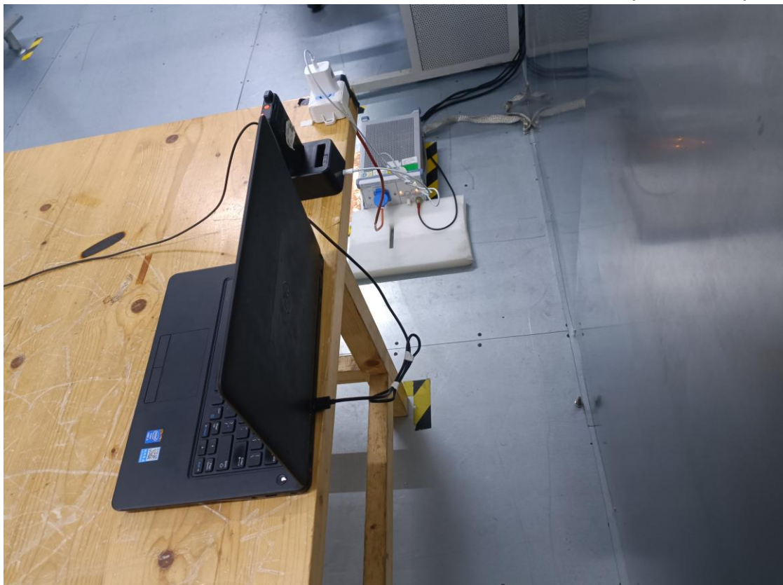
Photo of Power Line Conducted Emission Measurement-Side View(Test Mode 2)
