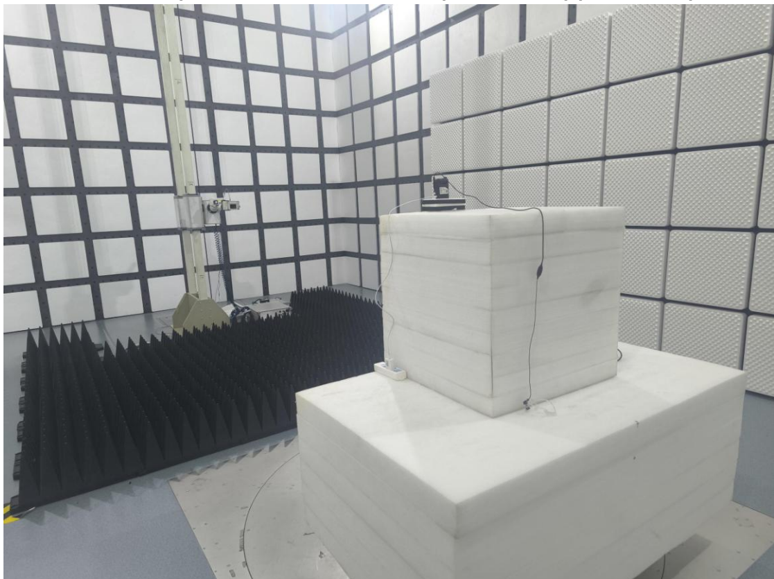
Radiated Spurious Emissions Test View (Above 18GHz) (Test Mode 1)
