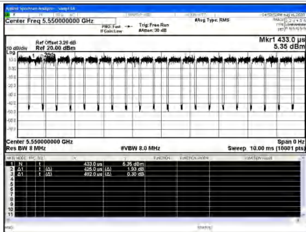
Duty Cycle NVNT ax40 5550MHz Ant0
