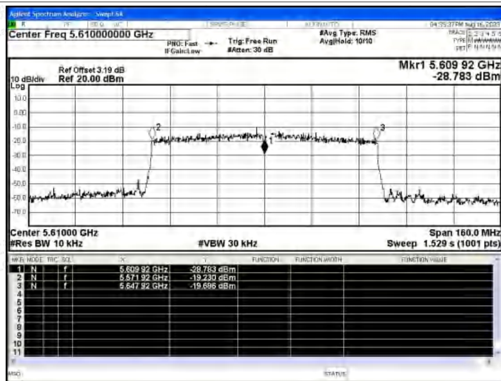
Freq. Stability NVNT ac80 5610MHz Ant0
