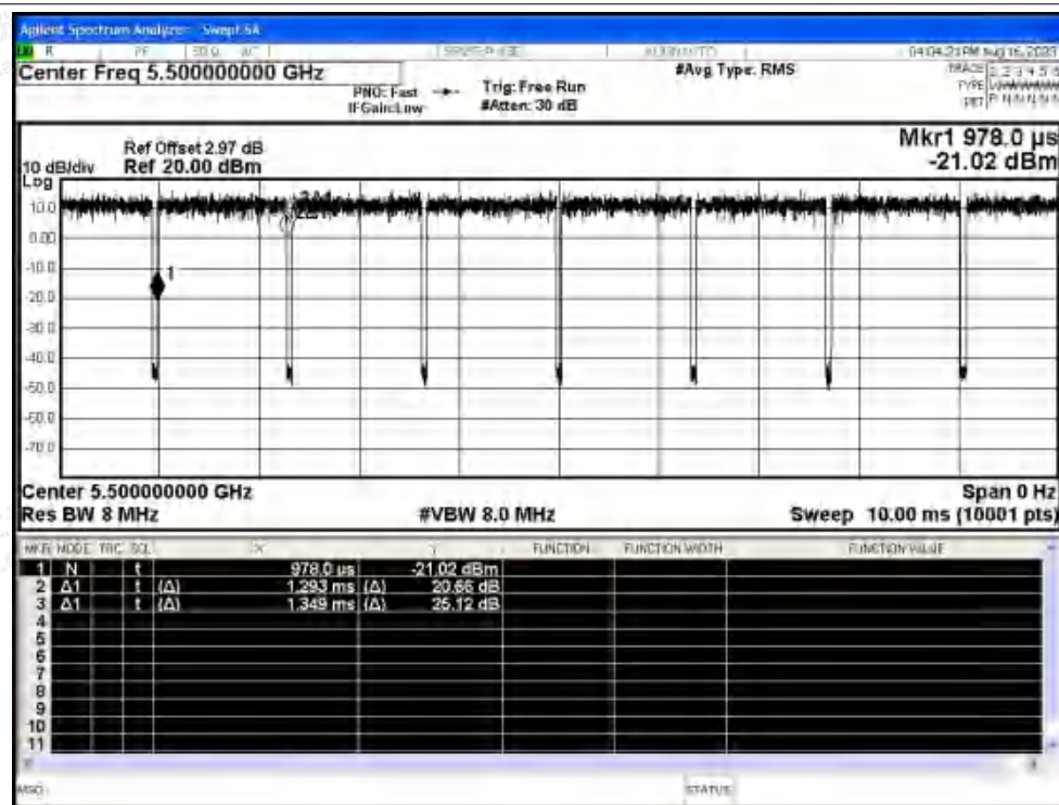
Duty Cycle NVNT n20 5500MHz Ant0
