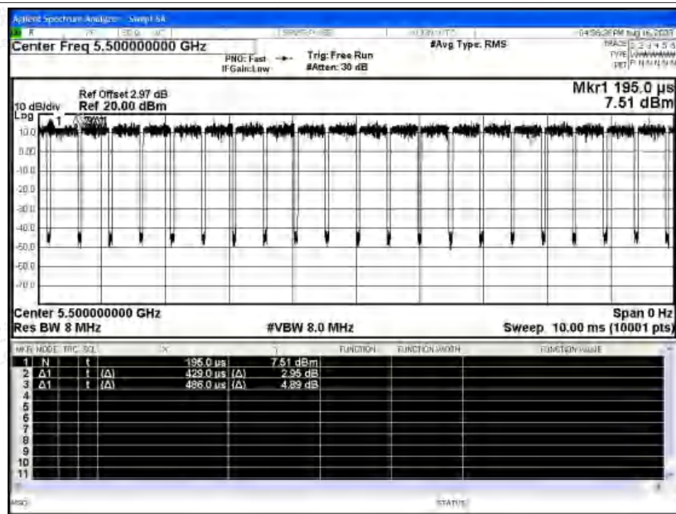
Duty Cycle NVNT ax20 5500MHz Ant0
