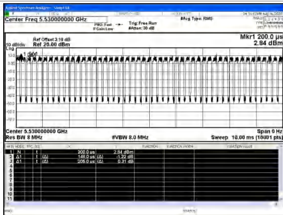
Duty Cycle NVNT ac80 5530MHz Ant0
