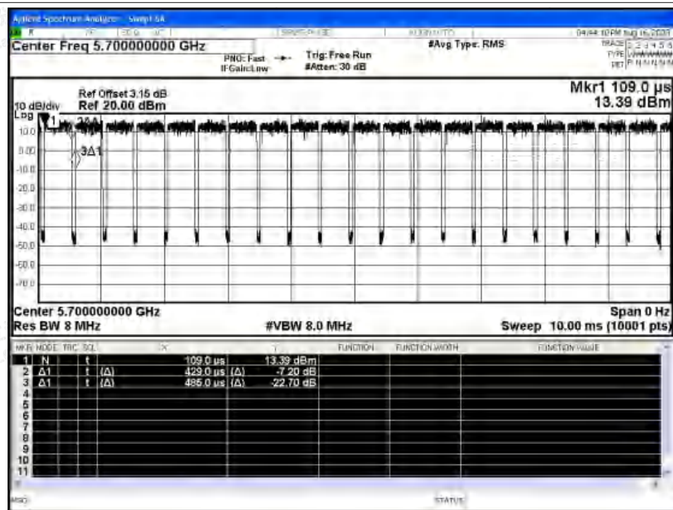
Duty Cycle NVNT ax20 5700MHz Ant0
