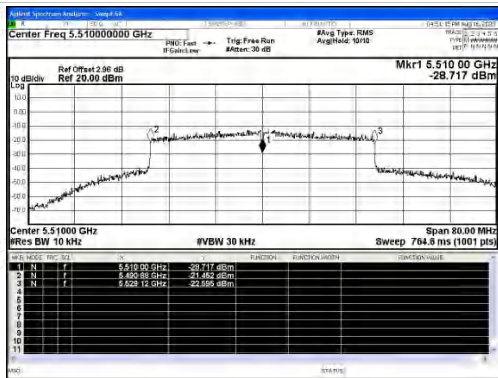
Freq. Stability NVNT ax40 5510MHz Ant0
