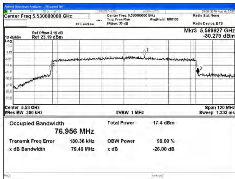
-26dB Bandwidth NVNT ax80 5530MHz Ant0
