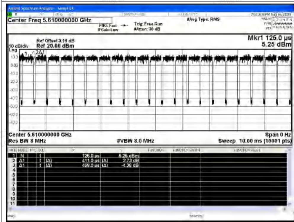
Duty Cycle NVNT ax80 5610MHz Ant0
