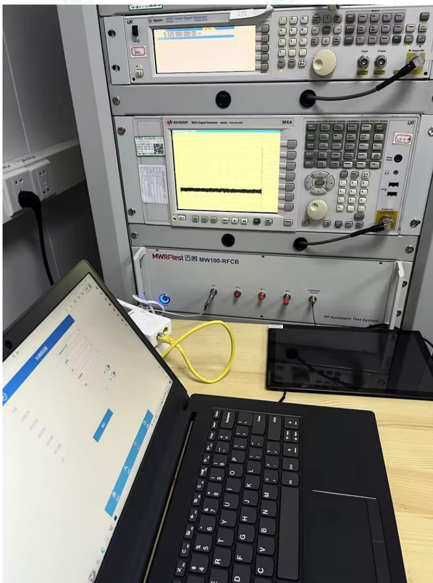
Test Setup Photo(s) of Radiated Emissions Measurement
