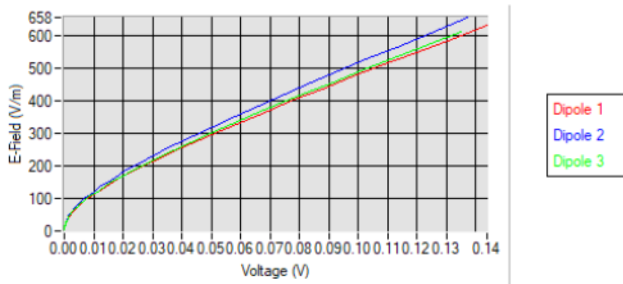
Calibration curves
