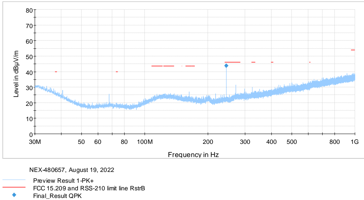
Figure 8.6-2: Field strength of spurious emissions above 30 MHz
