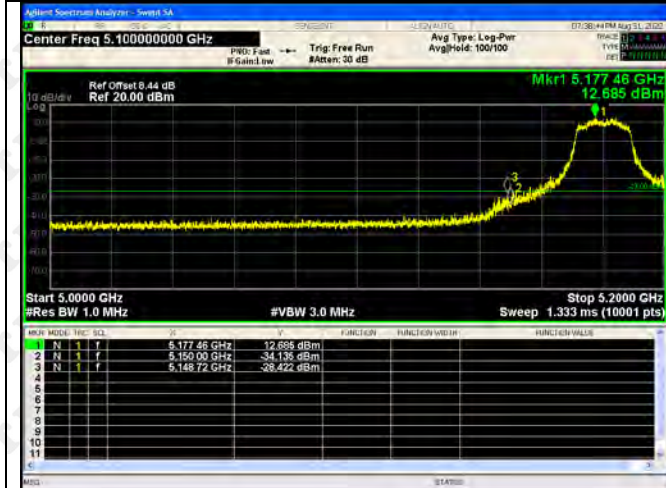
802.11ac(VH40)-5190
