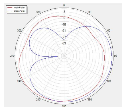
Theta=90 freq=2450MHz
