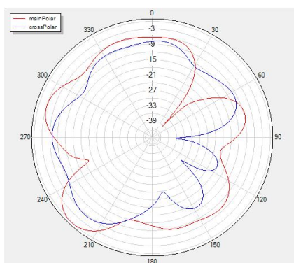
Phi=0 freq=2450MHz
