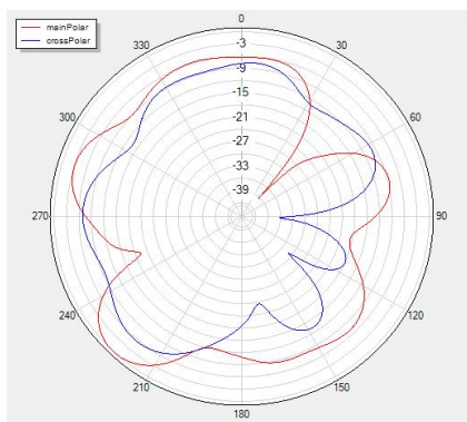
Phi=0 freq=2450MHz
