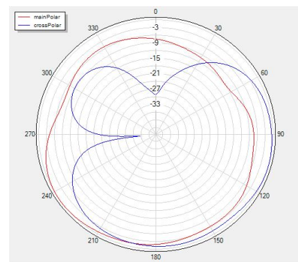
Theta=90 freq=2450MHz
