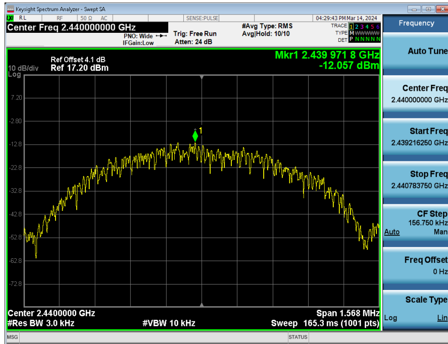
Power_Spectral_Density_NVNT_ANT1_1Mbps_2440
