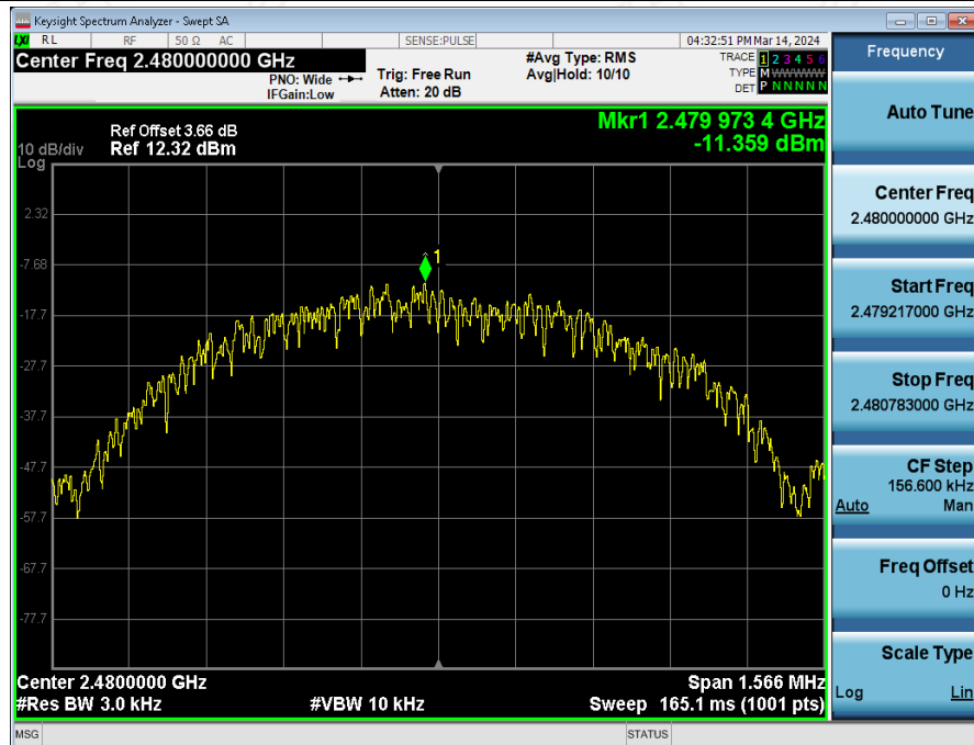
Power_Spectral_Density_NVNT_ANT1_1Mbps_2480
