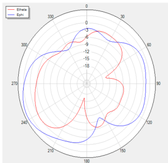
H Theta=90 freq=2450MHz
