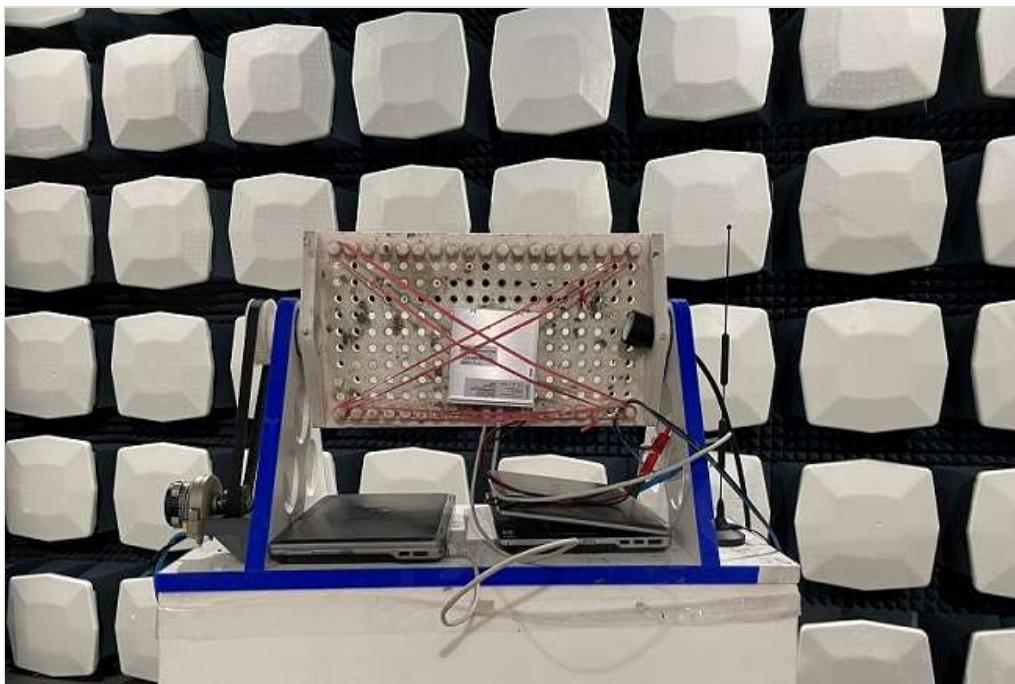
Photograph 4: EUT test setup in the fully anechoic chamber, close up view
