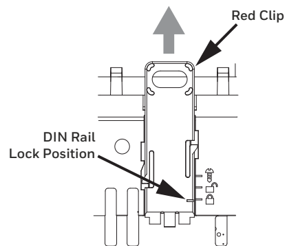
Fig. 7 Lock Position
