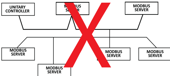
Fig. 34 Prohibited Wiring Topology (example)
