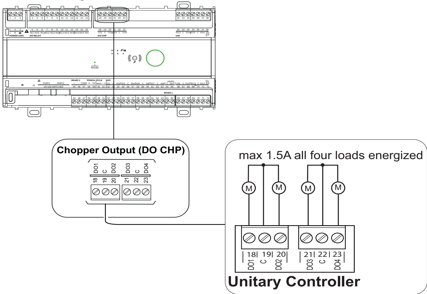
Fig. 17 DO (CHP) Wiring Example
