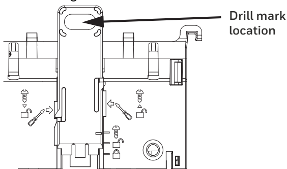
Fig. 10 Drill mark location
