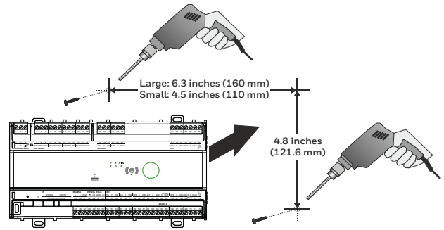
Fig. 11 Mounting and Dismounting
