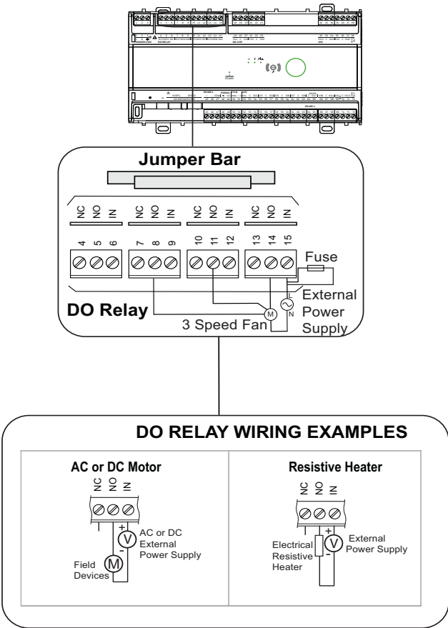
Fig. 19 DO Relay Wiring Examples
