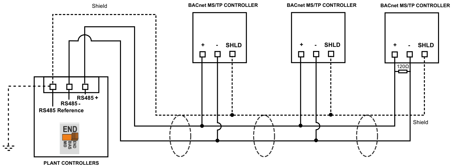
Fig. 22 Connection to a BACnet™ MS/TP Bus
