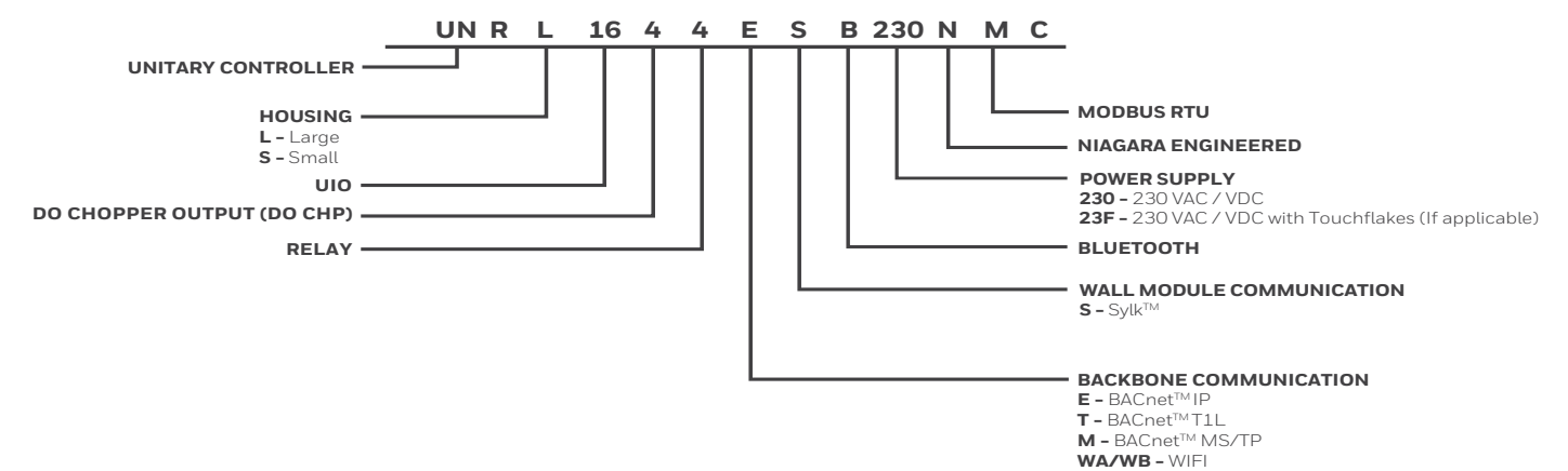
Fig. 1 Controller Part Numbers
