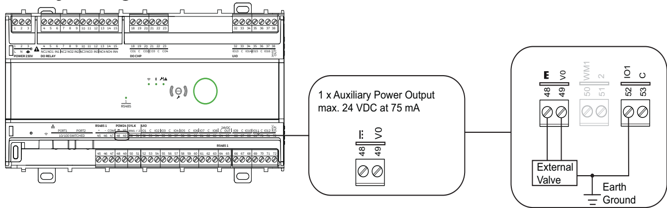
Fig. 18 Auxiliary Wiring Examples
