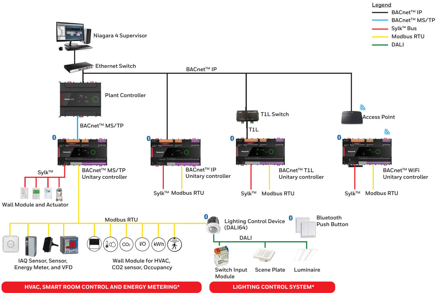
Fig. 5 System Overview
