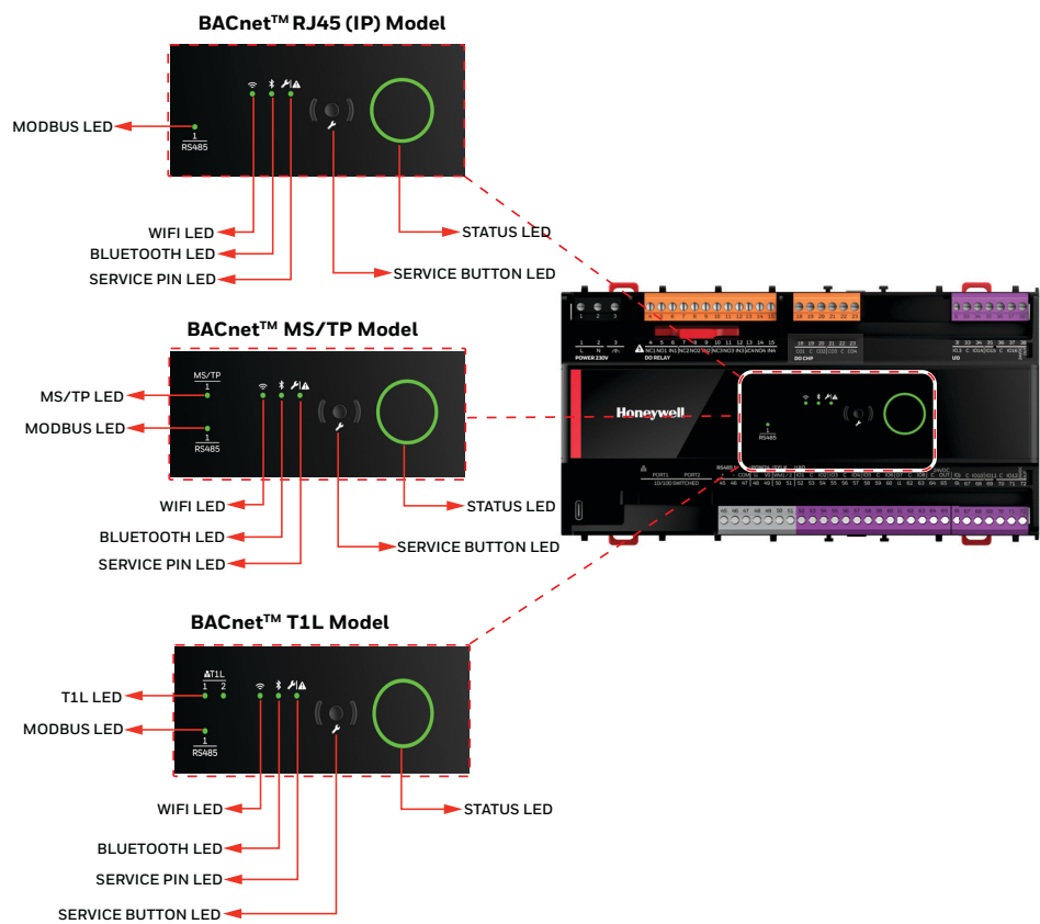
Fig. 36 LED Interface
