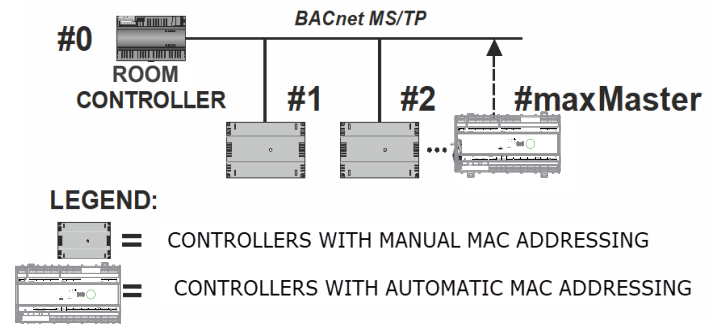
Fig. 23 Automatic MAC Addressing
