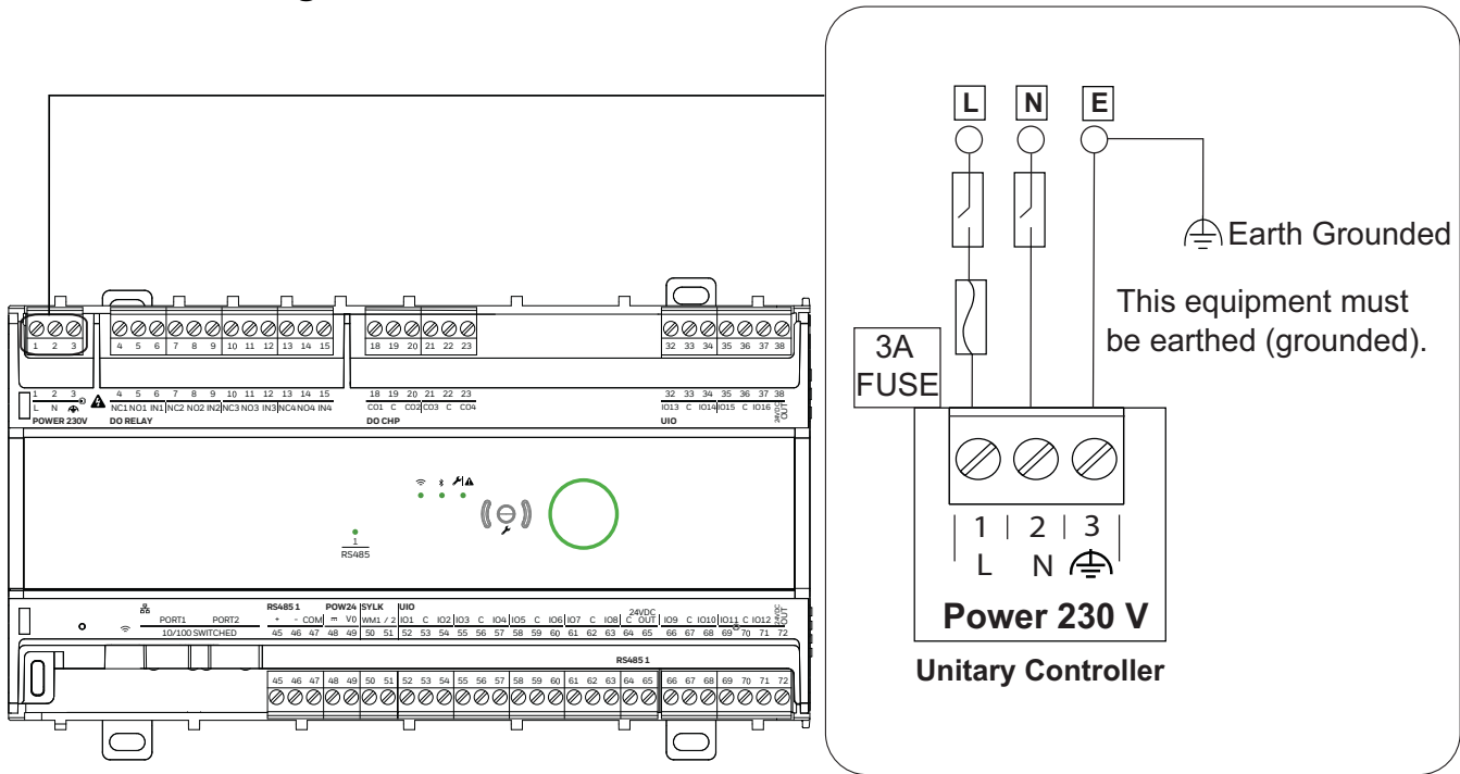
Fig. 12 Power Wiring Examples
