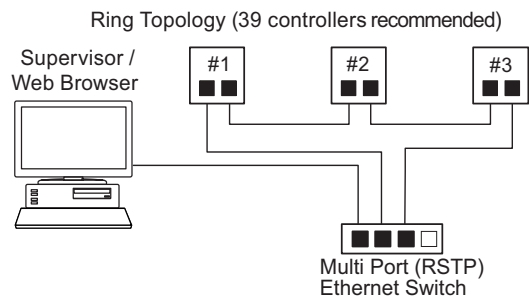
Fig. 21 Ring Topology
