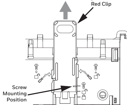
Fig. 9 Screw Mounting Position
