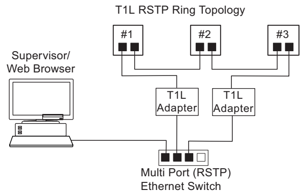
Fig. 27 T1L Ring Topology
