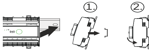
Fig. 8 Controller mounting on DIN Rail
