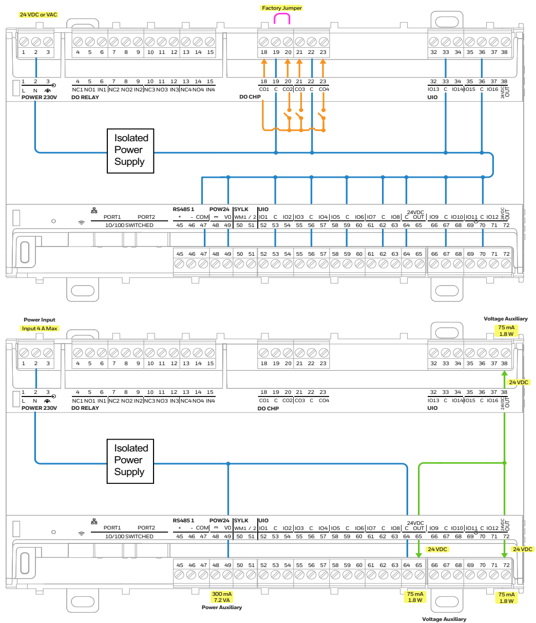
Fig. 14 Internal Wiring Large controller
