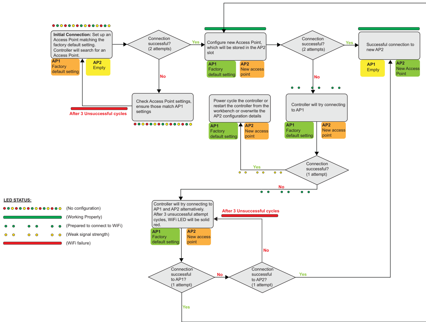
Fig. 32 WiFi Access Point Connection flow chart
