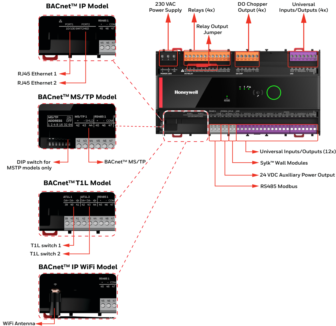
Fig. 4 Hardware Overview
