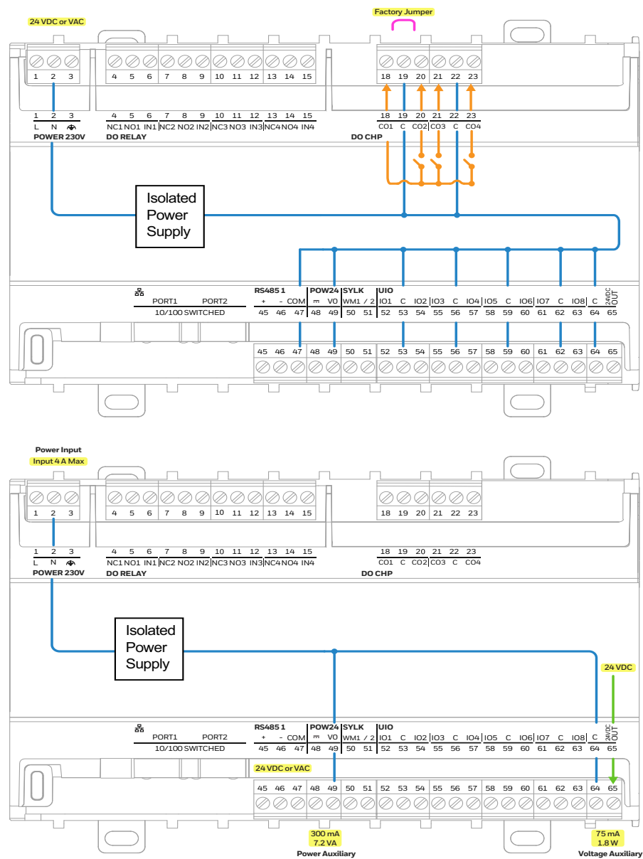
Fig. 15 Internal Wiring Small controller
