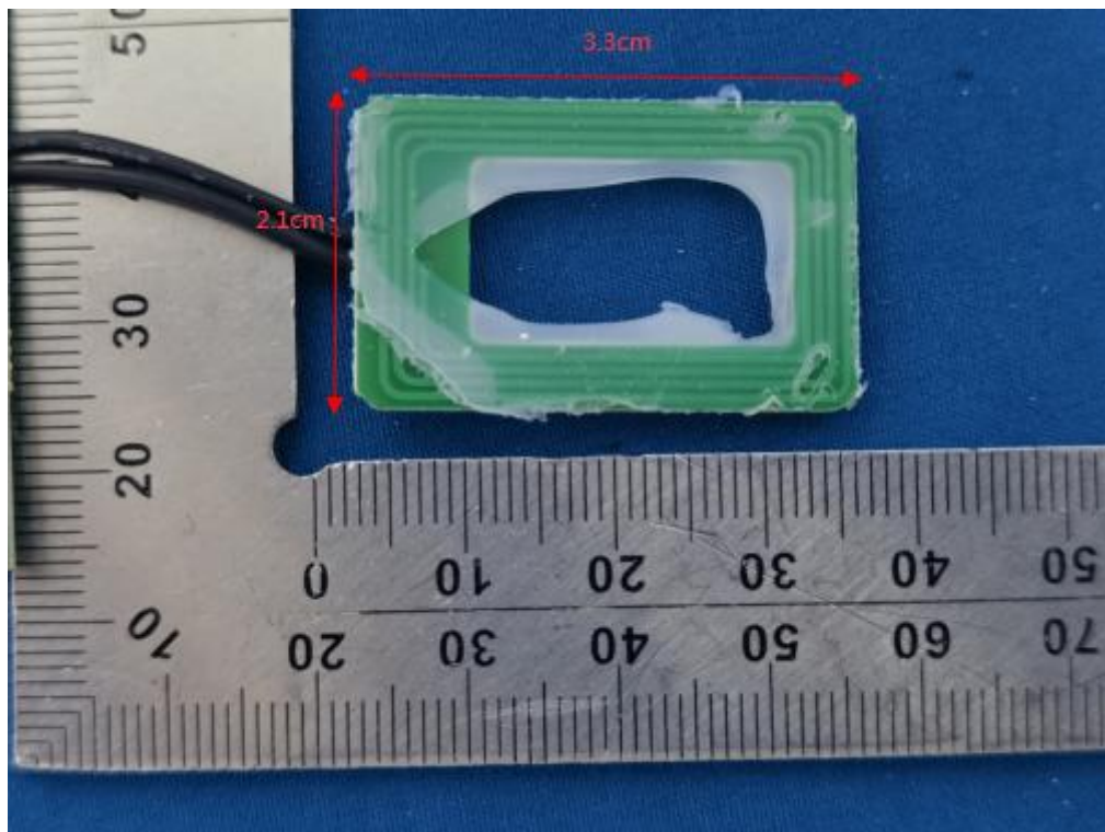
Antenna Diagram-2
