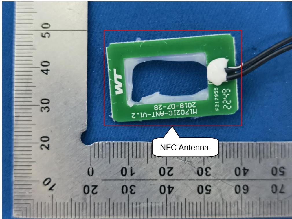
Antenna Diagram-2
