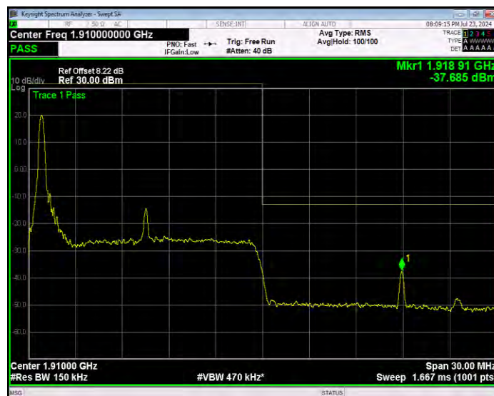
Band2 16QAM BW=15MHz Channel=19125 RB Size=1 Position=#Max Extended
