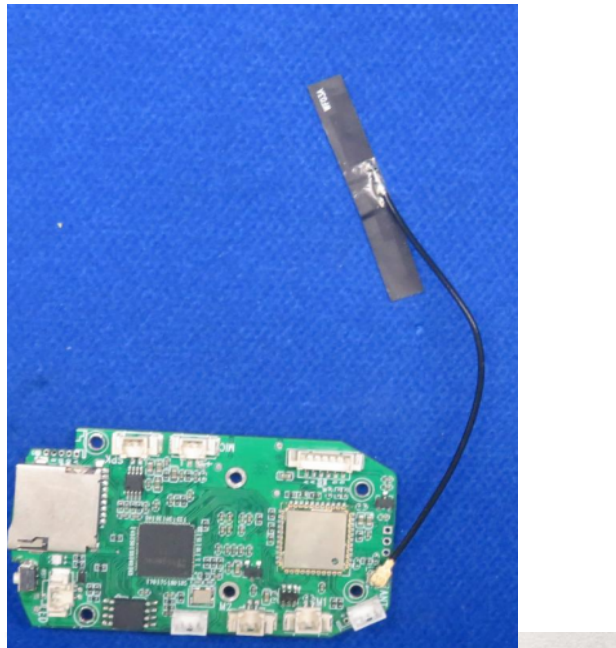
Antenna Picture
