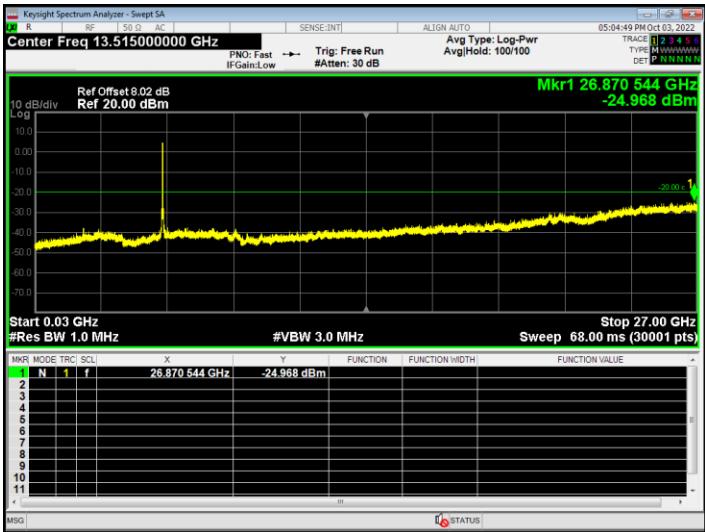
Tx. Spurious NVNT ax80 5210MHz Ant1 Emission
