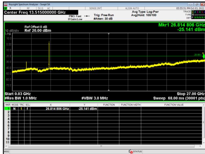
Tx. Spurious NVNT ax40 5230MHz Ant2 Emission
