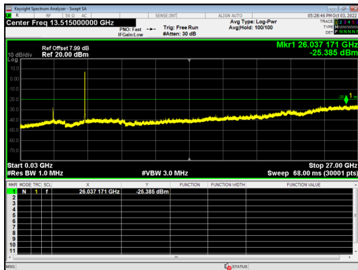
Tx. Spurious NVNT n20 5220MHz Ant2 Emission
