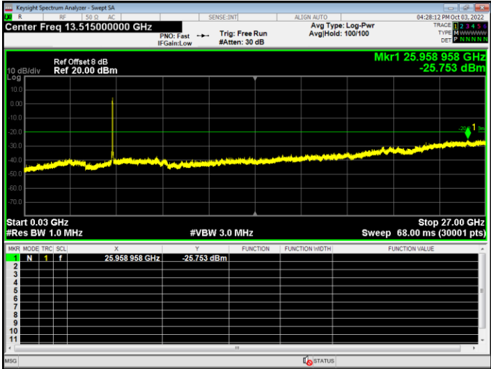
Tx. Spurious NVNT ac40 5230MHz Ant1 Emission
