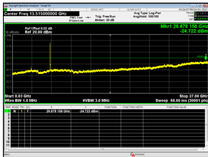
Tx. Spurious NVNT ac20 5240MHz Ant1 Emission
