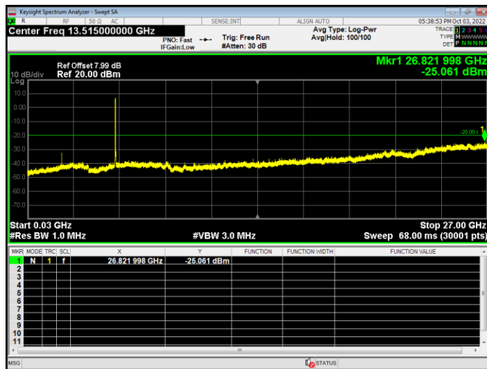
Tx. Spurious NVNT ac20 5220MHz Ant2 Emission
