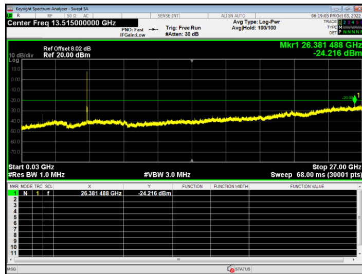
Tx. Spurious NVNT ax20 5240MHz Ant1 Emission
