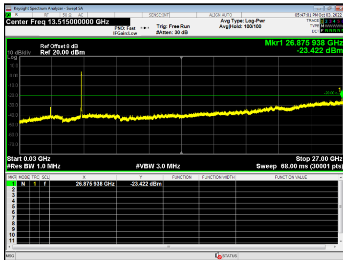
Tx. Spurious NVNT ac40 5230MHz Ant2 Emission
