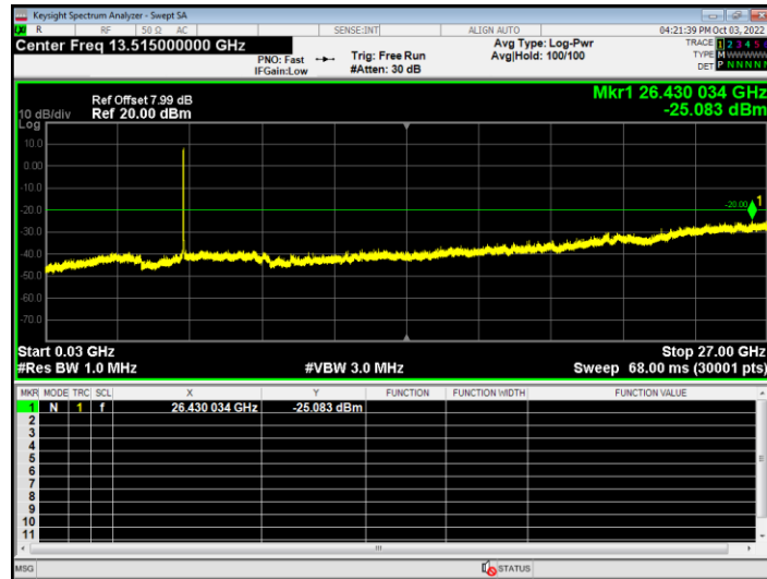
Tx. Spurious NVNT ac20 5220MHz Ant1 Emission
