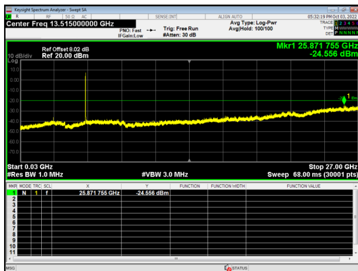
Tx. Spurious NVNT n20 5240MHz Ant2 Emission
