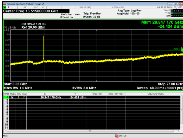
Tx. Spurious NVNT ax20 5220MHz Ant2 Emission
