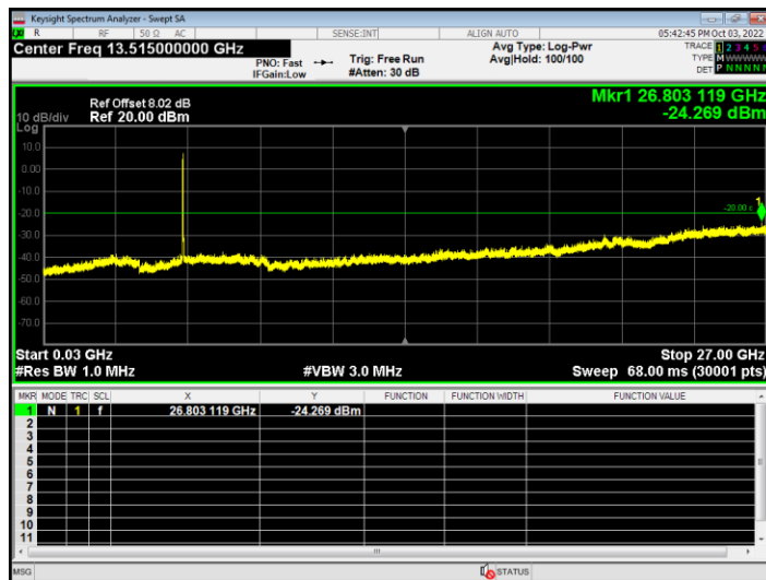
Tx. Spurious NVNT ac20 5240MHz Ant2 Emission
