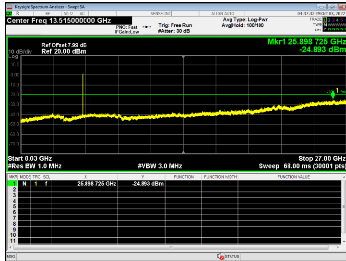
Tx. Spurious NVNT ax20 5220MHz Ant1 Emission
