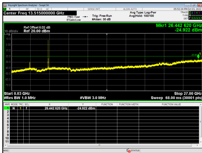
Tx. Spurious NVNT ax20 5240MHz Ant2 Emission
