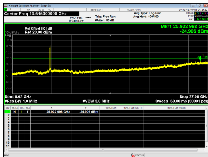
Tx. Spurious NVNT ax80 5210MHz Ant2 Emission
