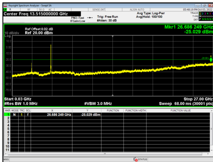
Tx. Spurious NVNT ac80 5210MHz Ant2 Emission
