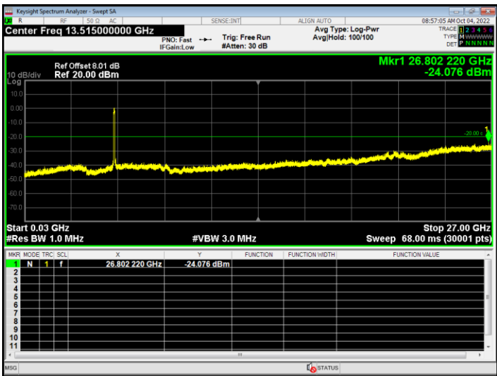
Tx. Spurious NVNT ac80 5210MHz Ant1 Emission
