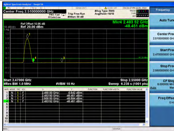
BLE_1M_Ant1_High_2480_Peak
