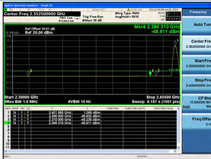
BLE_1M_Ant1_Low_2402_Peak
