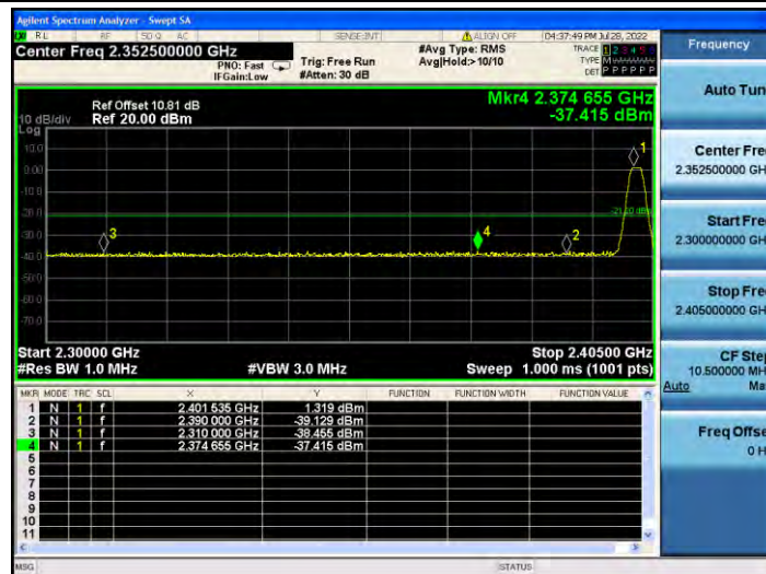
BLE_2M_Ant1_Low_2402_Peak
