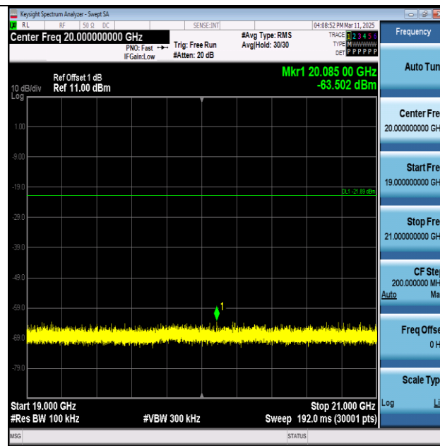
BLE_1M-Ant1-2402-19000~21000-PASS
