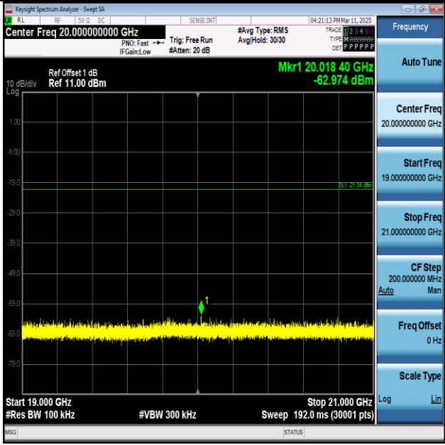
BLE_1M-Ant1-2440-19000~21000-PASS
