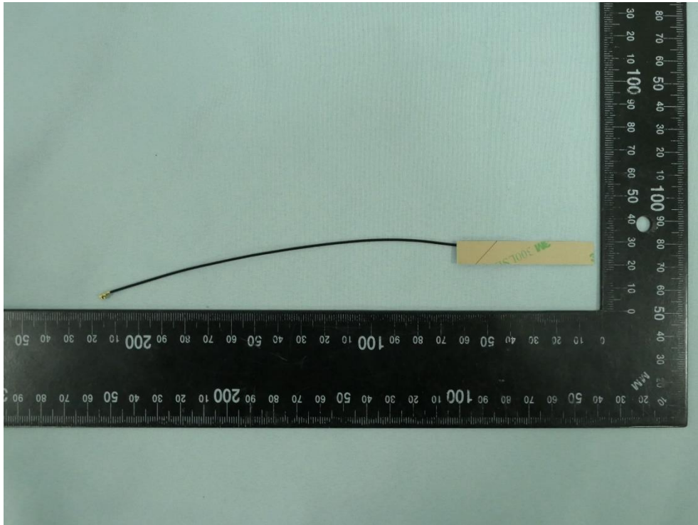
(12) EUT Photo - Raptor.Drone.ANT1.C113.382B.1
