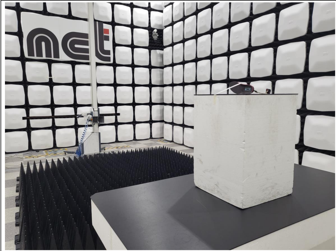
Above 1 GHz_Left
