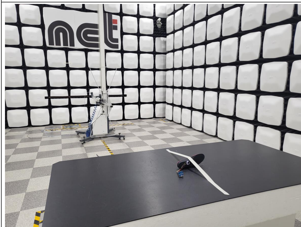
Below 1 GHz_Left
