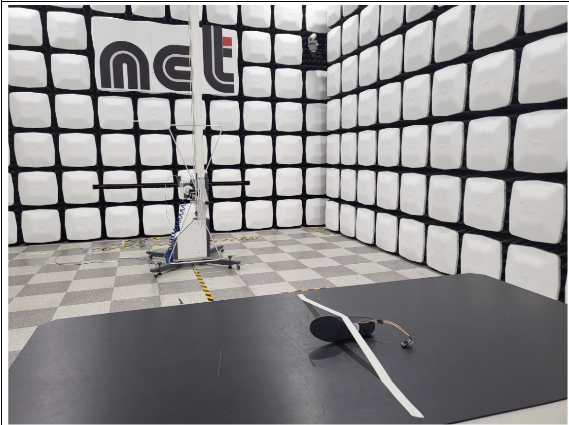
Below 1 GHz_Right
