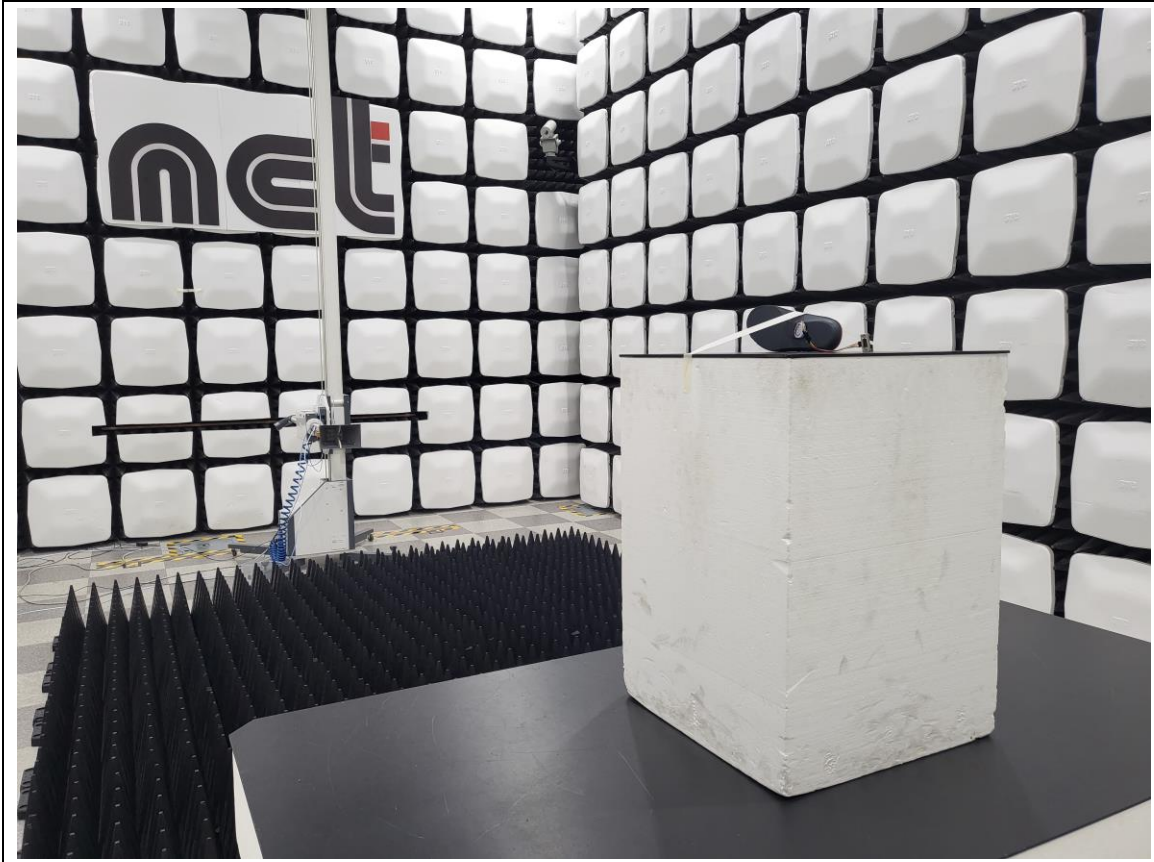
Above 1 GHz_Right
