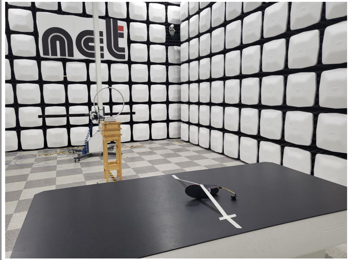
Below 30 MHz_Right
