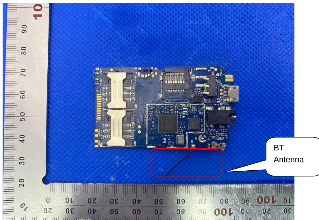
INTERNAL VIEW OF EUT (FIGURE 1)
