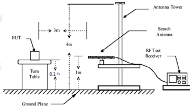
Above 1GHz
