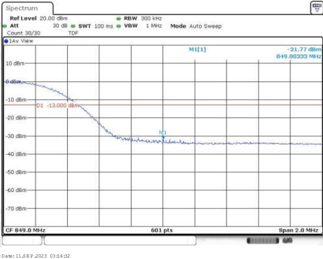
Band26-15MHz-16QAM-26965-75RB#0
