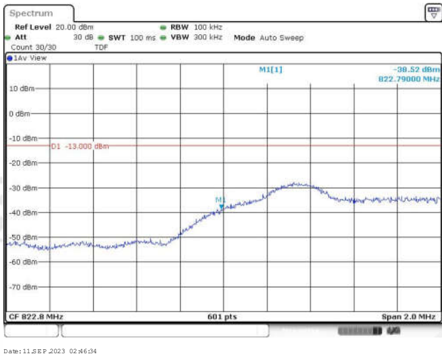
Band26-5MHz-16QAM-26803-25RB#0
