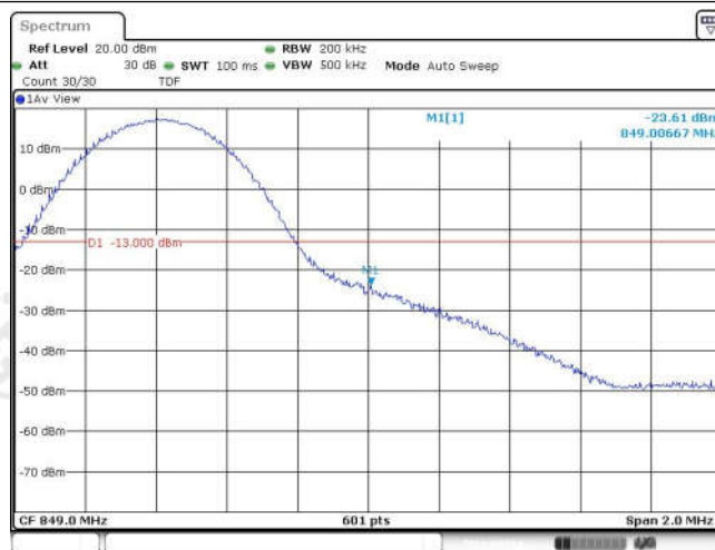
Band26-10MHz-16QAM-26990-50RB#0
