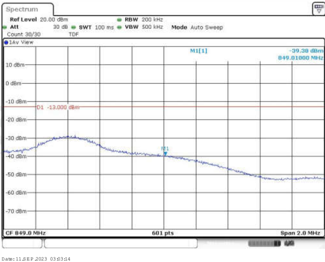
Band26-10MHz-16QAM-26990-1RB#49
