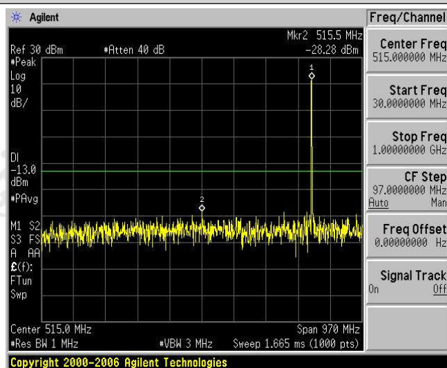
Band26-3MHz-16QAM-27025-1RB#0-Range2:1000~10000MHz
