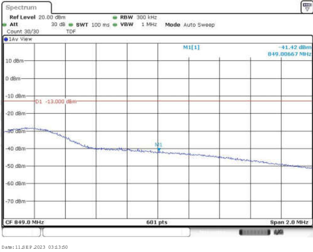
Band26-15MHz-16QAM-26965-1RB#74
