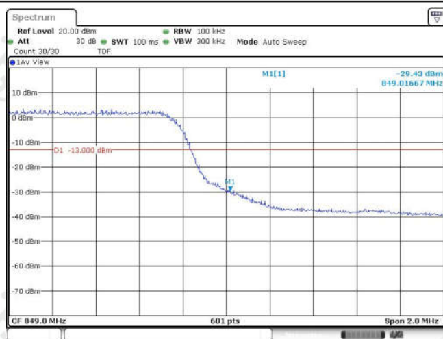
Band26-5MHz-QPSK-27015-25RB#0
