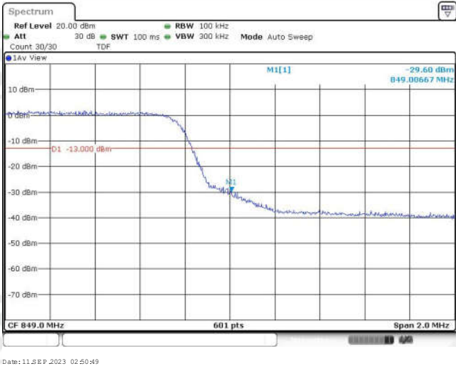
Band26-10MHz-QPSK-26828-1RB#0
