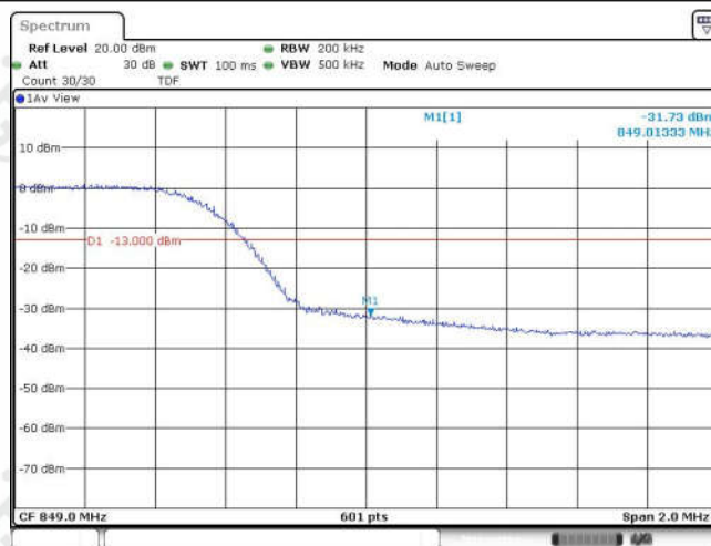
Band26-10MHz-16QAM-26990-50RB#0
