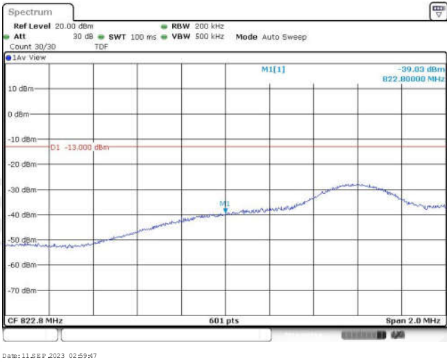
Band26-10MHz-16QAM-26828-50RB#0
