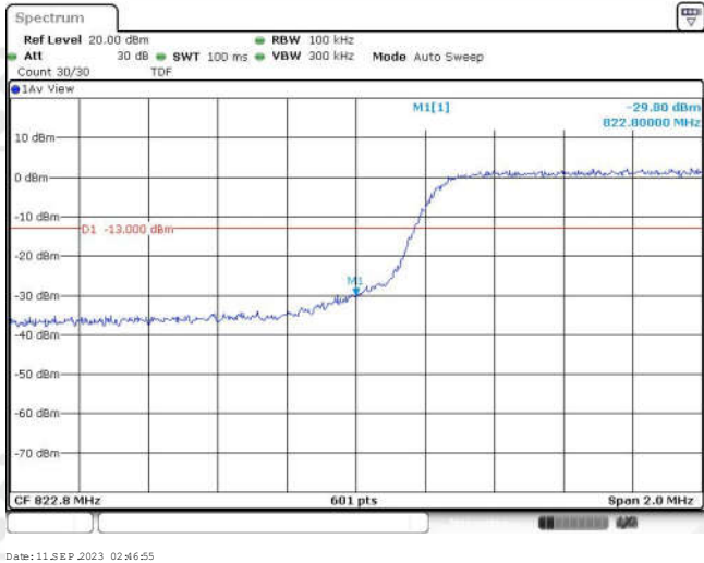
Band26-5MHz-16QAM-27015-1RB#0
