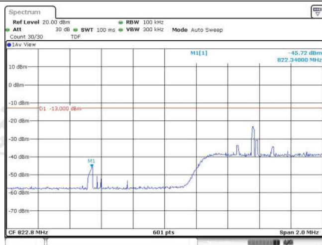
Band26-5MHz-16QAM-26803-1RB#0
