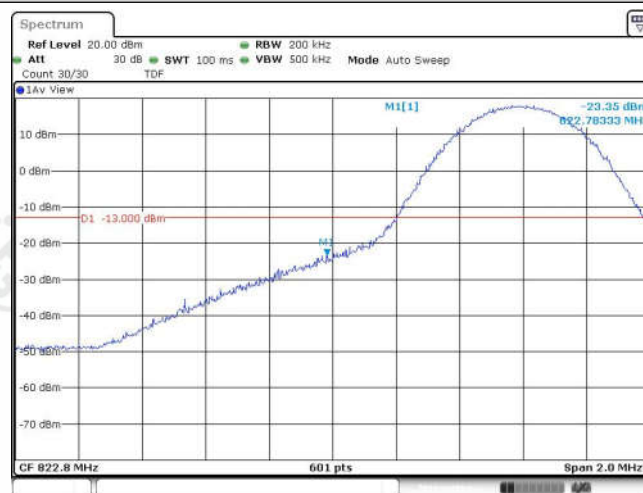
Band26-10MHz-16QAM-26828-1RB#0
