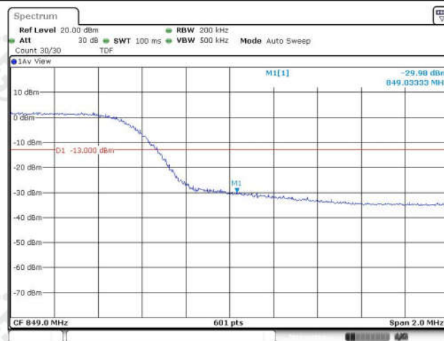
Band26-10MHz-QPSK-26990-50RB#0
