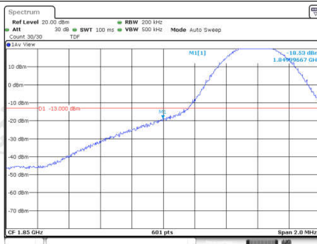
Band25-10MHz-QPSK-26090-1RB#0
