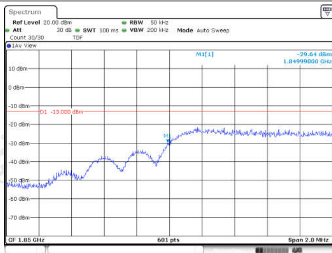
Band25-3MHz-16QAM-26055-15RB#0
