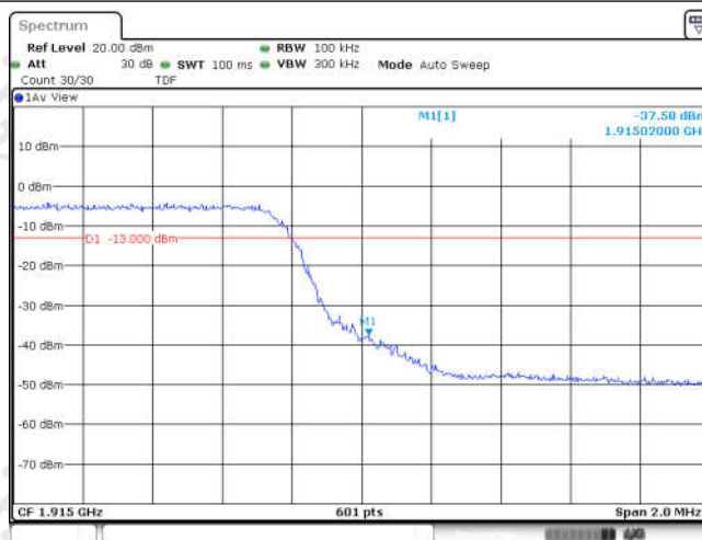
Band25-5MHz-16QAM-26665-25RB#0
