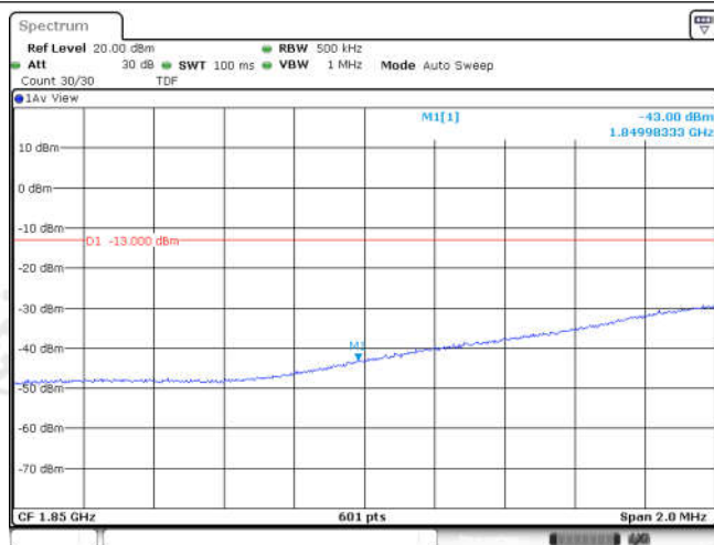
Band25-20MHz-QPSK-26140-100RB#0
