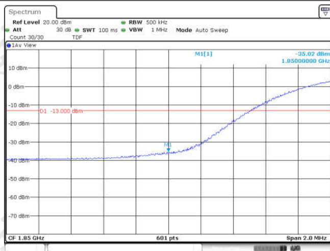
Band25-20MHz-QPSK-26140-100RB#0
