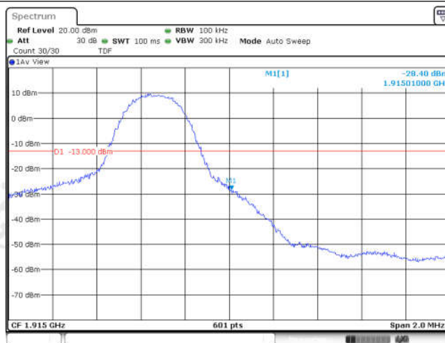
Band25-5MHz-16QAM-26665-25RB#0
