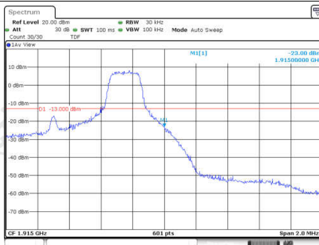
Band25-1.4MHz-QPSK-26683-1RB#5
