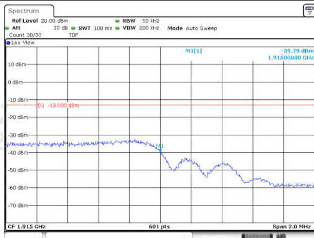
Band25-3MHz-16QAM-26675-1RB#0
