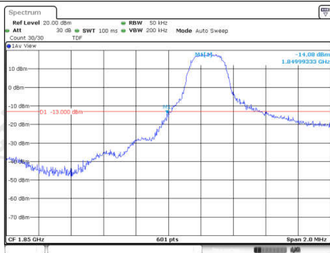
Band25-3MHz-16QAM-26055-1RB#0
