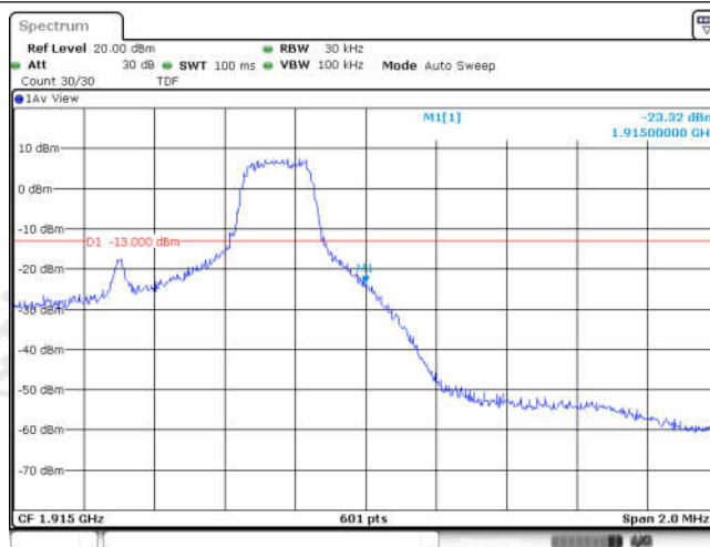
Band25-1.4MHz-16QAM-26683-6RB#0
