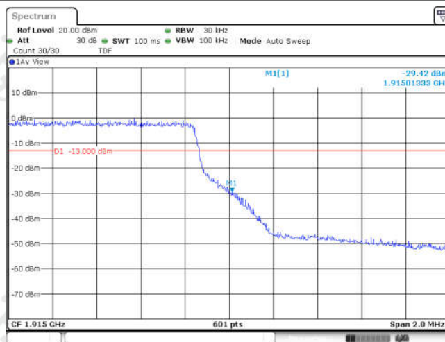
Band25-1.4MHz-16QAM-26683-6RB#0
