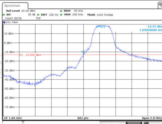
Band25-3MHz-QPSK-26055-1RB#0
