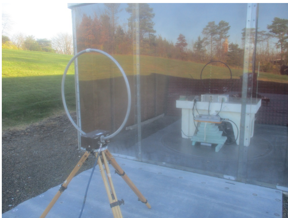
Parallel Antenna Polarization with VCC
