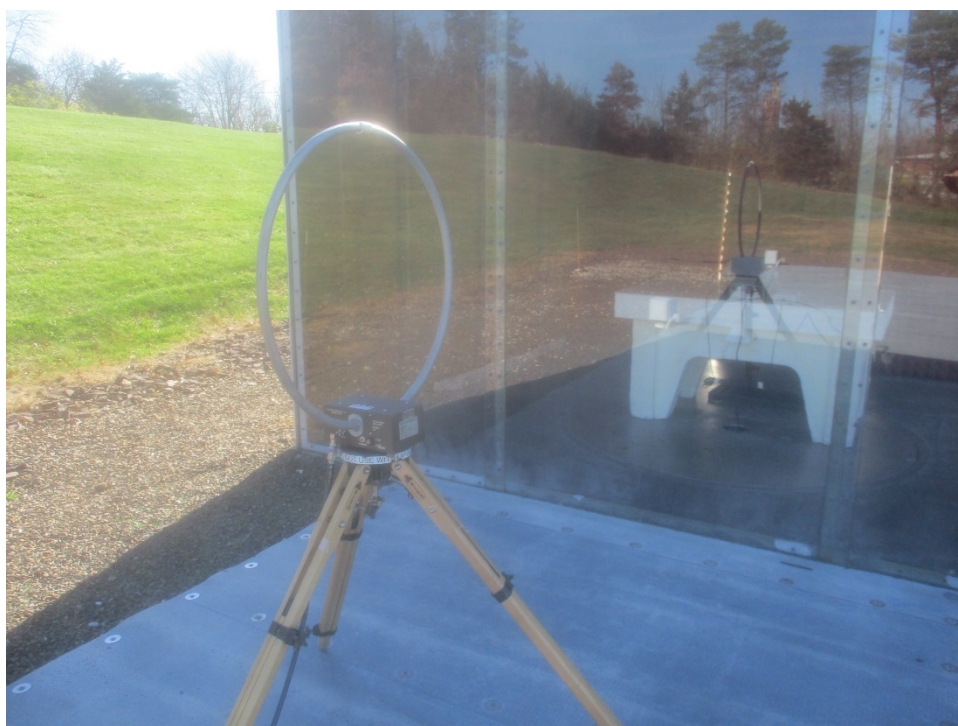
Perpendicular Antenna Polarization, Standalone
