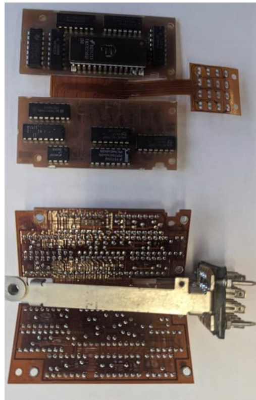
g) Transmitter Control Module (left) & Memory Module (right)-PCB Photos
