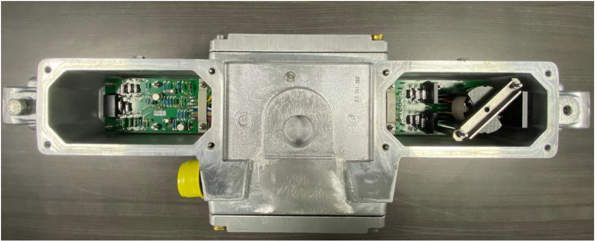
c) PCB Front
