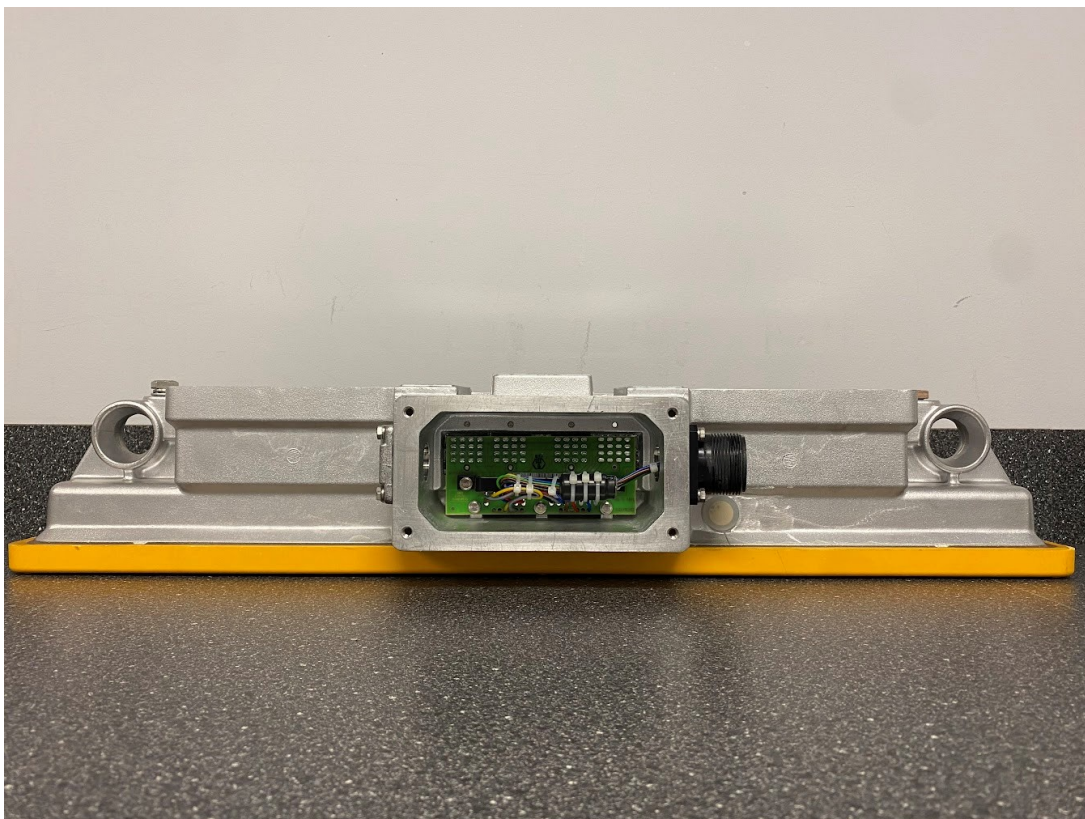
a) Track Coupling Coil
