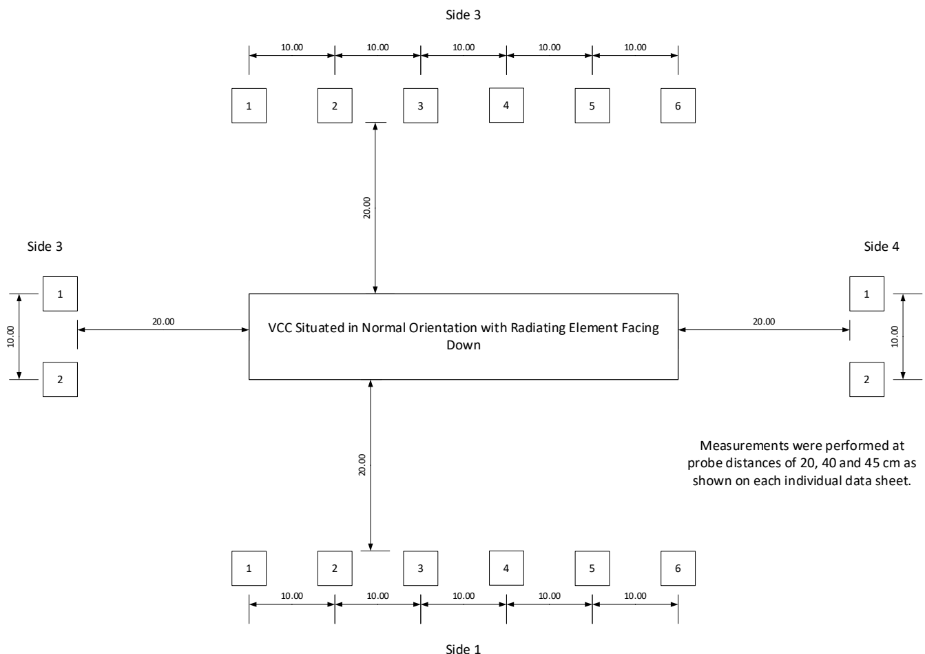
Figure 1 - Test Positions in Normal Orientation
