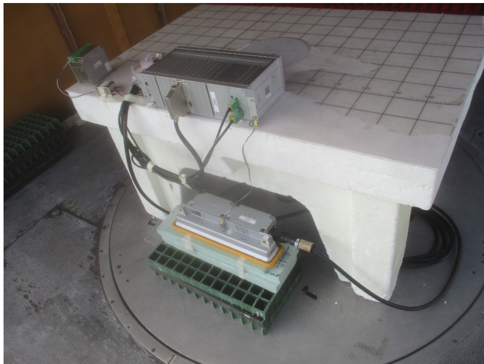
EUT Configuration, VCC without TCC
