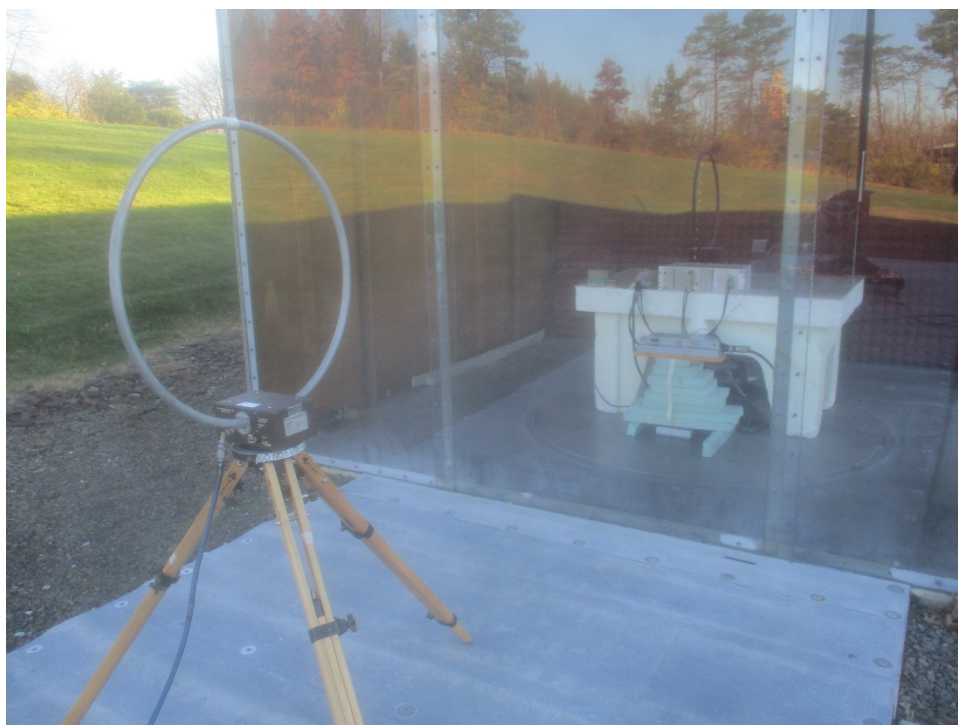
Perpendicular, 850 kHz with IMU Antenna
