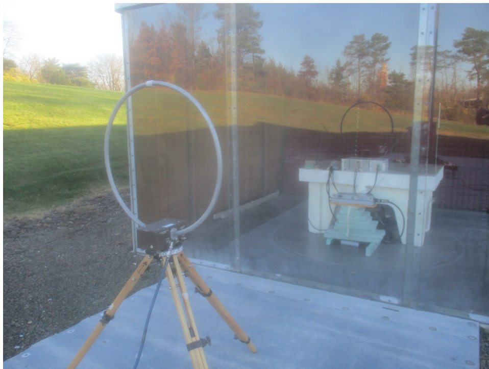
Parallel, 850 kHz with IMU Antenna
