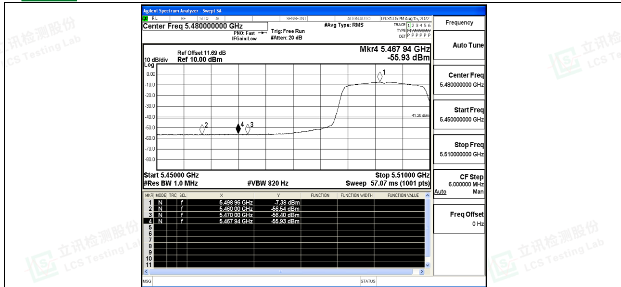
11N20SISO_Ant0_Low_5500_Peak
