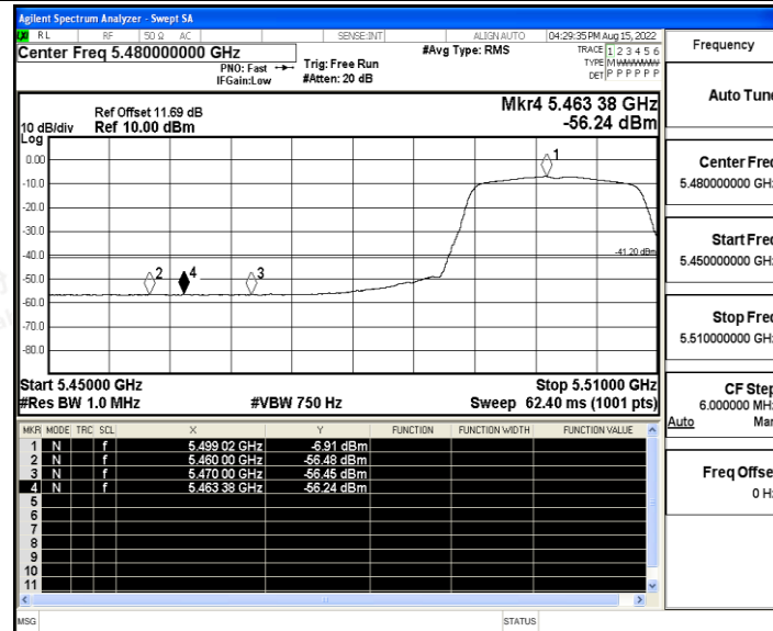
11A_Ant0_Low_5500_Peak
