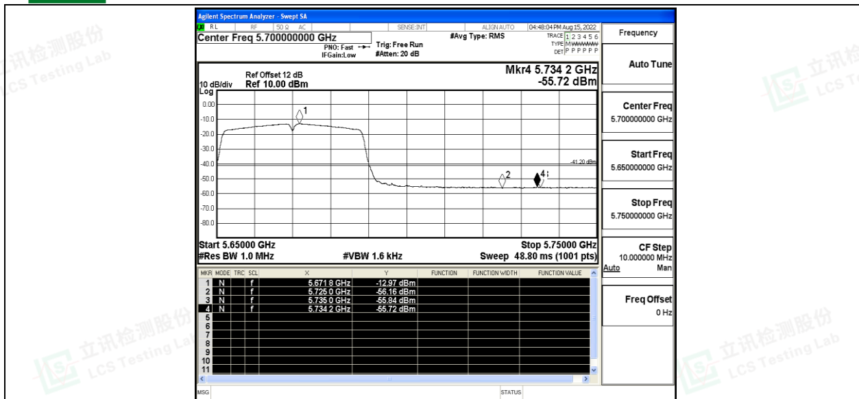
11AC40SISO_Ant1_High_5670_Peak
