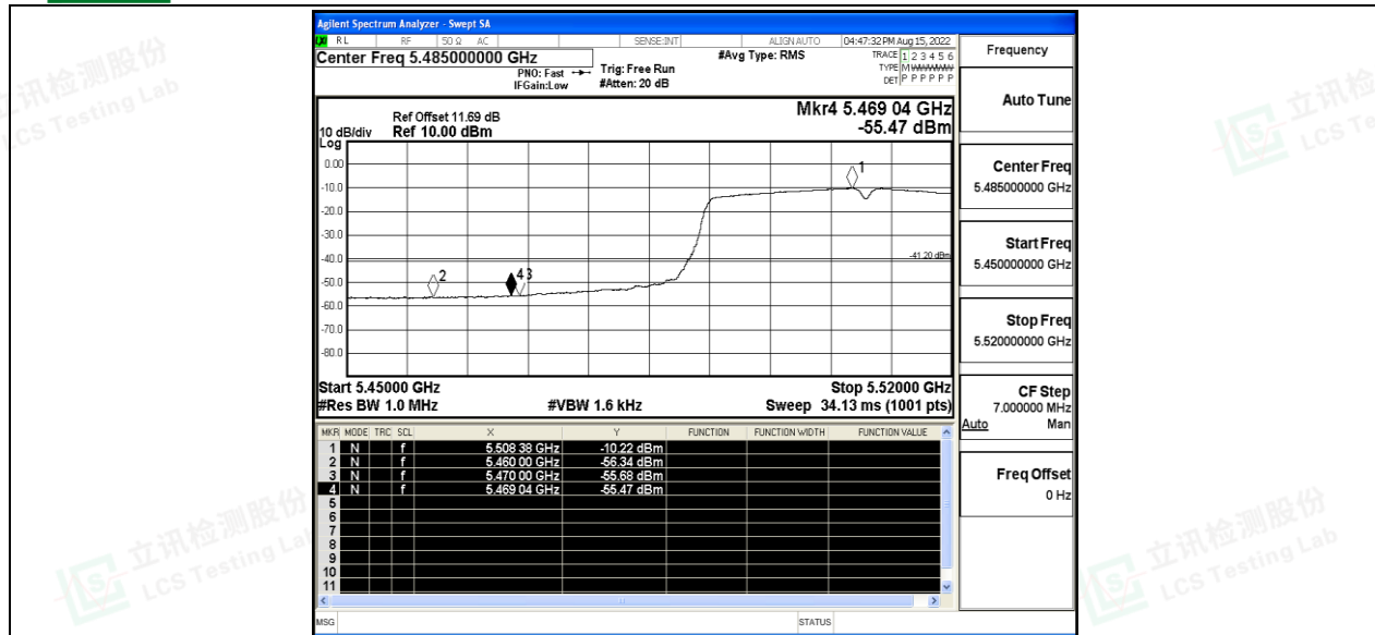
11AC40SISO_Ant1_Low_5510_Peak
