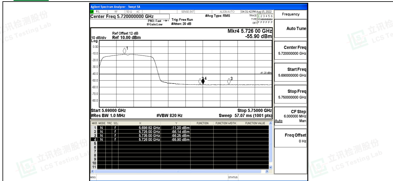
11N20SISO_Ant0_High_5700_Peak
