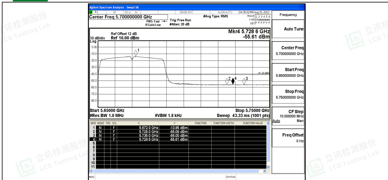
11N40SISO_Ant0_High_5670_Peak
