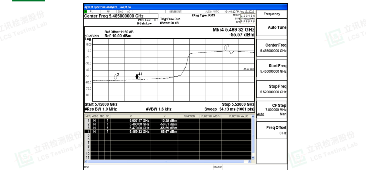
11N40SISO_Ant1_Low_5510_Peak
