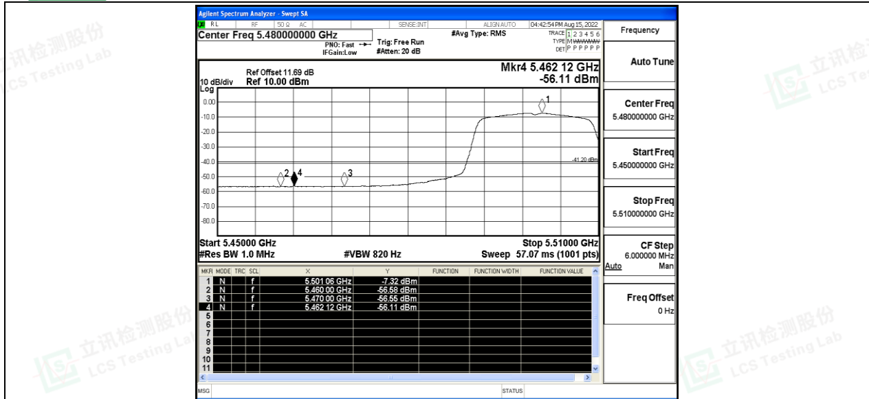
11N20SISO_Ant1_Low_5500_Peak
