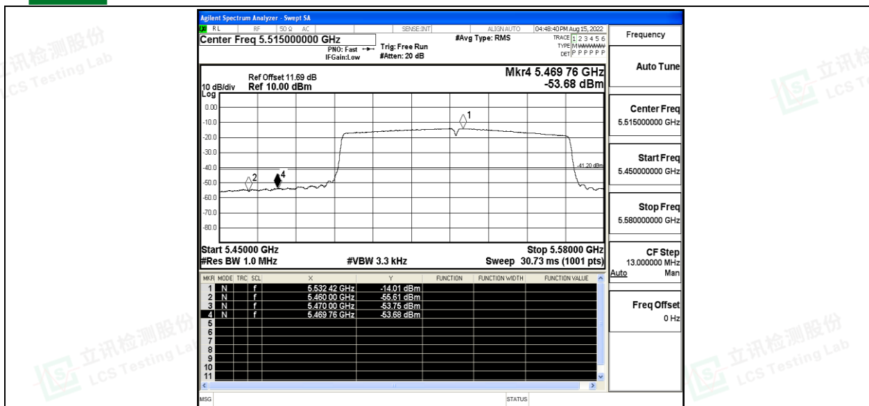
11AC80SISO_Ant1_Low_5530_Peak
