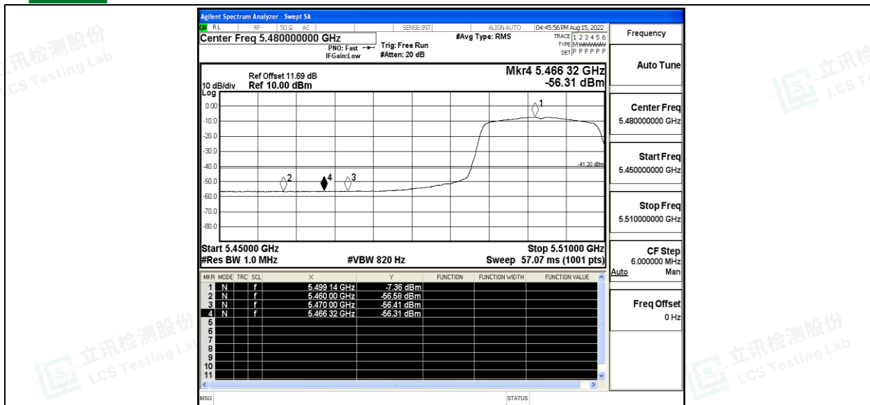
11AC20SISO_Ant1_Low_5500_Peak
