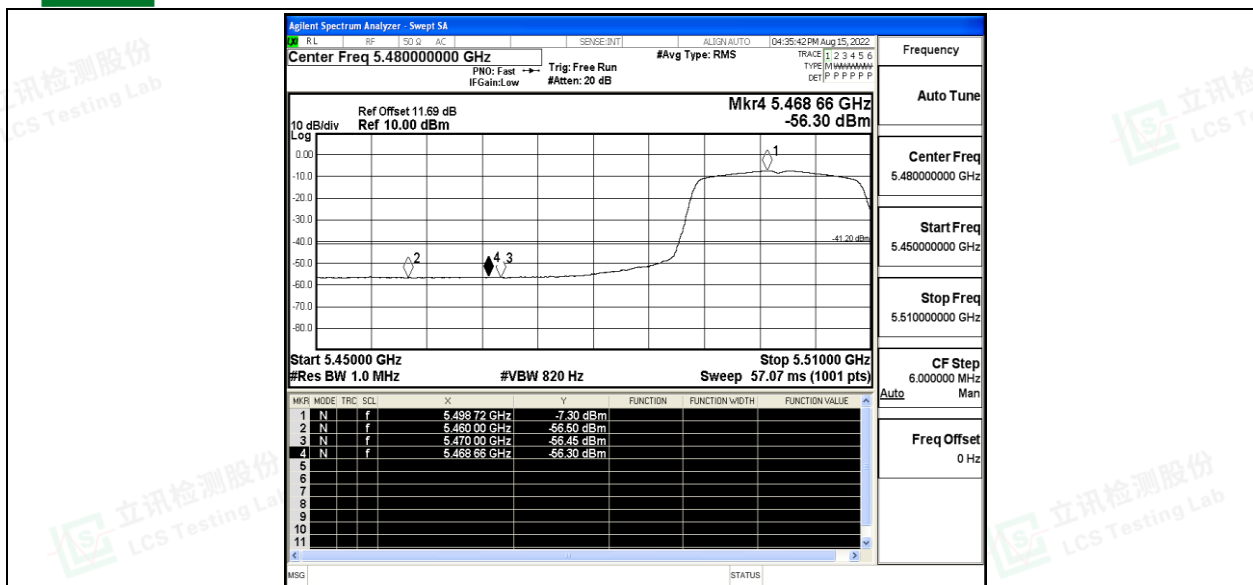
11AC20SISO_Ant0_Low_5500_Peak
