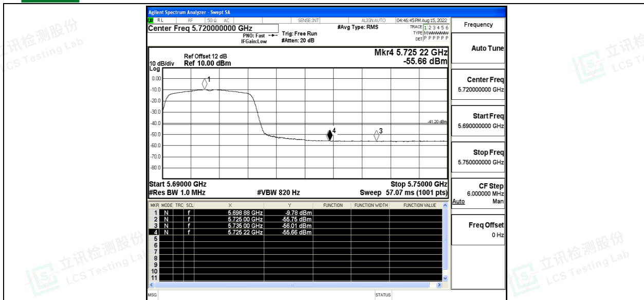
11AC20SISO_Ant1_High_5700_Peak
