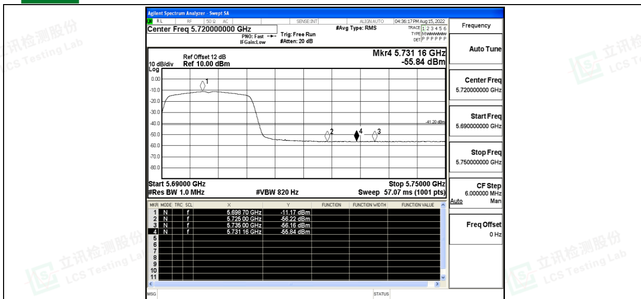
11AC20SISO_Ant0_High_5700_Peak
