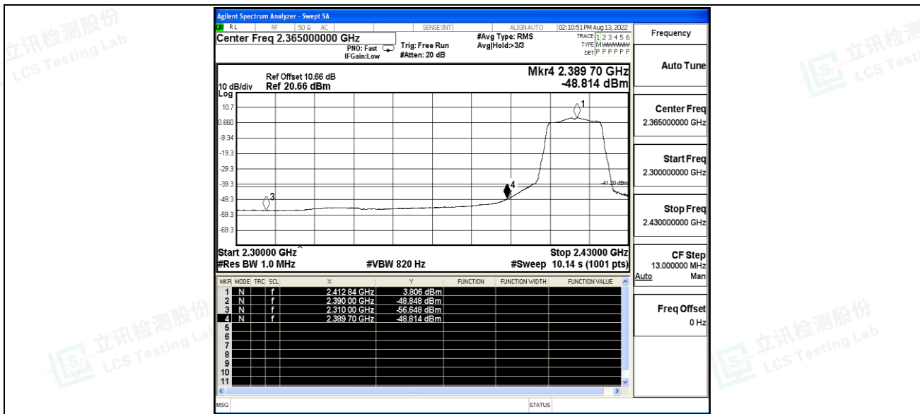
11N20SISO_Ant1_Low_2412_Peak
