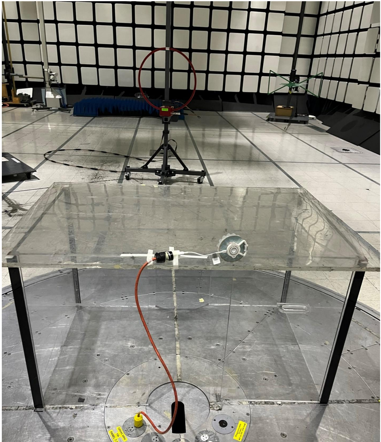
Radiated Emissions, Charging Operation
