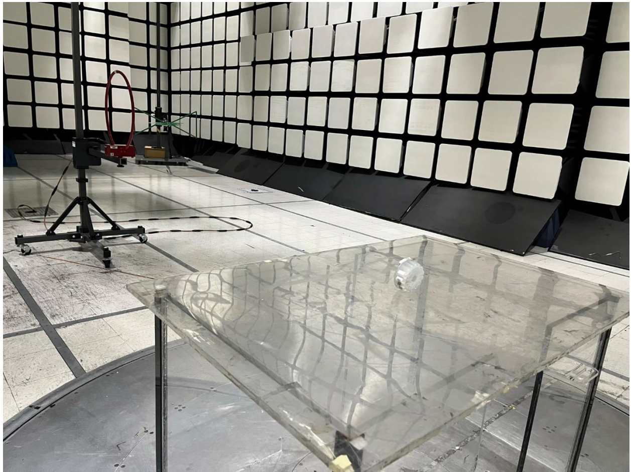
Radiated Emissions, Battery Powered Operation
