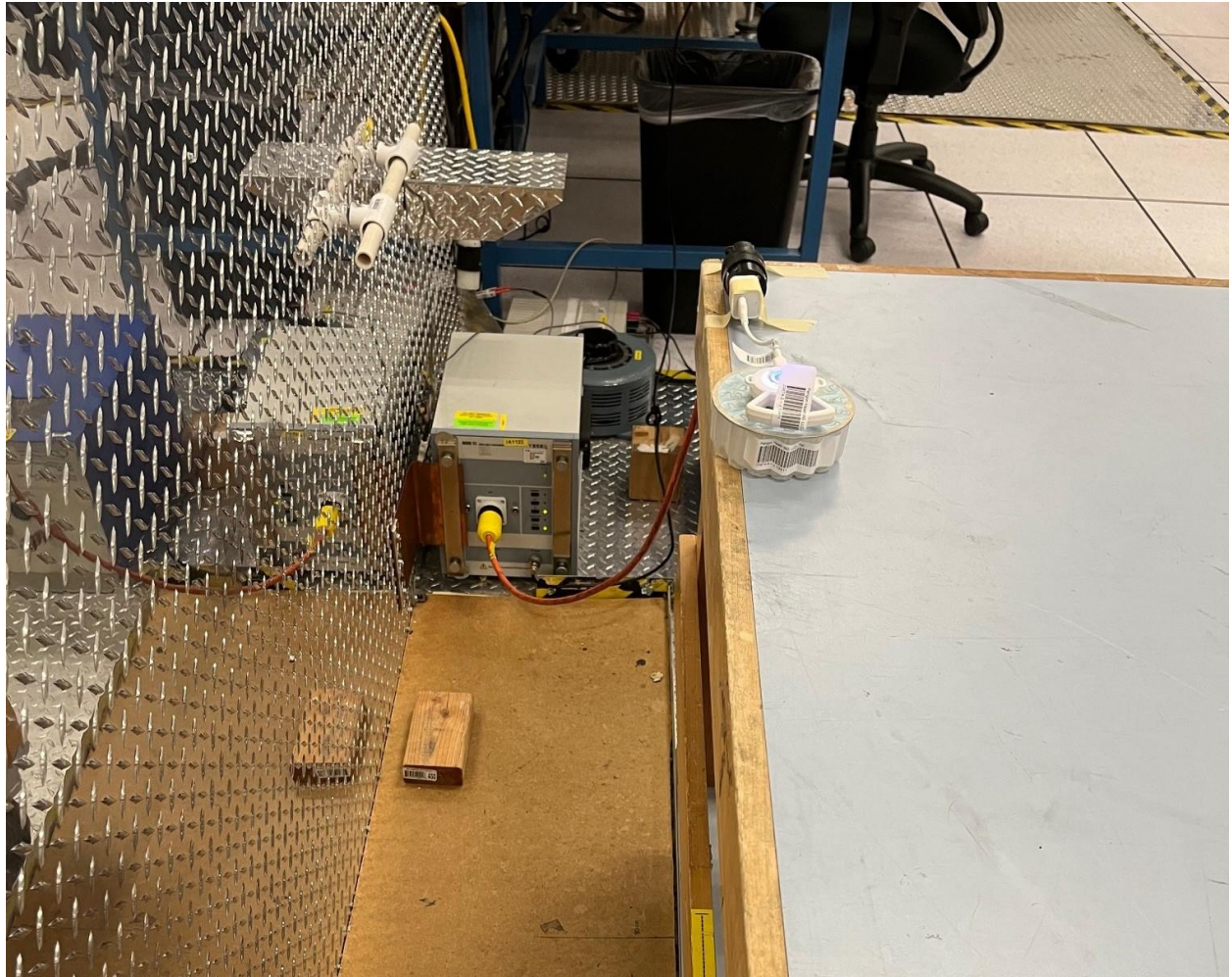
Conducted Emissions (Side)
