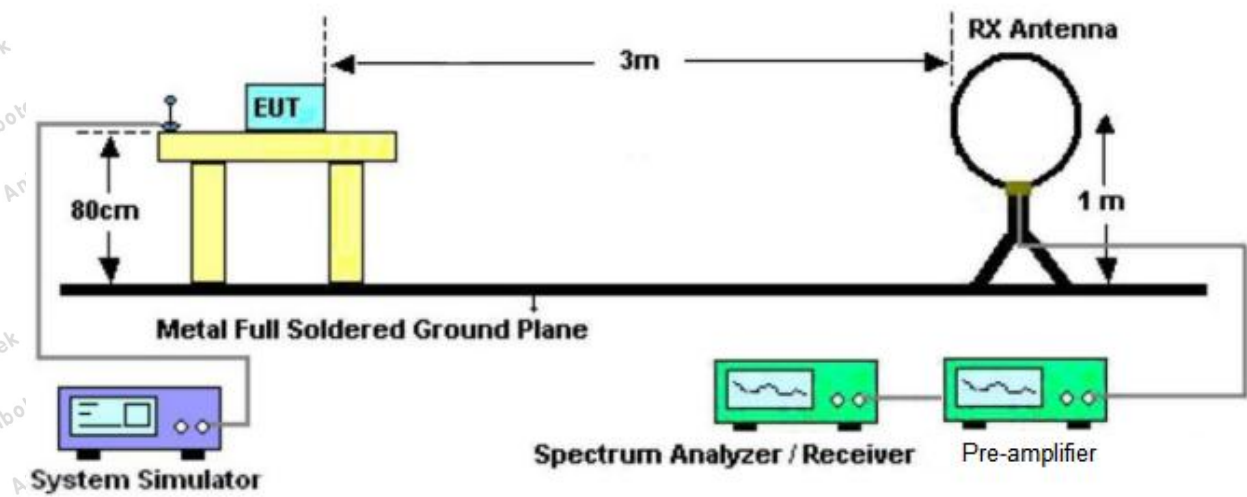
Figure 1. Below 30MHz
