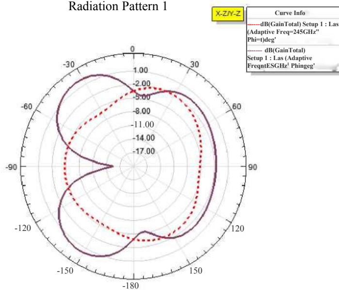
Radiation Pattern 1
