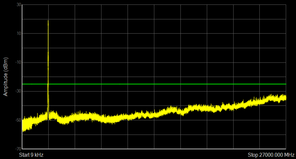
Band41 16QAM BW=20MHz Channel=41490 RB Size=100 Position=#0
