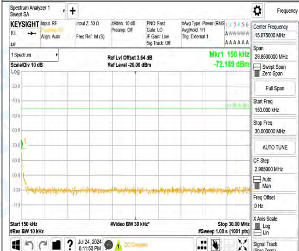
Band41_10MHz_16QAM_40290_1RB#0_1000-20000_1000-20000
