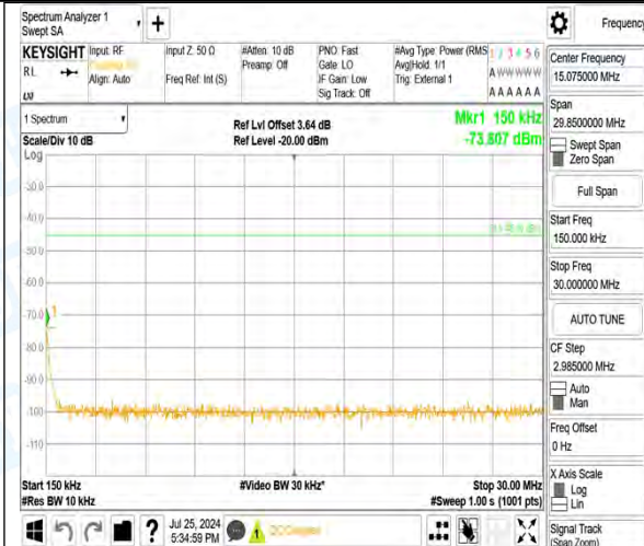
Band41_15MHz_QPSK_40690_1RB#0_1000-20000_1000-2000
