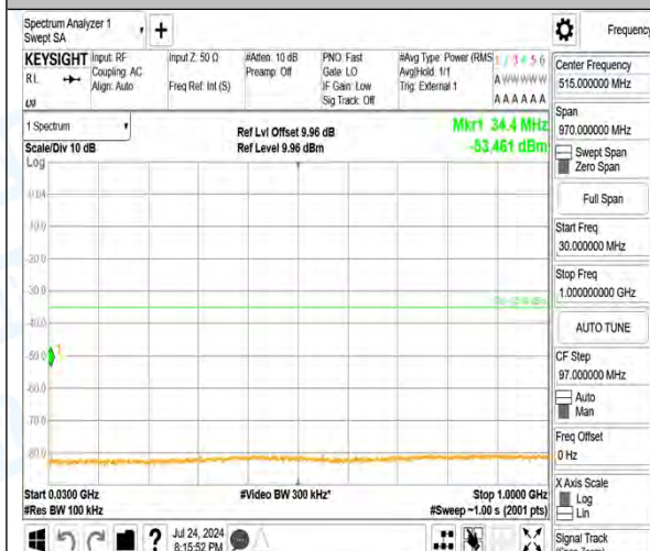
Band41_10MHz_16QAM_40690_1RB#0_20000~27000_20000~27000
