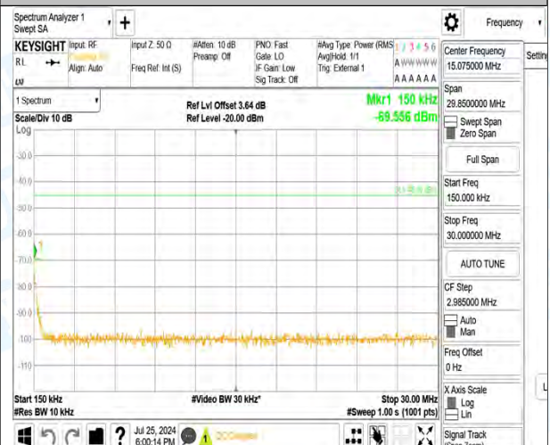
Band41_20MHz_QPSK_41140_1RB#0_1000-20000_1000-2000
