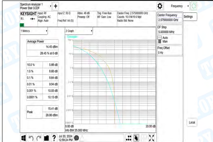
Band38-10MHz-16QAM-38000-1RB#0-PASS
