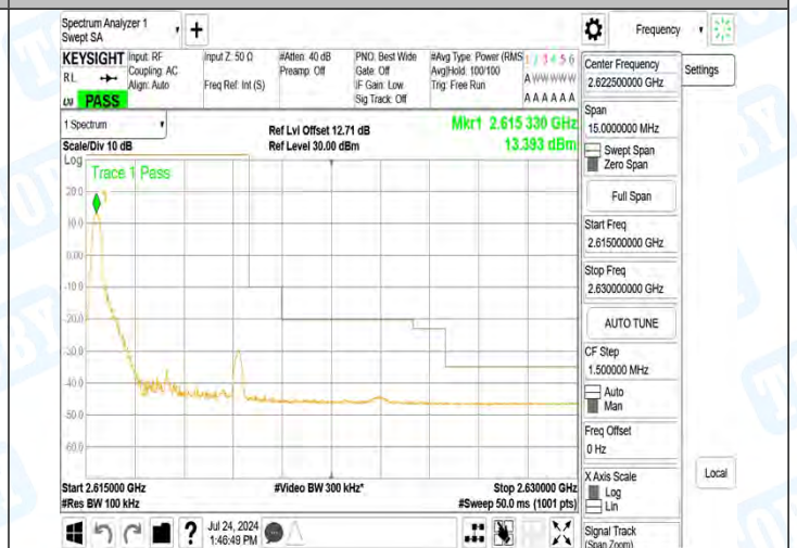
Band38_5MHz_16QAM_38225_25RB#0
