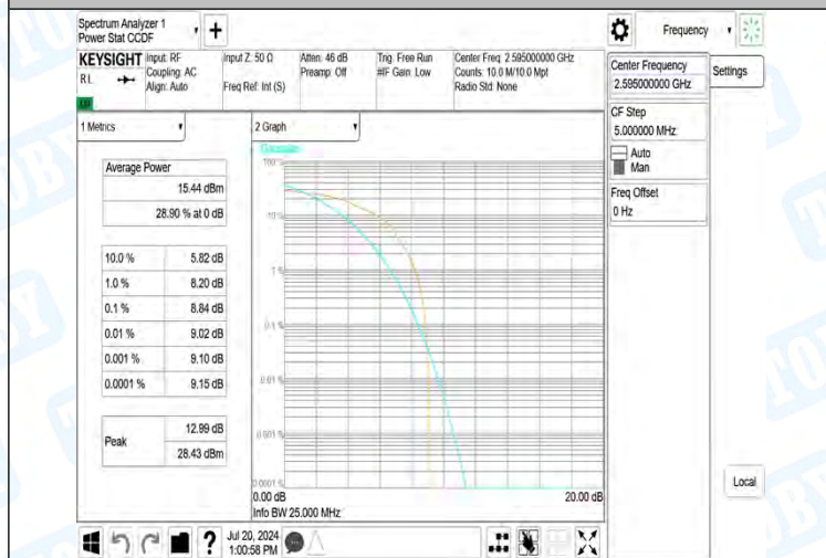
Band38-10MHz-16QAM-38200-1RB#0-PASS
