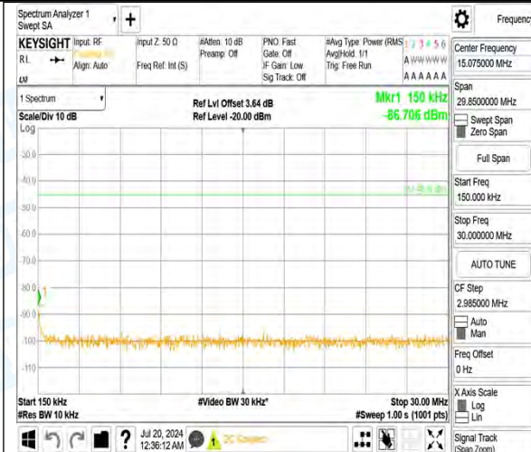
Band7_10MHz_QPSK_21100_1RB#0_1000~20000_1000~20000
