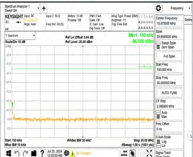
Band7_10MHz_QPSK_20800_1RB#0_1000-20000_1000-20000
