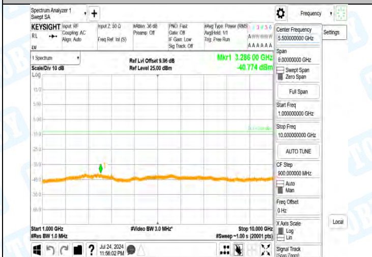
Band5-4233-4-1000~10000MHz-PASS
