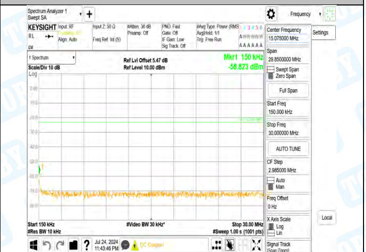
Band5-4233-3-0.15~30MHz-PASS
