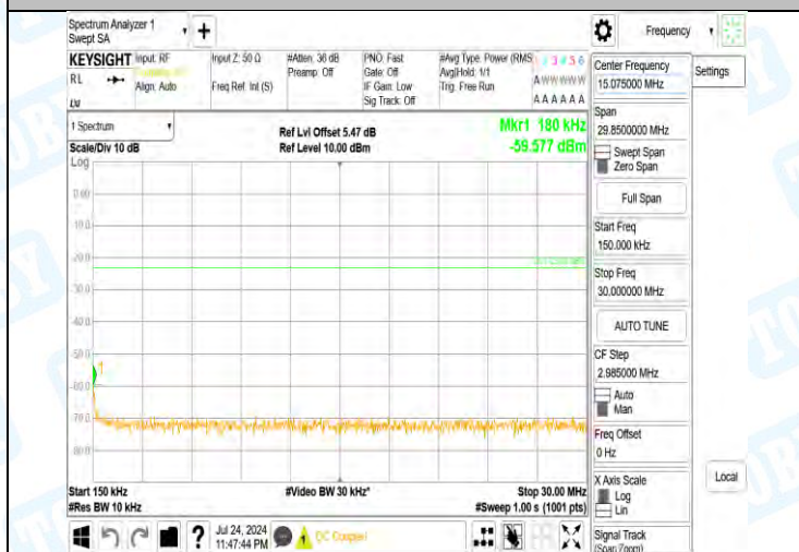
Band5-4233-4-0.15~30MHz-PASS
