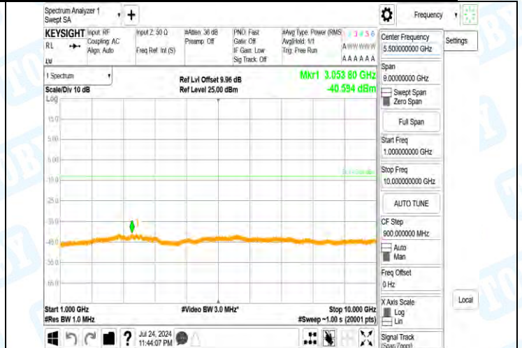
Band5-4233-3-1000~10000MHz-PASS
