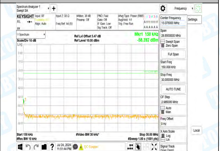
Band5-4233-5-0.15~30MHz-PASS
