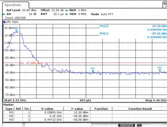
11A_Ant1_High_5240
