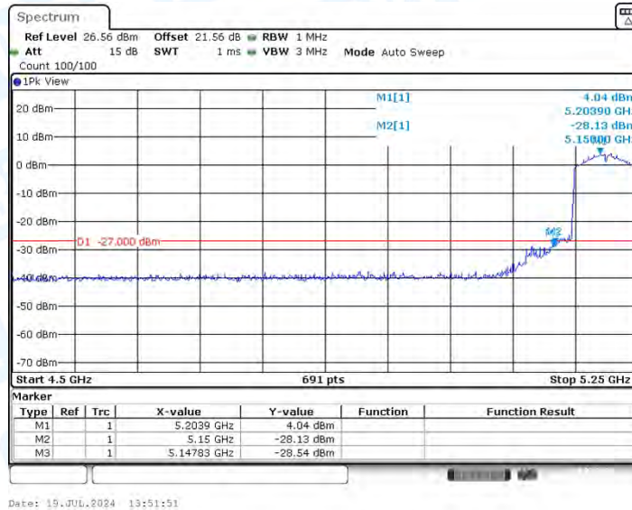
11AC80SISO_Ant1_High_5210
