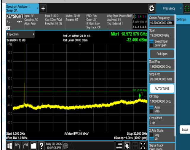
41(2555-2655)-15MHz-QPSK-40690-1RB#0-1000~20000-PASS
