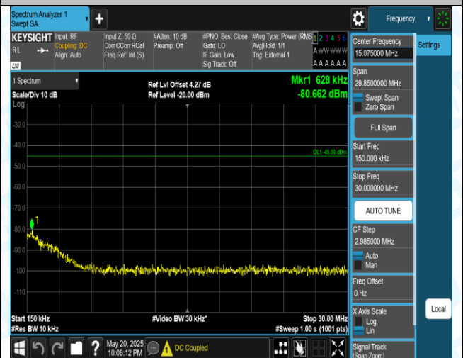
41(2555-2655)-15MHz-16QAM-40690-1RB#0-0.15~30-PASS
