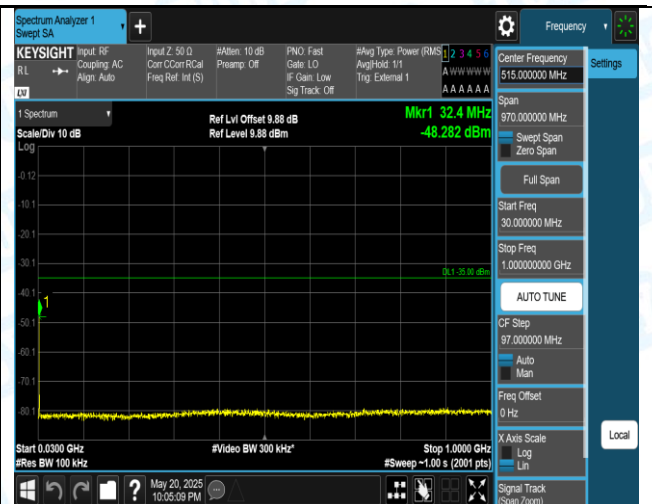
41(2555-2655)-15MHz-QPSK-40690-1RB#0-30~1000-PASS
