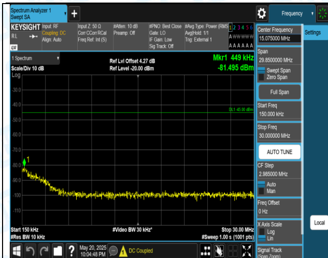
41(2555-2655)-15MHz-QPSK-40690-1RB#0-0.15~30-PASS
