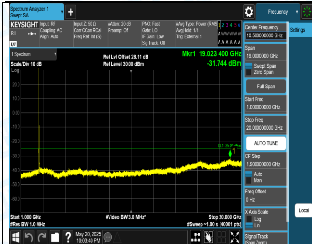
41(2555-2655)-15MHz-16QAM-40315-1RB#0-1000~20000-PASS
