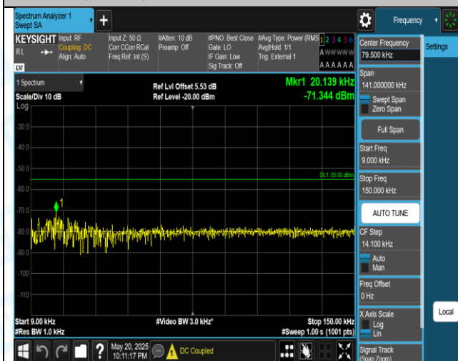
41(2555-2655)-15MHz-QPSK-41165-1RB#0-0.009~0.15-PASS
