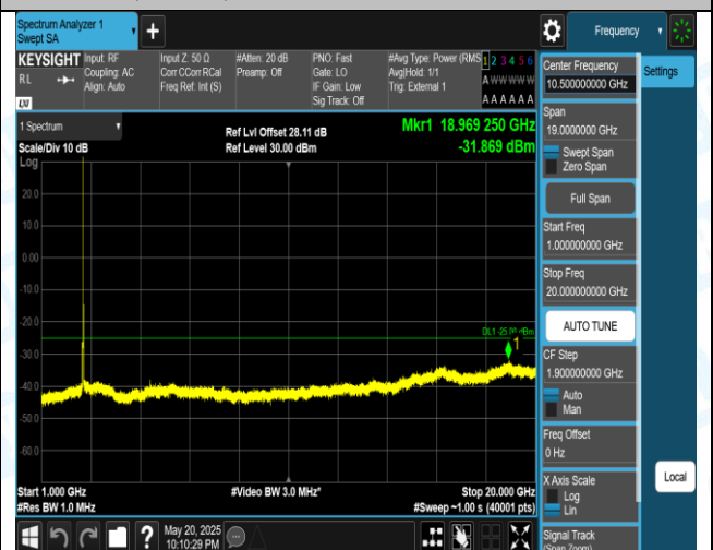
41(2555-2655)-15MHz-16QAM-40690-1RB#0-1000~20000-PASS
