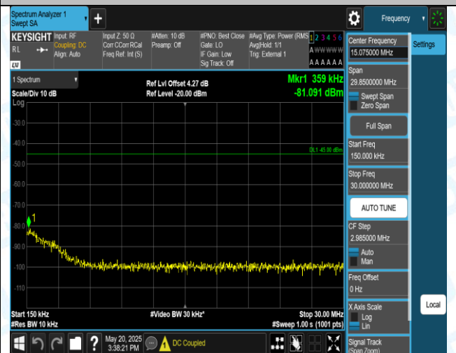
41(2555-2655)-5MHz-16QAM-40690-1RB#0-0.15-30-PASS
