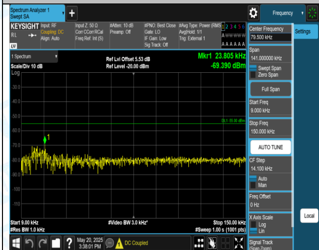
41(2555-2655)-5MHz-16QAM-40690-1RB#0-0.009-0.15-PASS
