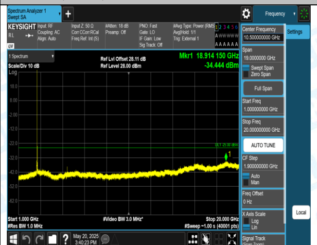
41(2555-2655)-5MHz-16QAM-40690-1RB#0-1000-20000-PASS
