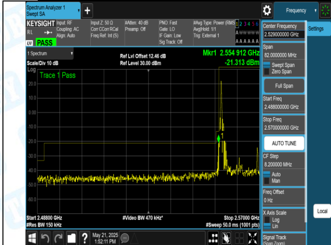
41(2555-2655)-15MHz-QPSK-40315-1RB#0-PASS
