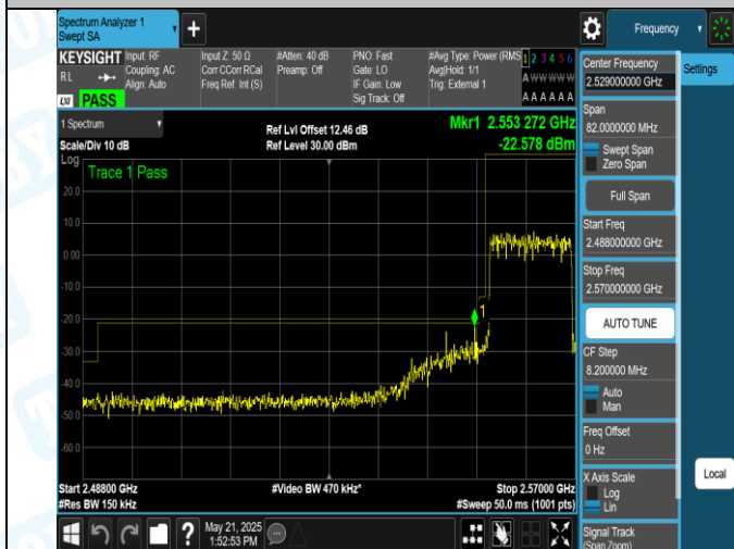
41(2555-2655)-15MHz-QPSK-40315-75RB#0-PASS
