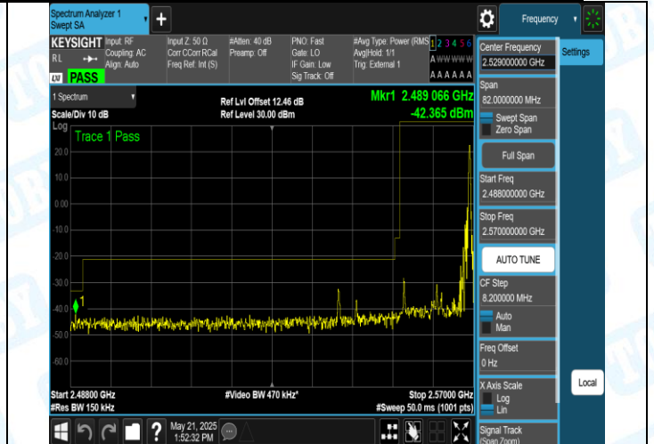
41(2555-2655)-15MHz-QPSK-40315-1RB#74-PASS
