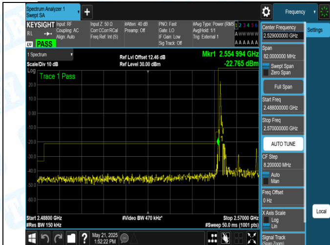
41(2555-2655)-15MHz-16QAM-40315-1RB#0-PASS
