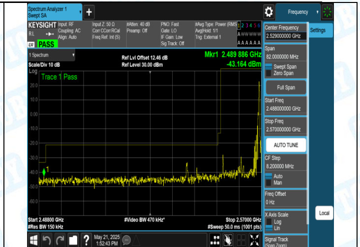
41(2555-2655)-15MHz-16QAM-40315-1RB#74-PASS
