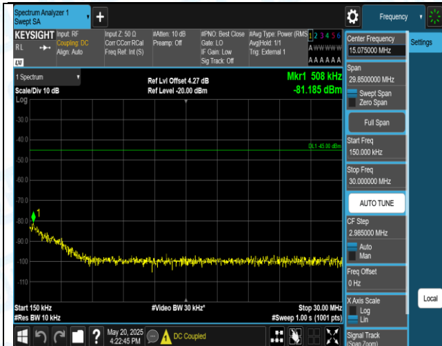
Band38-5MHz-QPSK-38000-1RB#0-0.15-30-PASS
