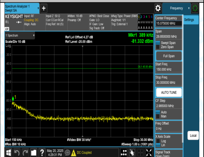
Band38-5MHz-QPSK-38225-1RB#0-0.15-30-PASS
