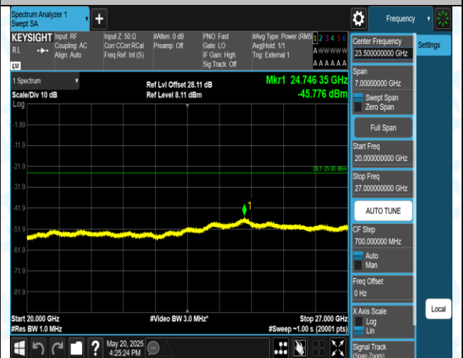
Band38-5MHz-QPSK-38000-1RB#0-20000-27000-PASS
