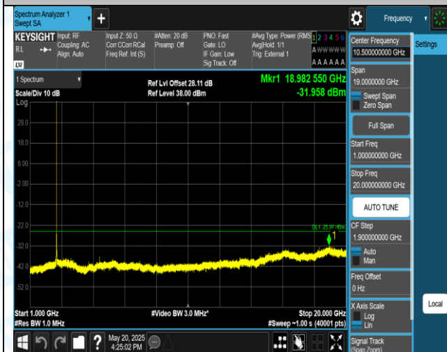
Band38-5MHz-QPSK-38000-1RB#0-1000-20000-PASS
