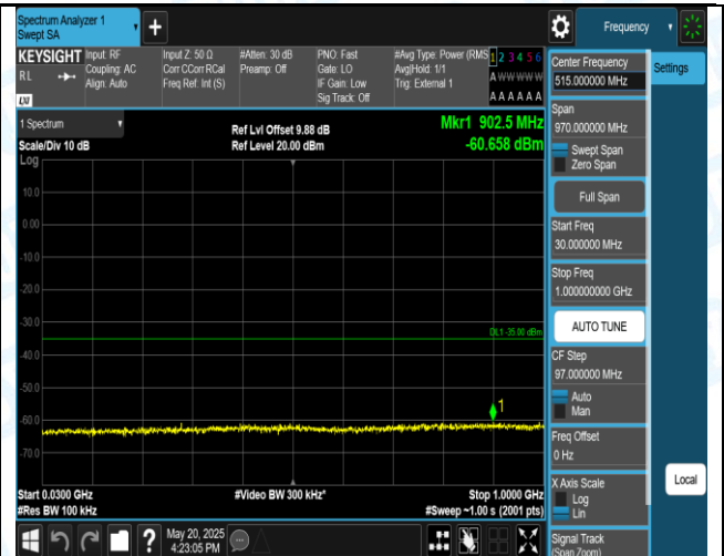
Band38-5MHz-QPSK-38000-1RB#0-30-1000-PASS
