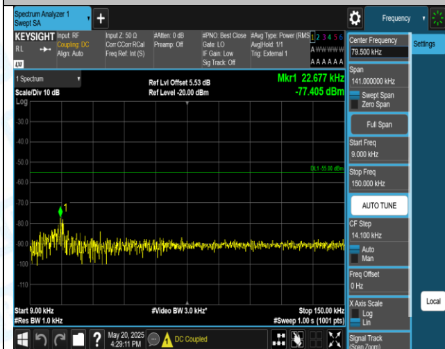
Band38-5MHz-QPSK-38225-1RB#0-0.009-0.15-PASS
